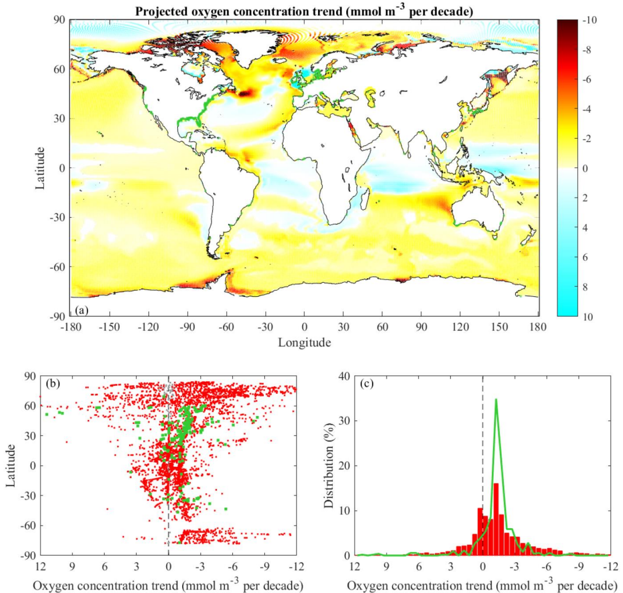
345 Figure 6: Projected vertical-minimum oxygen concentration trends: (a) spatial distribution for all CESM ocean grid cells, (b) latitudinal dependence for global coastal points and documented coastal hypoxic areas, and (c) histograms of global coastal points
