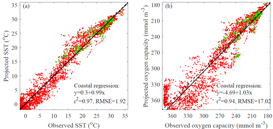
270 Figure 3: Comparison of projected to observed coastal conditions: (a) SST and (b) surface oxygen capacity. Mean values for the overlapping 2006-2021 period are compared. Global coastal points and documented coastal hypoxic areas are marked in red and green, respectively. The one-to-one line (dashed) and linear regression (solid) are included along with associated regression statistics ( p < 0.001 for both regressions).
