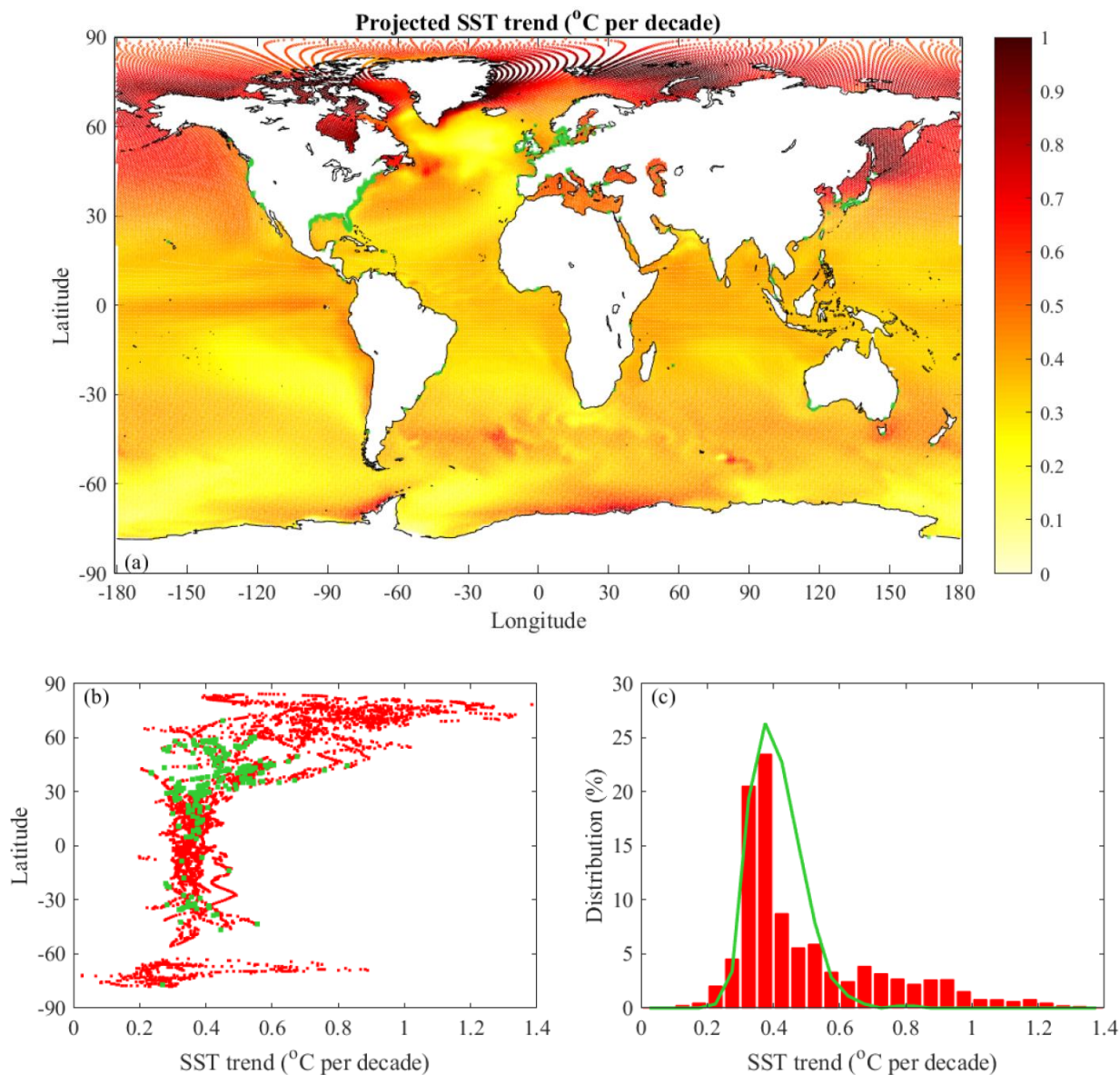
Figure 4: Projected SST trends: (a) spatial distribution for all CESM ocean grid cells, (b) latitudinal dependence for global coastal points and documented coastal hypoxic areas, and (c) histograms of global coastal points and documented coastal hypoxic areas. The format and color coding follow Fig. 1.
