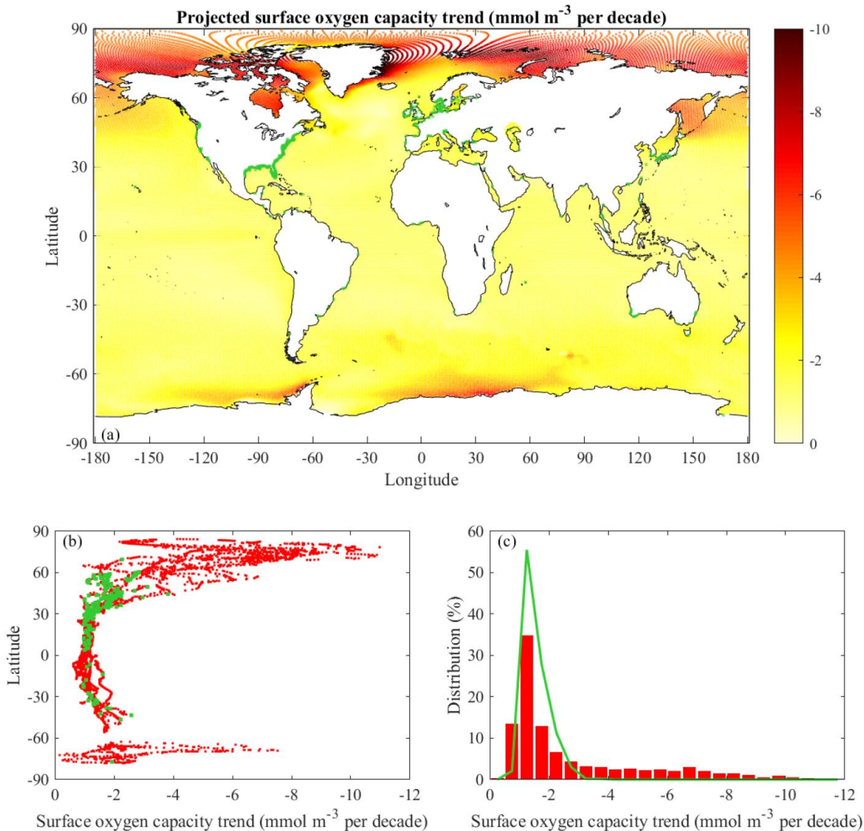
335 Figure 5: Projected surface oxygen capacity (saturation concentration) trends: (a) spatial distribution for all CESM ocean grid cells, (b) latitudinal dependence for global coastal points and documented coastal hypoxic areas, and (c) histograms of global coastal points and documented coastal hypoxic areas. The format and color coding follow Fig. 1.
