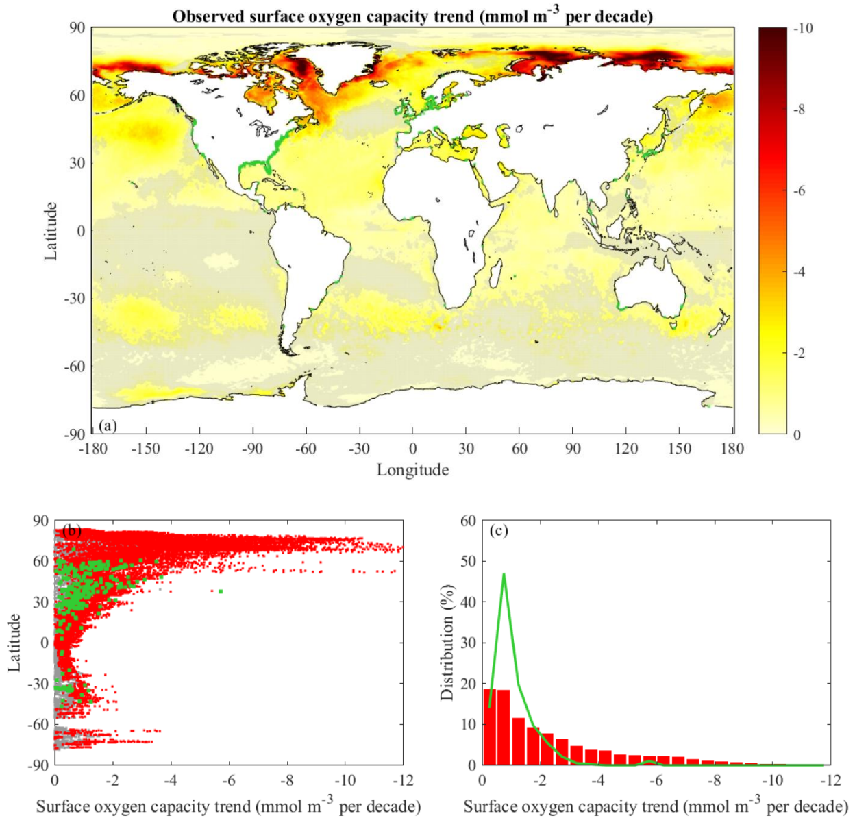
260 Figure 2: Observed surface oxygen capacity (saturation concentration) trends: (a) spatial distribution for all ocean observational points, (b) latitudinal dependence for global coastal points and documented coastal hypoxic areas, and (c) histograms of global coastal points and documented coastal hypoxic areas. The format and color coding follow Fig. 1.
