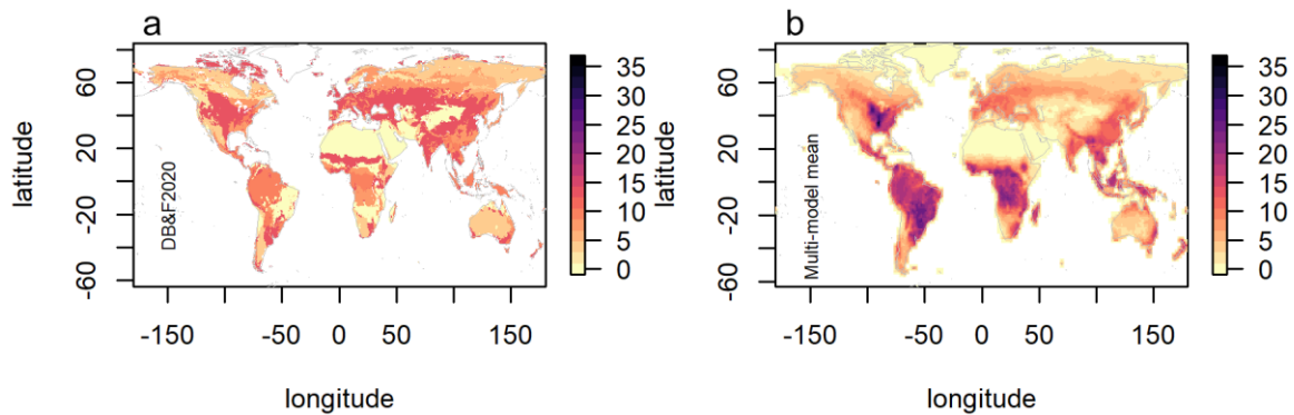
520 Figure 2: Map of observation-biome-based estimates of BNF in \text{kg N ha}^{-1} \text{yr}^{-1} (a) and a map of multi-model mean BNF for the period 1980 – 2015 (b).
