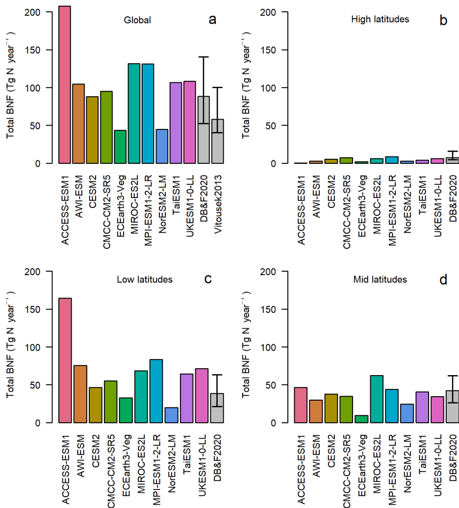
515 Figure 1: The global total annual BNF (TgN yr -1 ) for the average of the period 1980 – 2014. The grey bars areas represent the observationally-constrained ranges by Davies-Barnard and Friedlingstein, (2020) and (Vitousek et al., 2013). The four panels represent latitude bands and global. High latitudes: more than 60°N or 60°S. Mid latitudes: less than 60°N and more than 30°N less than 60°S and more than 30°S. Low latitudes: less than 30°N and less than 30°S.
