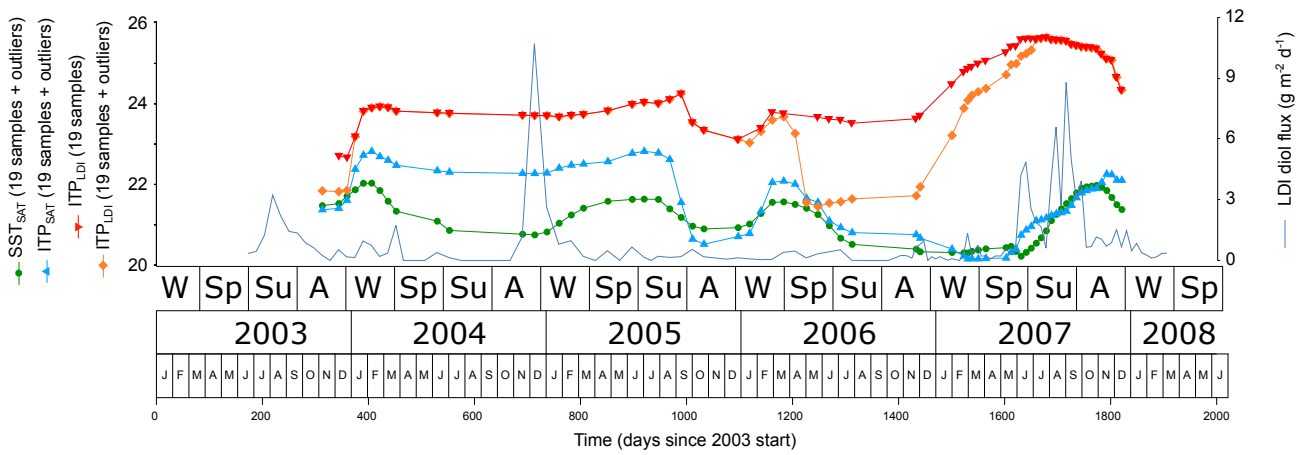
Figure RC1-1. Nineteen sample moving average SST SAT (green spheres) and nineteen sample moving integrated production temperatures for SST SAT (IPT SAT , blue upward triangles) and for SST LDI (IPT LDI , orange diamonds), both based on the LDI diol fluxes and the respective SST records. Samples with LDI outliers (values < 17°C) are included except for the upper graph of IPT LDI (red downward pointing triangles). For reference, the LDI dot flux is included as well.
