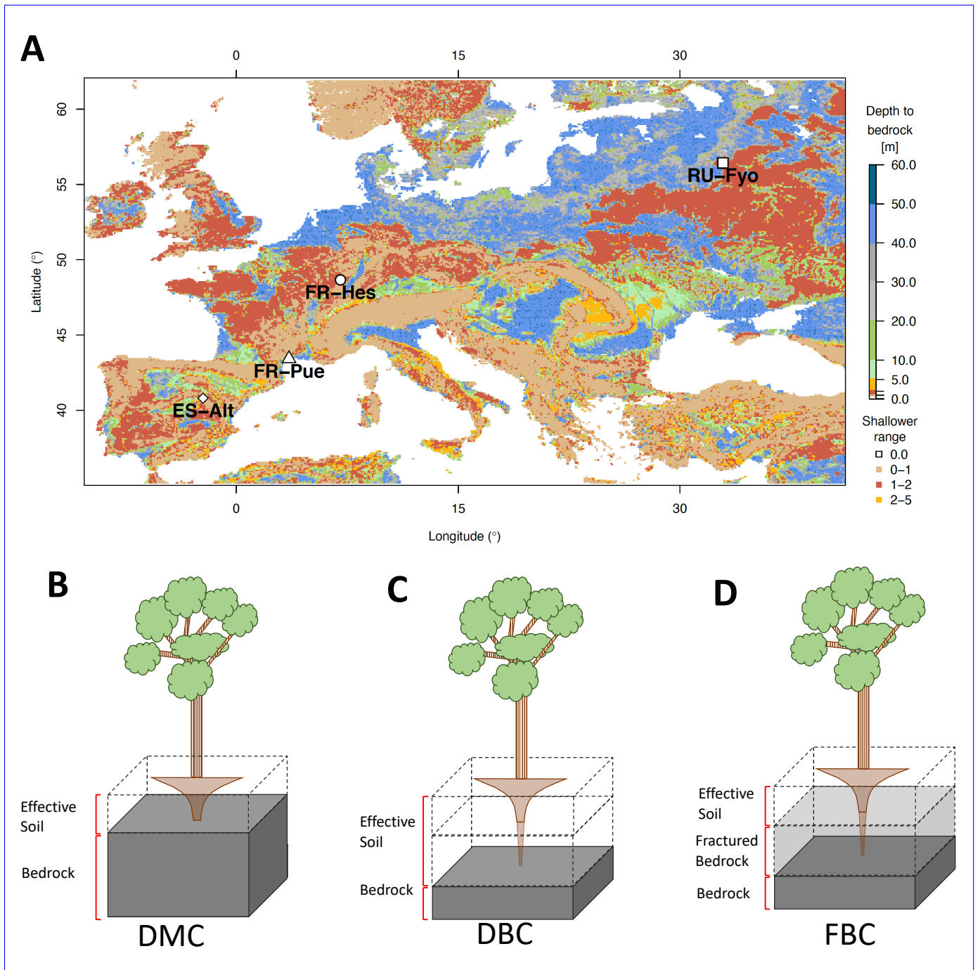
Figure 1. Geographical location of the experimental sites and spatial distribution of the depth to bedrock across Europe (A) based on Pelletier et al. (2016) . Schematic —The graphics below the map are the schematic of the three bedrock representations model configurations used in this work: default model configuration, DMC (B); deeper bedrock configuration, DBC (C); and fractured bedrock configuration, FBC (D). The block with dashed lines represents the soil profile, the solid grey block represents the impermeable bedrock layer as it is assumed by CLM 5, and the translucent grey block represents the mimicked fractured bedrock layer.
