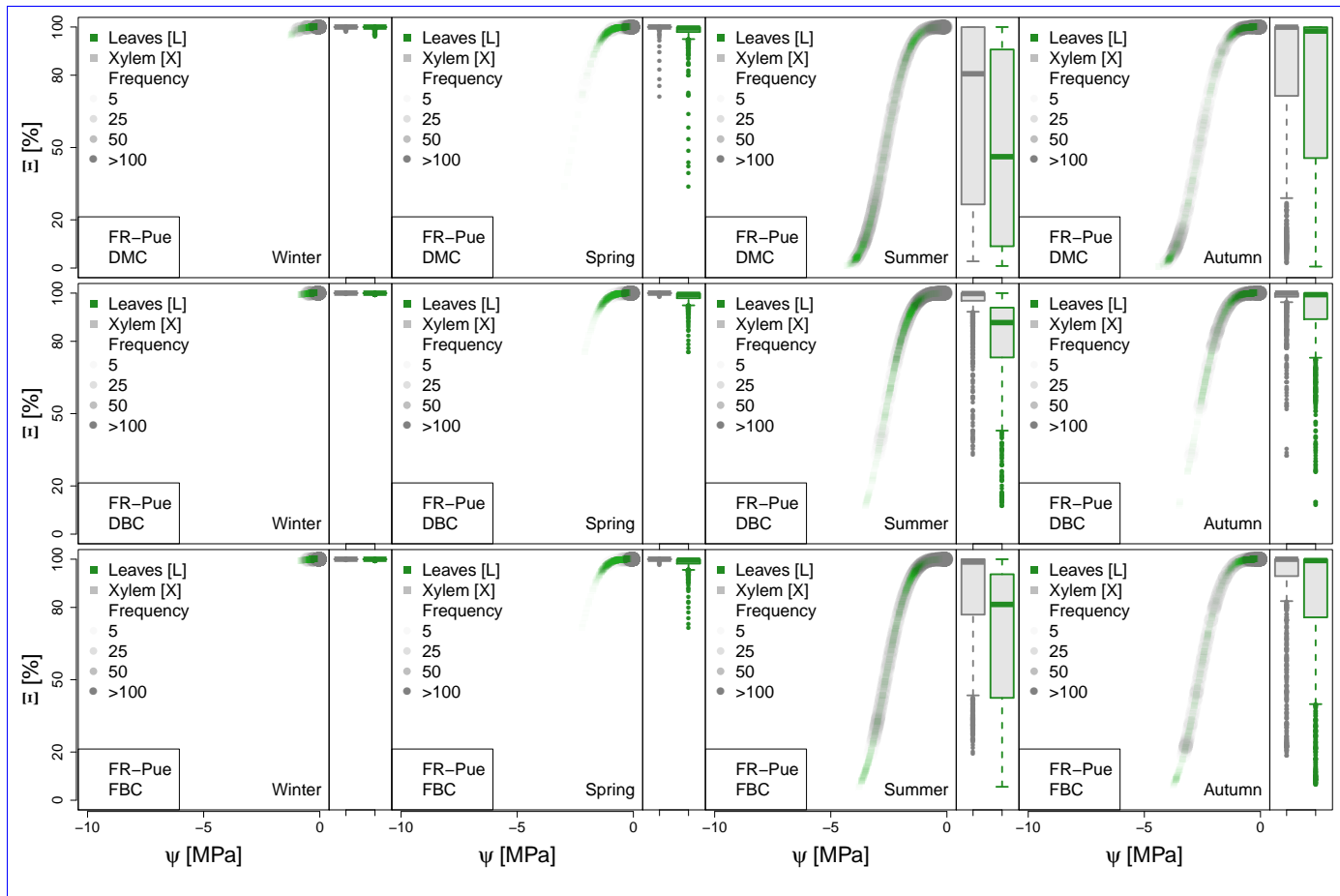
Figure A4. Seasonal variation of the plant vulnerability curves describing the hydraulic stress as percentage of conductivity ( \Xi ) experienced by the modeled vegetation in FR-Pue experimental site. Each plot describes the hydraulic stress experienced by stem xylem (X) and sunny leaves xylem (L).
