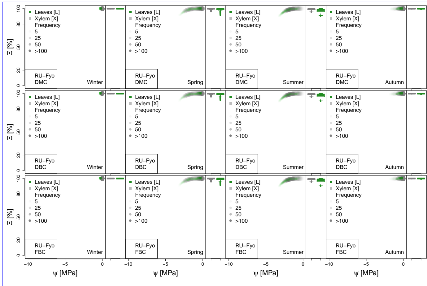
Figure A6. Seasonal variation of the plant vulnerability curves describing the hydraulic stress as percentage of conductivity ( \Xi ) experienced by the modeled vegetation in RU-Fyo experimental site. Each plot describes the hydraulic stress experienced by stem xylem (X) and sunny leaves xylem (L).
