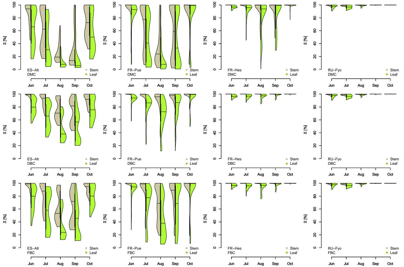
Figure 5. Plant vulnerability curves describing the hydraulic stress as percentage of conductivity ( \Xi ) experienced by the modeled vegetation per experimental site during based on the drier months vulnerability curves of each plant organ (July, August, and September See Fig. A1 to Fig. A6) between June and October. Each plot describes the distribution of the hydraulic stress experienced by stem xylem (X) and sunny leaves xylem (L) expressed as percentage of conductivity ( \Xi ).
