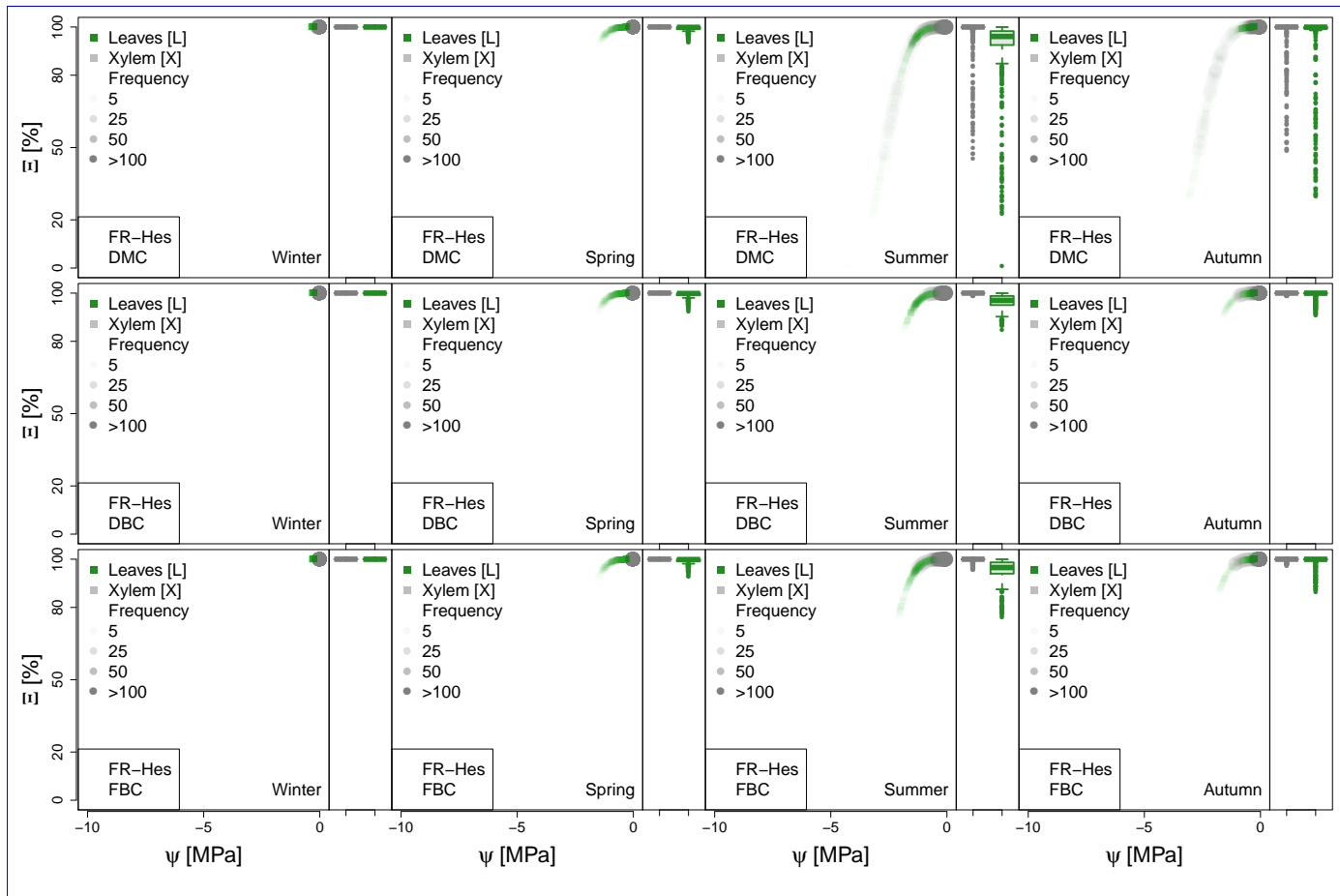
Figure A5. Seasonal variation of the plant vulnerability curves describing the hydraulic stress as percentage of conductivity ( \Xi ) experienced by the modeled vegetation in FR-Hes experimental site. Each plot describes the hydraulic stress experienced by stem xylem (X) and sunny leaves xylem (L).
