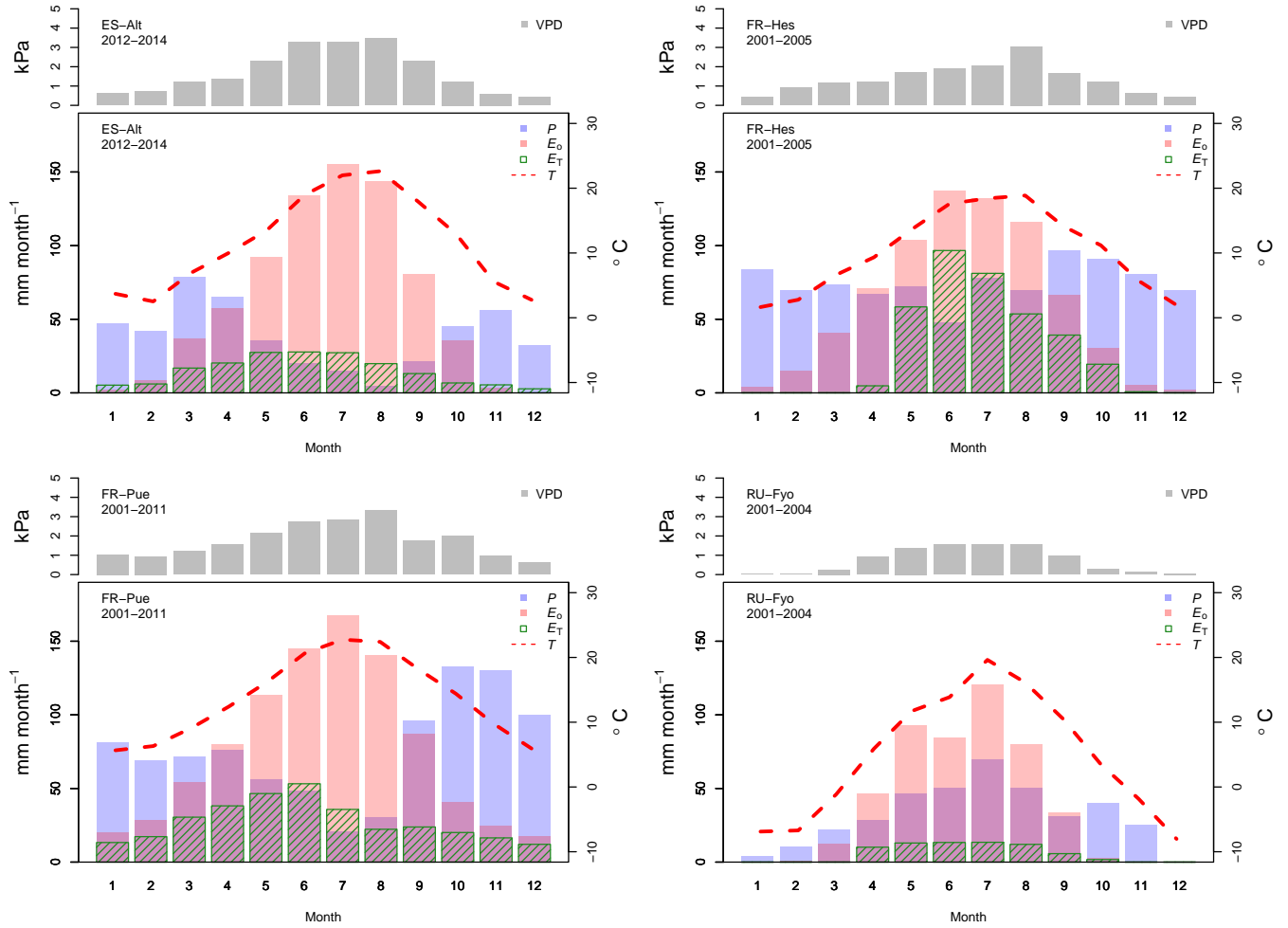
Figure 2. Monthly temporal variation of the maximum vapor pressure deficit (VPD), total precipitation ( P ), total potential evaporation ( E_o ), measured total transpiration ( E_T ), and mean air temperature ( T ) for the selected experimental sites across Europe. Monthly averages. The monthly values are based on the different sampling periods for each site.
