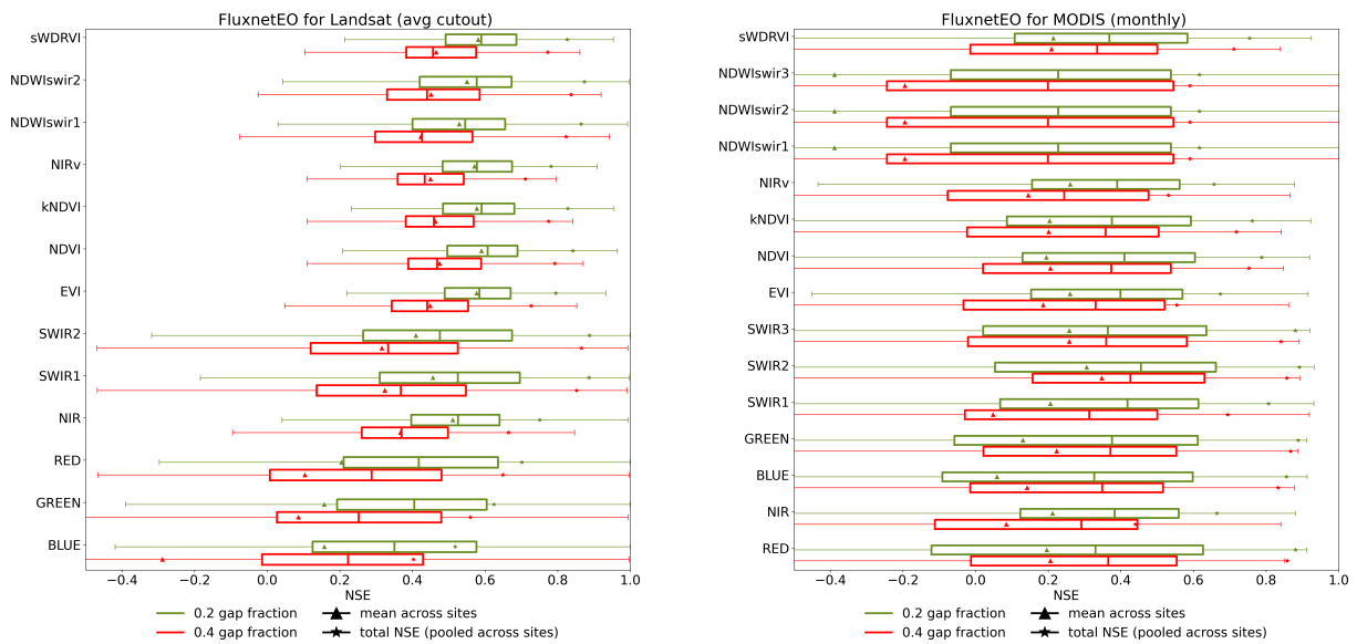
Figure C2. Benchmarking in artificial gaps: distribution of NSE per site of the gap-fill estimates in artificial gaps by FluxnetEO. 20% and 40% of data were removed and gapfilled. Left: Landsat time series of the average reflectance/ vegetation index across the whole cutout. Right: the centre pixel of MODIS data aggregated to monthly temporal resolution.
