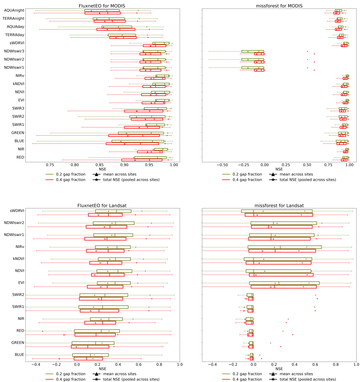
Figure C1. Benchmarking in artificial gaps: distribution of NSE per site of the gap-fill estimates in artificial gaps by FluxnetEO (left) and missForest (right) within the physical ranges of the indices for 20% and 40% of good quality data removed. For MODIS (top) and Landsat (bottom), random good quality samples are removed from the tower pixel. Note the different x-axis limits.
