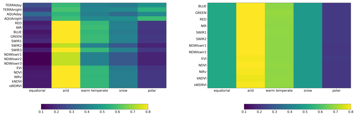
Figure 1. Fraction of good quality data in the MODIS (left) and Landsat (right) time series. Colours represent the median data availability in tower pixels across sites grouped by Koeppen climate classification. Data refer to the period 2003–2020 for MODIS (the time period when both TERRA and AQUA satellites are in space) and 1990–2017 for Landsat.
