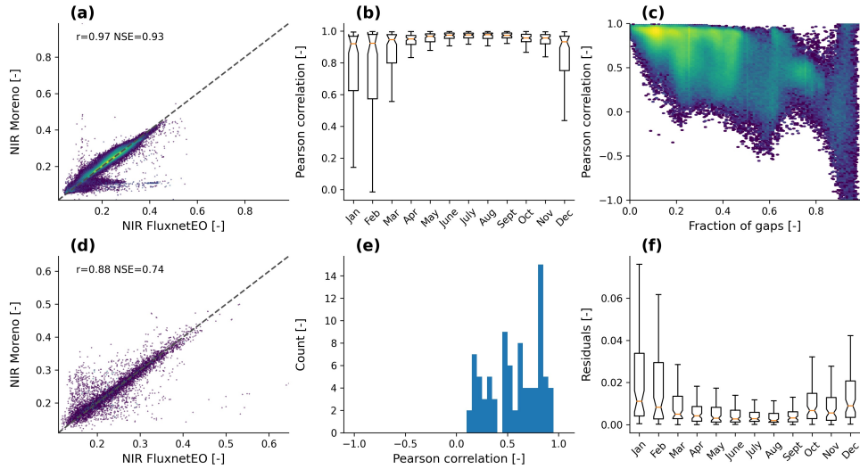
Figure 8. Benchmarking Landsat NIR reflectance from FluxnetEO against the product produced by Moreno-Martínez et al. (2020) at EC sites in the CONUS. Each NIR s,t,p value refers to one site (s), time step (t) and subpixel (p). Comparing spatial patterns: (a) scatterplot of the temporally averaged NIR reflectance (mean t (NIR s,p,t ), each dot reflects one subpixel and site). (b) Temporal average across years for each month separately and the spatial Pearson correlation across all subpixels in a cutout per site and month cor_p(\text{mean}_t\text{-month}(\text{NIR FluxnetEO}_{s,p,t}), \text{mean}_t\text{-month}(\text{NIR Moreno et al}_{s,p,t})) . (c) Temporal correlation in dependence of the amount of missing values in the FluxnetEO product in each subpixel and site ( cor_t(\text{NIR FluxnetEO}_{s,t,p}, \text{NIR Moreno}_{s,t,p}) ). (d-f): Compute a spatial average across all subpixels in a cutout per time step: \text{NIR}^*_{s,t} = \text{mean}_p(\text{NIR}_{s,t,p}) . (d) Temporal Pearson correlation of the spatially averaged NIR ( cor_t(\text{NIR FluxnetEO}^*_{s,t}, \text{NIR Moreno}^*_{s,t}) ). (e) Pearson correlation of the deviations from the mean seasonal cycle of the spatially averaged time series. (f) Difference between FluxnetEO and Moreno NIR reflectance and their average per month of the year \text{mean}_t\text{-month}(\text{NIR FluxnetEO}^*_{s,t} - \text{NIR Moreno}^*_{s,t}) . r refers to the Pearson correlation coefficient, NSE to the Nash-Sutcliffe efficiency (Nash and Sutcliffe, 1970).
