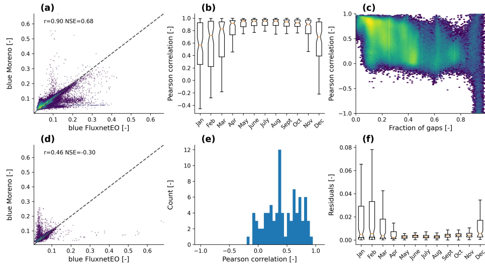
Figure C3. Benchmarking Landsat reflectance in the blue spectral band from FluxnetEO against the product produced by Moreno-Martínez et al. (2020) at EC sites in the CONUS. Each reflectance s,t,p value refers to one site (s), time step (t) and subpixel (p). Comparing spatial patterns: (a) scatterplot of the temporally averaged reflectance (mean(reflectance s,p ) t , each dot reflects one subpixel and site). (b) Spatial Pearson correlation across all subpixels in a cutout per site of the average grouped by month. (c) Temporal correlation in dependence of the amount of missing values in each subpixel and site. (d-f): Compute a spatial average across all subpixels in a cutout per time step. (d) Temporal Pearson correlation of the spatial average. (e) Pearson correlation of the deviations from the mean seasonal cycle of the spatially averaged time series. (f) Difference between FluxnetEO and Moreno reflectance and their average per month of the year. r refers to the Pearson correlation coefficient, nef to the Nash-Sutcliffe efficiency (Nash and Sutcliffe, 1970).
