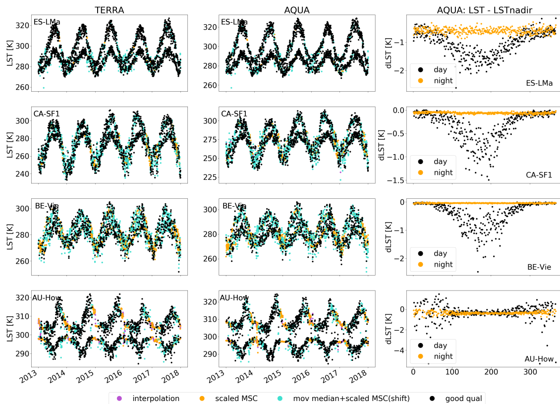
Figure 6. MODIS LST gap-filling steps in the 1km pixel containing selected eddy-covariance sites for daytime and nighttime LST. The rightmost column shows the average annual cycle of the correction factor between LST from variable viewing angles and LST corrected to nadir view.
