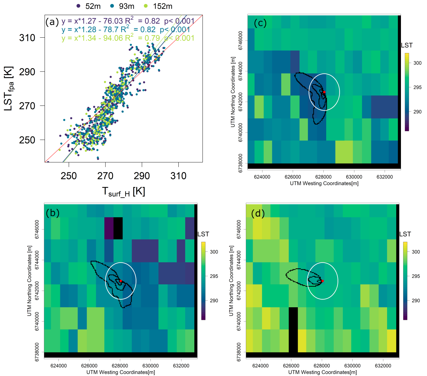
Figure 10. Relationship between MODIS AQUA day LST fpa and surface temperature ( T_{\text{surf}_H} ) calculated from the inverted sensible heat flux (details about the methods in Appendix D). The red line represents the 1:1 line. Subplots b to d show example footprints at the three levels (black lines) overlaid on the LST map from May 31st to June 2nd, 2017, respectively. Non-original low quality LST values are blacked out. The white circle indicates the 1 km diameter around the tower.
