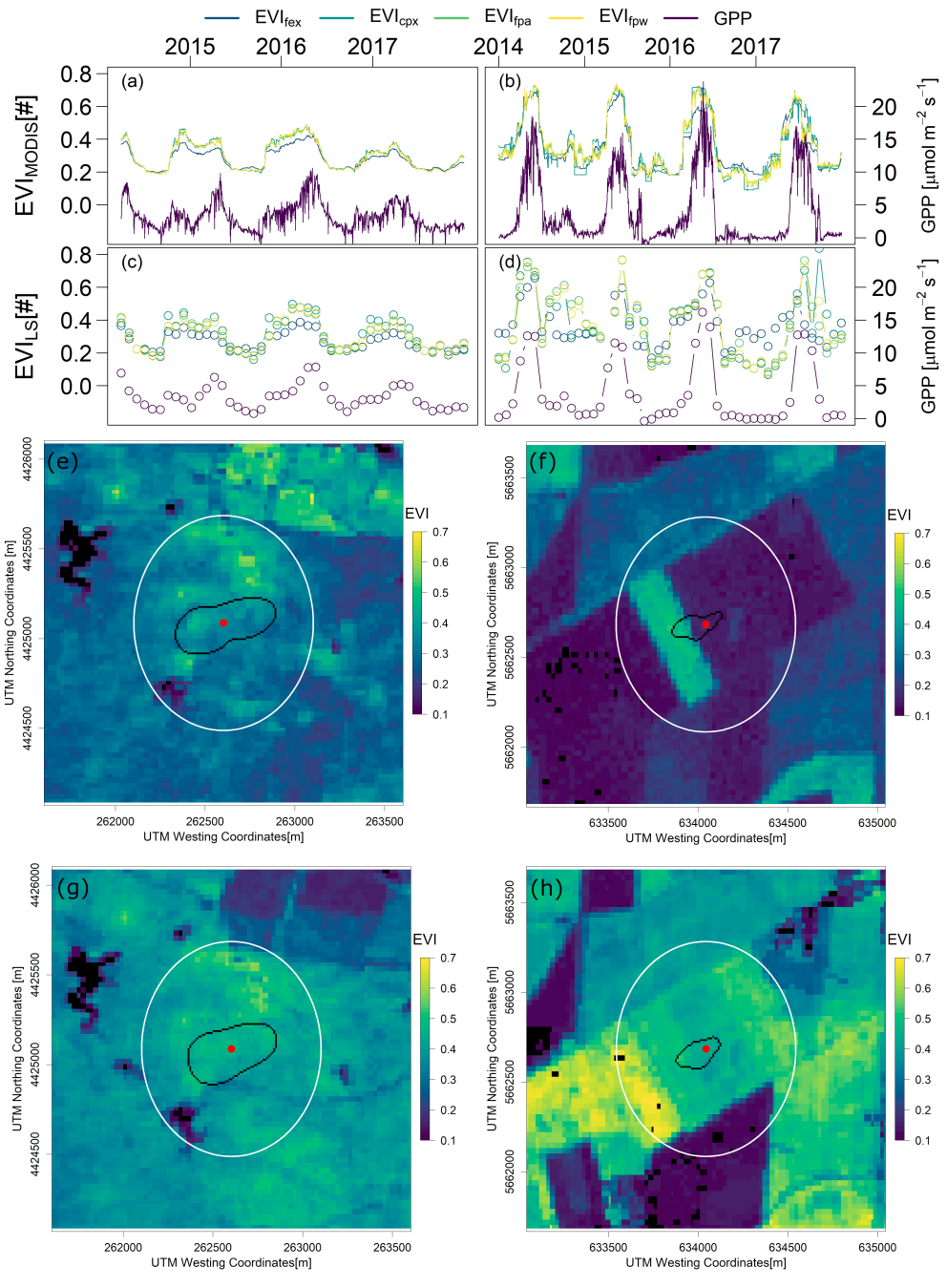
Figure 9. Time series of EVI and GPP for ES-LM1 (a,c) and DE-Geb (b,d). MODIS EVI (top row) and Landsat EVI (second row) represent areas with different extents: full extent of the cutout ( EVI_{fex} ), the center pixel that contains a tower ( EVI_{cpx} ), the EVI averaged over the flux footprint area ( EVI_{fpa} ), and the EVI_{fpa} weighted with the flux probability density function ( EVI_{fpw} ). Subplots e-h: Landsat EVI overlaid with the monthly flux footprint (black line) for ES-LM1 in November 2014 (e) and April 2016 (g), and for DE-Geb in February 2012 (f) and February 2016 (h). Non-original low quality EVI values are blacked out. Red circles indicate the location of the EC station, white circle denotes 1 km diameter from the station.
