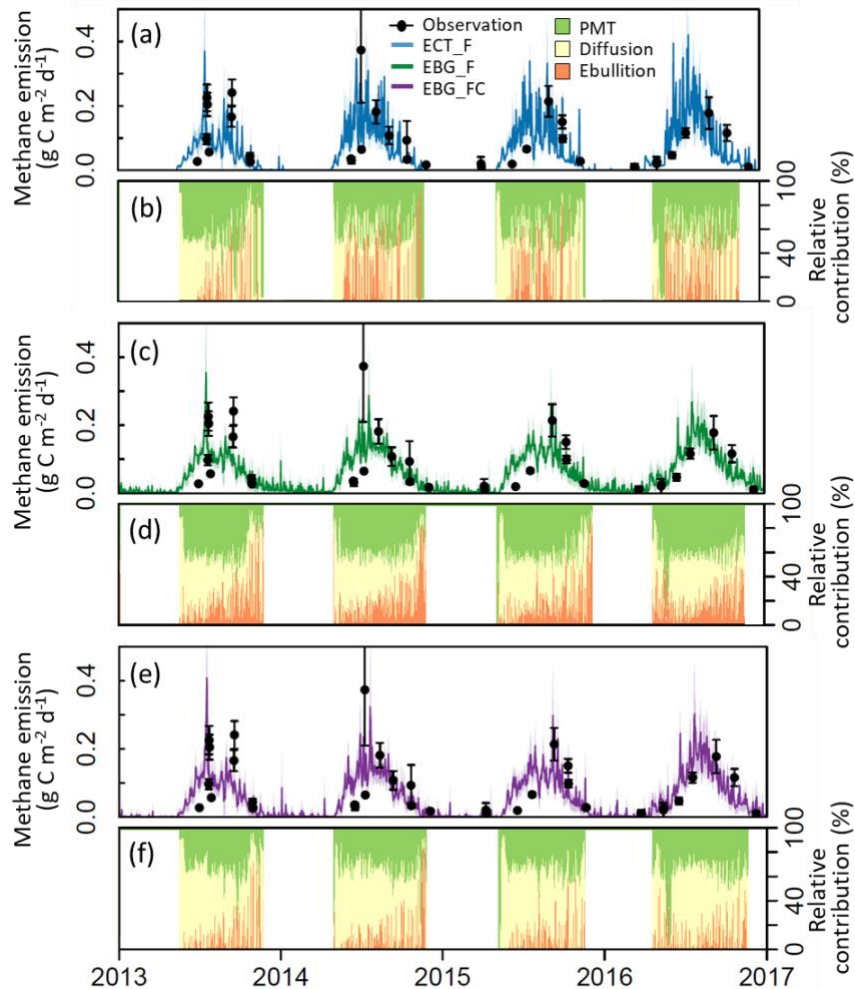
375 Figure 3. Observed versus modeled methane emissions (a, c, e) and simulated relative contributions (%) of plant- mediated transportation (PMT), diffusion, and ebullition under ambient conditions (b, d, f). Black dots are observed CH 4 emissions from static chamber measurements. Error bars are the standard errors. Blue lines are ECT model simulated CH 4 emissions based on the parameter probability distributions (PPDs) constrained by CH 4 flux data (ECT_F, RMSE = 0.61). Green lines are EBG model simulated CH 4 emissions based on the PPDs constrained by 380 CH 4 flux data (EBG_F, RMSE = 0.53). Purple lines are EBG model simulated emissions based on the PPDs constrained by both CH 4 flux and concentration data (EBG_FC, RMSE = 0.52). The midlines and shaded areas correspond to the means and standard deviations, respectively from 500 model simulations with parameters randomly drawn from the posterior distributions. Relative contributions (%) are the daily mean values calculated from the simulations.
