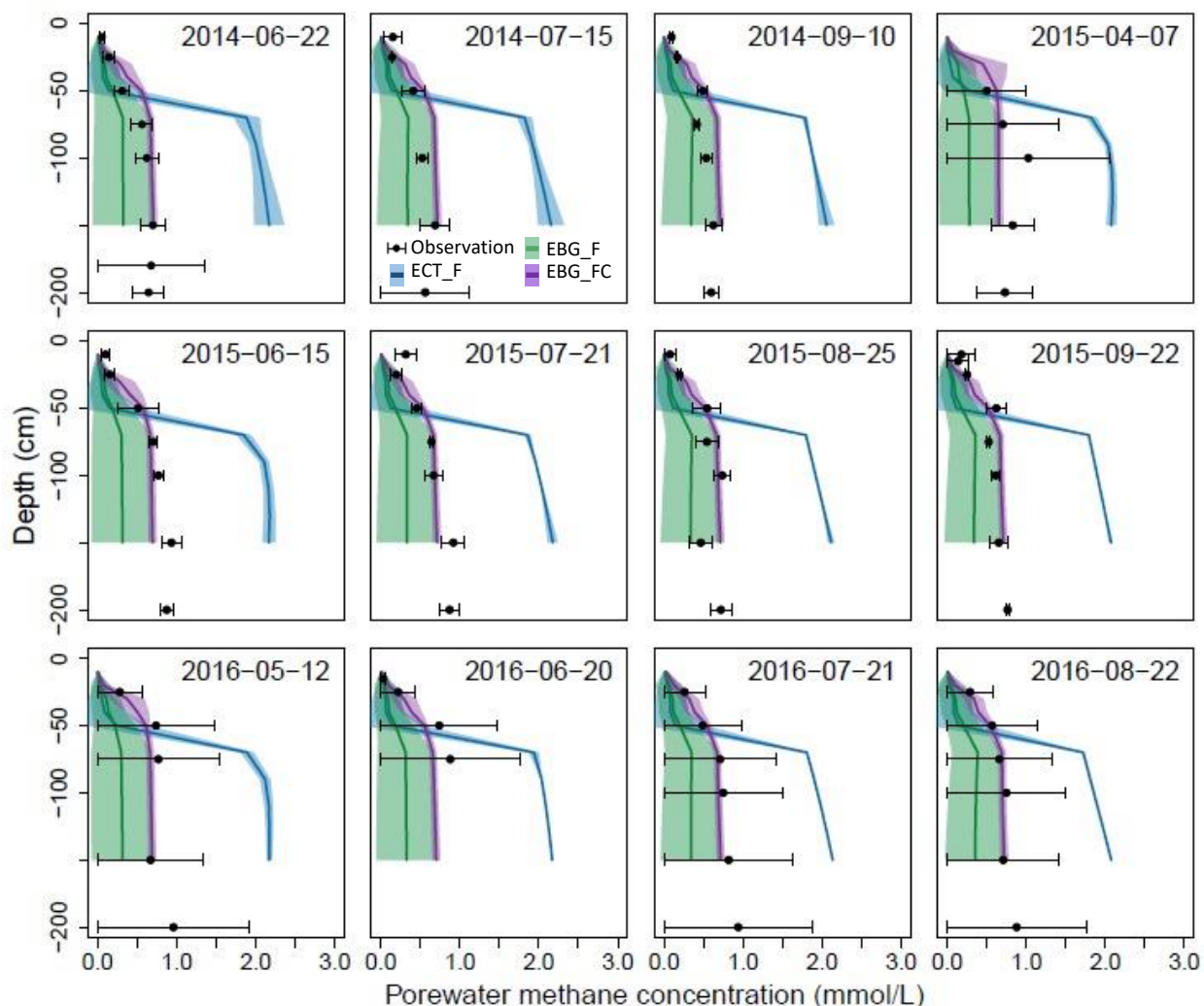
400 Figure 4. Observed versus simulated pore water CH 4 concentration profiles. Black dots are observed concentrations measured from piezometer samples. Blue lines are the ECT model simulated concentrations based on the parameter probability distributions (PPDs) constrained by CH 4 flux data (ECT_F). Green lines are the EBG model simulated concentrations based on the PPDs constrained by CH 4 flux data (EBG_F). Purple lines are the EBG model simulated concentrations based on the PPDs constrained by both CH 4 flux and concentration data (EBG_FC). All midlines and shaded areas correspond to the means and standard deviations, respectively from 500 model simulations with parameters randomly drawn from the posterior distributions.
