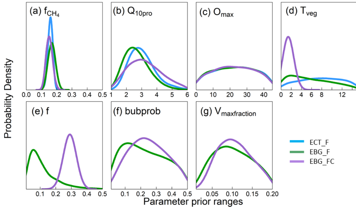
Figure 2. Posterior distribution of parameters that govern methane emission processes from data-model fusion. Parameters are defined in Table 2. (a) and (b) are parameters related to methane production, (c) is a parameter related to methane oxidation, (d) is a parameter related to plant transport, and (e)–(g) are parameters related to ebullition. X axes indicate the prior ranges of parameters used for data-model fusion. The blue lines are the parameter posterior distributions (PPDs) from the ECT model structure trained with CH_4 emission data (ECT_F). The green lines are the PPDs from the EBG model structure trained with CH_4 emission data (EBG_F). The purple lines are the PPDs from EBG trained with both CH_4 emission and CH_4 concentration data (EBG_FC). Well-constrained parameters have a unimodal distribution whereas poorly constrained parameter distributions tend to be flat.
