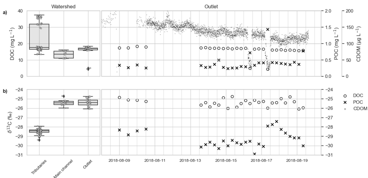
Figure 3. DOC concentrations (mg/L) measured within tributaries, main channel and outlet (panel A, left), and POC (mg/L; cross-markers), DOC (mg/L; circles; please note that the scale is on left panel and applies on the right panel as well) and cDOM (μg/L; filled small circles) concentrations within stream water at the watershed outlet over time (panel A, right). \delta^{13}\text{C} -DOC isotopic signal within tributaries, main channel and outlet (panel B, left), and \delta^{13}\text{C} -DOC and \delta^{13}\text{C} -POC over time at the catchment outlet (panel B, right). Note that two clear drops in the CDOM measurements on the 16 th and 17 th of August mark a storm event. This is also visible in the \delta^{13}\text{C} -POC and to lesser extent \delta^{13}\text{C} -DOC source shift (B, right) around these dates.
