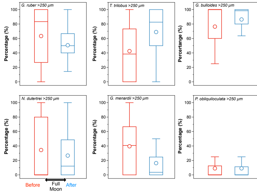
Figure A2. Size class distribution of the six selected species. Globigerinoides ruber , N. dutertrei , and G. menardii show a reduction in the proportion of the size class >250 μm after full moon (blue). The large difference in their median values suggest synchronized reproduction; P. obliquiloculata shows no differences in the size class distribution before (red) and after (blue) full moon; Globigerina bulloides and T. trilobus show an increase in the proportion of larger organisms after the full moon the 1st and 3rd quartiles; median values are shown by bar and circles represent mean values.
