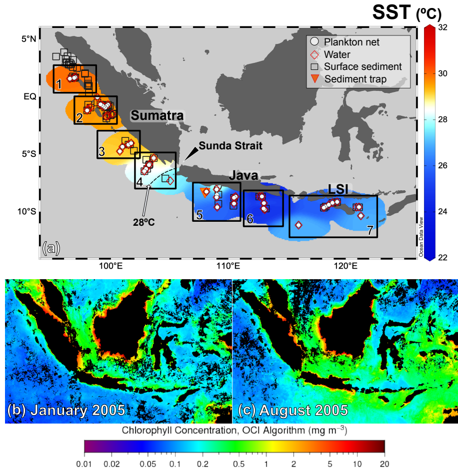
Figure 1. (a) Distribution of the in-situ sea surface temperature in the study area during PABESIA cruise on board of R/V Sonne in August 2005 (Hebbeln and cruise participants, 2006). The study area was divided into seven land-sea transects (numbered rectangles). The stations are divided into plankton net (white circles) and water (red diamond). The location of the sediment trap (Mohtadi et al., 2009) and surface sediments (Mohtadi et al., 2007) are indicated by triangle and squares, respectively. Upper ocean chlorophyll- a (Chl- a ) (retrieved from https://oceancolor.gsfc.nasa.gov ) during (b) January (Non-monsoon) and (c) August (SE-monsoon) 2005 i.e., the sampling period. Temperature map was created with Ocean Data View 5.2.1 (Schlitzer, 2021).
