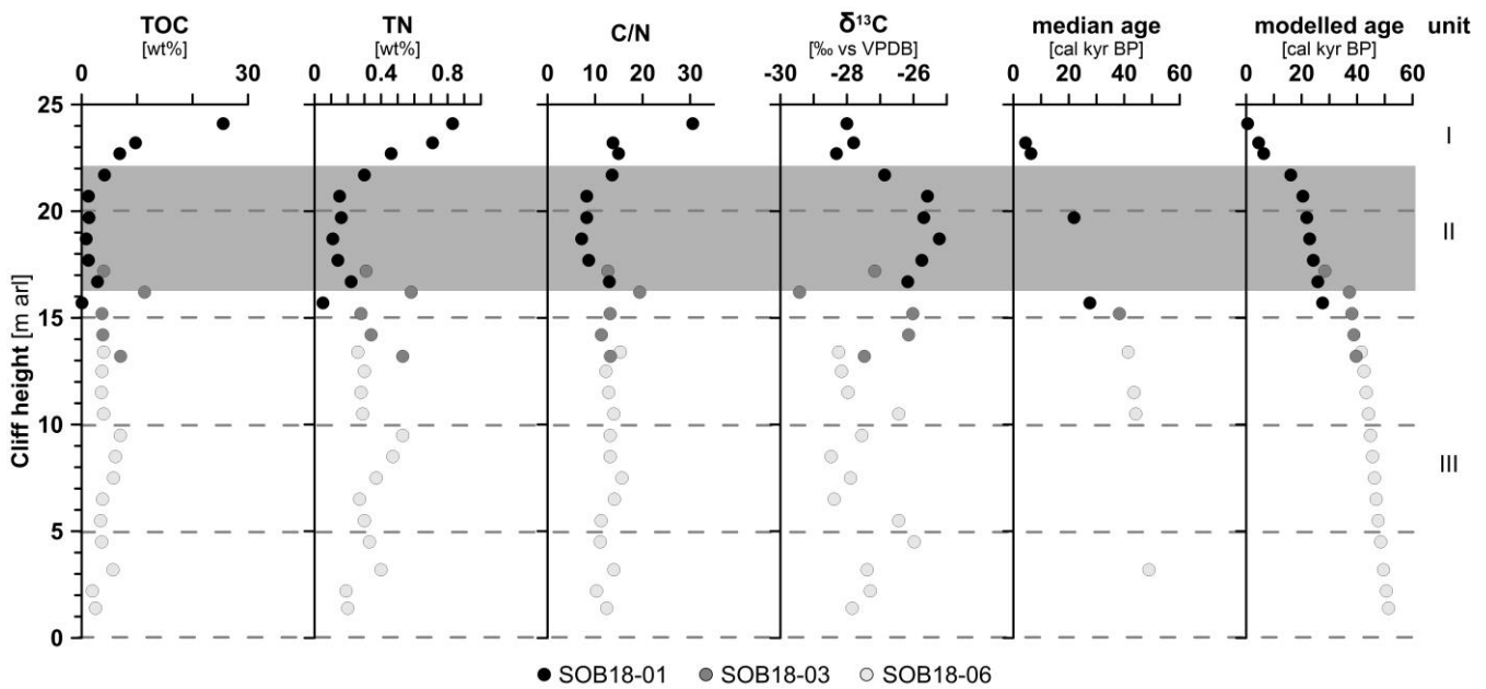
780 Figure 2: Biogeochemical parameters of the Sobo-Sise Yedoma cliff: total organic carbon (TOC) content, total nitrogen (TN) content, carbon over nitrogen (C/N) ratio, bulk stable carbon isotope ratios ( \delta^{13}\text{C} ), radiocarbon ages and modelled age in calibrated years before present (cal kyr BP). Data points are displayed over cliff height from cliff top at 25 m above river level (arl) to cliff bottom at 0 m arl. The three sections of SOB18 are plotted separately for each parameter (black, dark grey and light grey circles). Units I, II (grey rectangle) and III correspond to Marine Isotope Stage (MIS) 1 to 3, respectively. The radiocarbon ages were published in Wetterich et al., 2020a).
