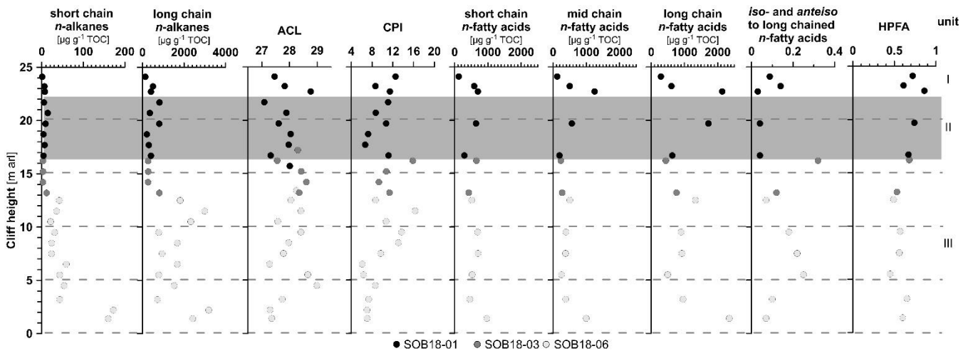
785 Figure 3: Biomarker parameters of the Sobo-Sise Yedoma cliff. First four columns: n -Alkane parameters, like short chain ( \text{C}_{14}\text{-C}_{20} , concentration for microbial and algal production), and long chain ( \text{C}_{21}\text{-C}_{33} , for higher land plants) n -alkane concentrations, both in \mu\text{g/g}\cdot\text{TOC} \text{g}^{-1}\cdot\text{TOC} . After that the n -alkane average chain length (ACL 23-33 ) and n -alkane carbon preference index (CPI 23-33 ) is shown. Last five columns: n -fatty acid based parameters, like short ( \text{C}_8\text{-C}_{20} , microbial estimator), mid chain ( \text{C}_{21}\text{-C}_{23} , estimation for different inputs, for instance from Sphagnum moos species) long ( \text{C}_{24}\text{-C}_{32} , higher land plants) n -fatty acid concentrations in \mu\text{g/g}\cdot\text{TOC} \text{g}^{-1}\cdot\text{TOC} . After that the ratio of iso - and anteiso -branched saturated fatty acids ( \text{C}_{11} , \text{C}_{13} , \text{C}_{15} and \text{C}_{17} ) to mid and long 790
