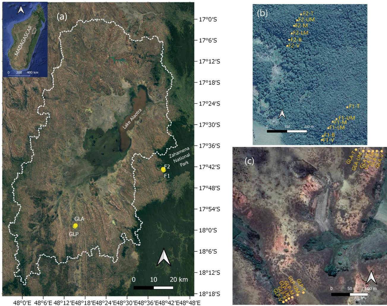
710 Figure 1: (a) Location of the study region with indication of the sampled hillslope profiles. The dotted white line delineates the watershed of the Lake Alaotra Basin. GLA and GLP are the two convex hillslopes under grassland, F1 and F2 the two forested convex hillslopes in the Zahamena National Park. Satellite view of the two forest transects (b) and the two grassland transects (c). (© Google Earth 2020).
