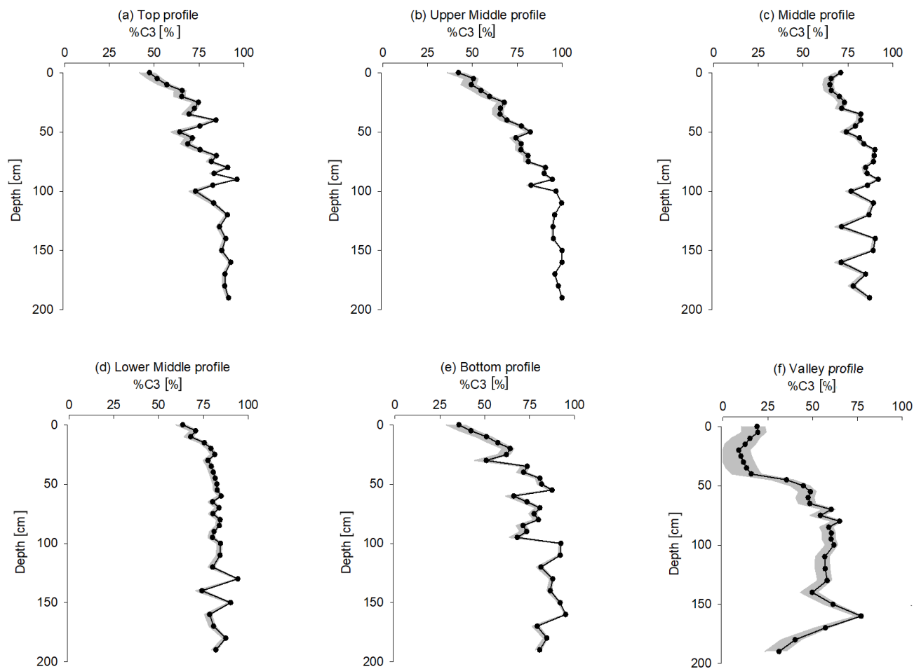
730 Figure 6: Variation with depth of the fraction of remaining forest SOC for the grassland profiles. The black line represents the variation of %C3 by taking -13.8\text{‰} as the reference value of \delta^{13}\text{C} SOC under permanent C4 vegetation. The grey area represents the range of %C3 by using a reference range of -15\text{‰} to -13\text{‰} as the \delta^{13}\text{C} SOC under permanent C4 vegetation.
