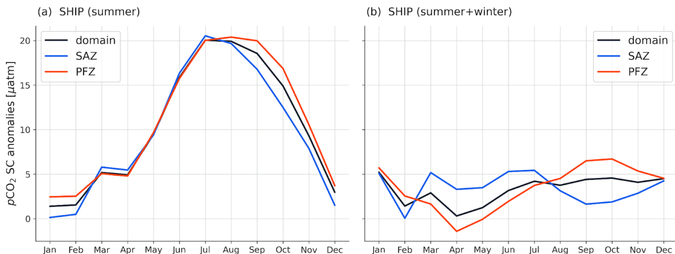
625 Figure 7: Anomalies of the mean surface ocean p\text{CO}_2 seasonal cycle (SC) reconstructions from two SHIP-only experiments. Panel (a) shows the p\text{CO}_2 SC anomalies from the SHIP (summer-only)-based reconstruction in the whole domain, the SAZ, and the PFZ; and in contrast, panel (b) shows the p\text{CO}_2 SC anomalies from the SHIP (summer + winter)-based reconstruction for the whole domain, the SAZ, and the PFZ.
