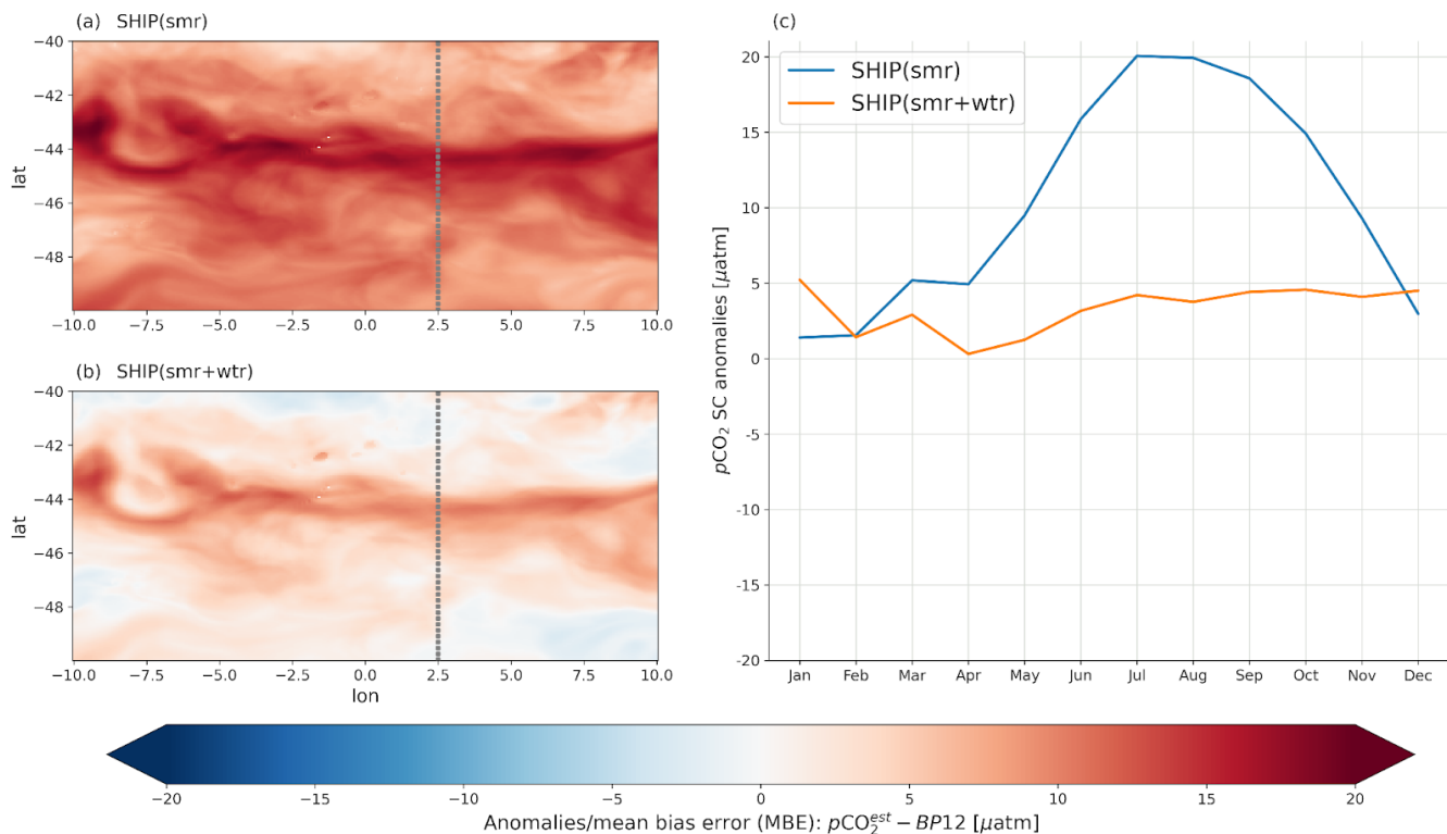
455 Figure 5: Reconstruction anomalies for the idealized SHIP experiment where the idealized ship sampled the domain based on the sampling regimes/scenarios, SHIP(smr) for summer, SHIP(smr+wtr) for summer and winter. Panels (a) and (b) show the maps of the reconstruction anomalies according to the two sampling regimes SHIP(smr), and SHIP(smr+wtr) respectively; panel (c) shows the anomalies of the mean seasonal cycle (SC) reconstruction based on these two sampling regimes; that is, SHIP(smr) and 460 SHIP(smr+wtr). The meridional dotted grey line in panels (a) and (b) illustrates the sampling line (summer & winter) and serves as a reminder of how SHIP sampling was performed.
