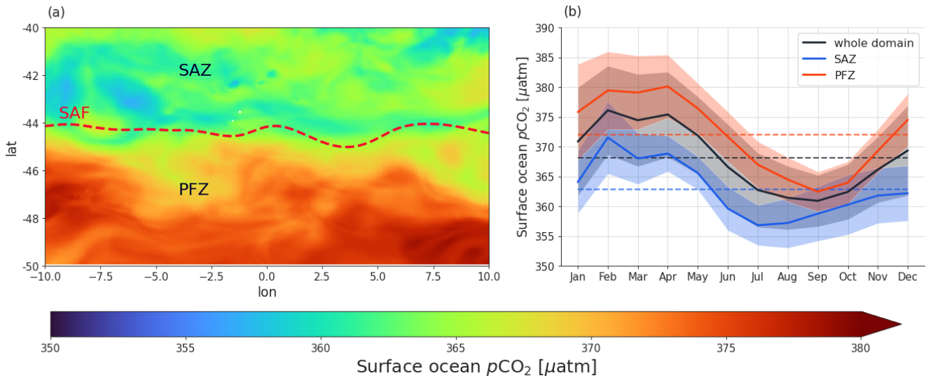
425 Figure 4: Characterisation of the spatial and temporal surface ocean p\text{CO}_2 annual mean state within the selected 10^\circ -by- 20^\circ experimental domain located in the northern ACC that corresponds to SPSS biome (Fay and McKinley, 2014) as shown in Fig. 1a. Panel (a) shows the map of mean annual p\text{CO}_2 from the BIOPERIANT12 (BP12) model. It shows that the domain is characterized by a regional meridional gradient including the Sub-Antarctic Front (SAF) (red dashed line) as well as mesoscale gradients in both SAZ and PFZ; panel (b) shows the mean seasonal cycles for surface ocean p\text{CO}_2 in the BP12 model domains (SAZ, SAF and PFZ) where the dashed lines indicate the magnitude of the annual mean for each domain - 368.16 \mu\text{atm} (domain), 362.85 \mu\text{atm} (SAZ), and 371.78 \mu\text{atm} (PFZ).
