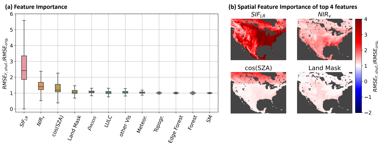
Figure 5. Feature Importance. (a) shows the total RMSE of the permuted feature divided by the RMSE without feature permutation (b) shows the RMSE of each pixel with permuted features divided by the RMSE without feature permutation. Some input variables are clustered and all variables of that class are permuted at the same time. \rho_{MODIS} : all 7 MODIS bands; LULC: all 11 land cover classes; other VIs: kNDVI , NDVI , EVI ; Meteor.: temperature, precipitation, temperature with 16 day delay, precipitation with 16 days delay; SM: surface soil moisture and sub-surface soil moisture.
