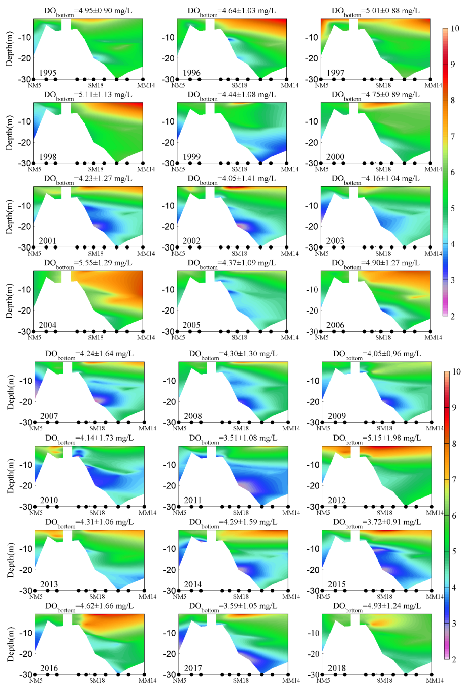
Figure A1. Vertical distributions of average DO of all summer cruises (three months). Note that the mean values and standard deviations of bottom-water DO were also shown at the top of each subplot.
