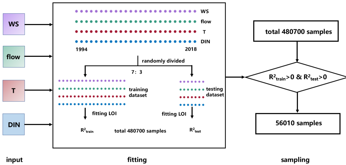
620 Figure A4. Flowchart describing the fitting of LOI and the cases sampling used for analysis.
