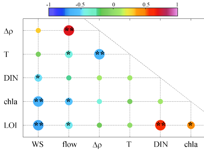
Figure 8. Pearson correlation coefficients ( r ) among the wind speeds (WS), freshwater discharges (flow), vertical density differences ( \Delta\rho ), bottom temperature (T), surface DIN concentrations (DIN), surface Chl a concentrations (Chl a ), and LOI. Note that the color of dots show the correlation coefficients, and the symbols * and ** represents the significant level at p < 0.05 and p < 0.01 , respectively.
