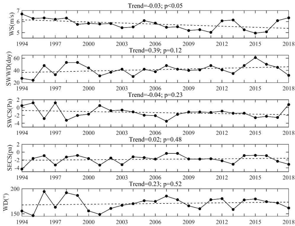
610 Figure A2. Average wind speed (WS), southwestern wind duration (SWWD), southwestern wind cumulative stress (SWCS), southeastern wind cumulative stress (SECS), average wind direction (WD) in summer, and their long-term trends during 1994-2018. Note that the negative values of SWCS and SECS represent southwestern and southeastern wind, respectively. The trends and significant p values were shown in the title of each subgraph.
