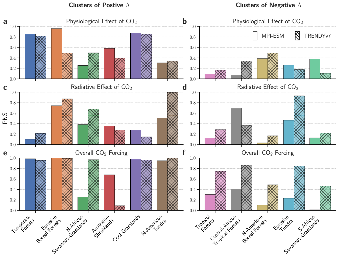
Figure 5. Probabilities of sufficient and necessary causation (PNS) of LAI changes in response to CO 2 for eleven clusters. Probabilities of sufficient and necessary causation (PNS) of LAI changes in response to the effects of rising CO 2 for eleven clusters. Bar charts represent PNS of LAI changes in response to the physiological effect (a, b), radiative effect of CO 2 (c, d) and all anthropogenic forcings (e, f). Different colors represent the identified clusters of substantial change in LAI. Panels on the left comprise clusters that show consistent greening, panels on the right represent emerging browning clusters (observed net leaf area loss in the period 2000–2017; attribution is conducted only for significant decreasing trends; Data and Methods ; see Section 2 for details). The two types of bar illustrate the two different ensembles of model simulations (left: MPI-ESM, right: TRENDYv7).
