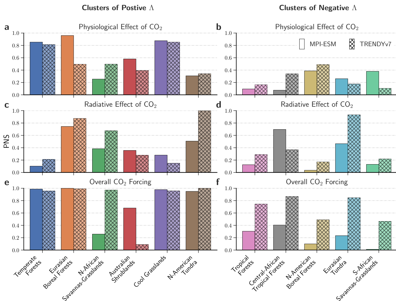
Figure 4. Probabilities of sufficient and necessary causation (PNS) of LAI changes in response to CO 2 for eleven clusters. Bar charts represent PNS of LAI changes in response to the physiological effect (a, b), radiative effect of CO 2 (c, d) and all anthropogenic forcings (e, f). Different colors represent the identified clusters of substantial change in LAI. Panels on the left comprise clusters that show consistent greening, panels on the right represent emerging browning clusters (observed net leaf area loss in the period 2000–2017; attribution is conducted only for significant decreasing trends, Data and Methods). The two types of bar illustrate the two different ensembles of model simulations (left: MPI-ESM, right: TRENDYv7).
