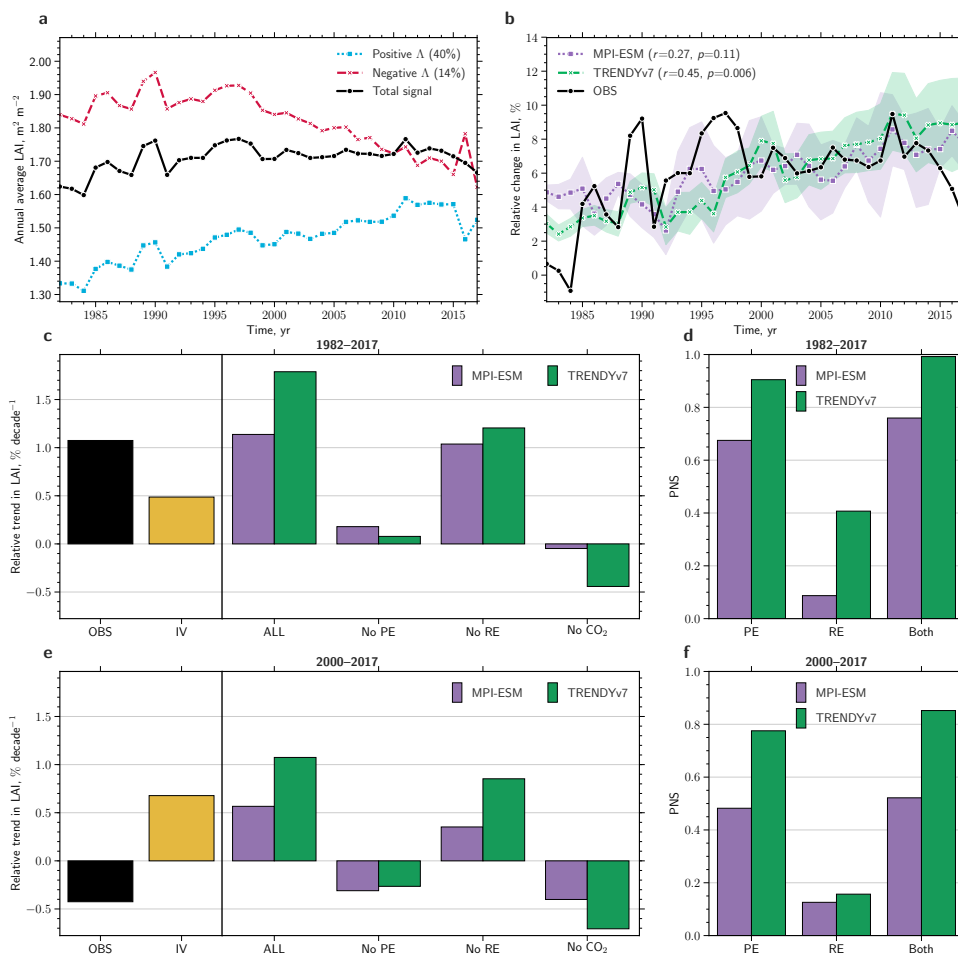
Figure 3. Global driver attribution of changing natural vegetation for the entire period versus the second half of the observational record. a Time series of the area-weighted annual average LAI (GIMMS LAI3g, 1982–2017) for regions of positive (blue dotted line) and negative sensitivity (red dashed line) to rising atmospheric CO 2 concentration ( \Delta ) of natural vegetation. Black solid line represents the overall signal of all pixels. The percentages in brackets in the legend represent the greening and browning proportions with respect to the total area. b Time series of changes in LAI relative to the average state from 1982–1984, comparing observations (black solid line) with historical simulations, where the green dashed line denotes the ensemble mean of 13 offline-driven land surface models (TRENDYv7, Data and Methods), and the purple dotted line denotes the average of an ensemble of multi-realizations with a fully-coupled Earth system model (MPI-ESM, Data and Methods). The colored shading represents the 95% confidence interval estimated by bootstrapping. The correlation coefficients (including significance level) of the observed and simulated time series are displayed in brackets in the legend. c Bar chart showing relative trends in LAI (in % yr -1 ) of the total observed signal (black) and for factual (all historical forcings; ALL) as well as for counterfactual simulations, i.e. no historical CO 2 forcing (No CO 2 ), all historical forcings except the physiological effect (No PE) or the radiative effect (No RE) of atmospheric CO 2 , as estimated by TRENDYv7 (green) and MPI-ESM (purple). The yellow bar represents internal variability (IV) derived from all simulations (control, factual and counterfactual). d Probabilities of necessary and sufficient causation (PNS) of the change in LAI, comparing the physiological (PE) and radiative effect (RE) of CO 2 as well as their combined effect (Both). e as in c but for the period 2000–2017. f as in d but for the period 2000–2017.
