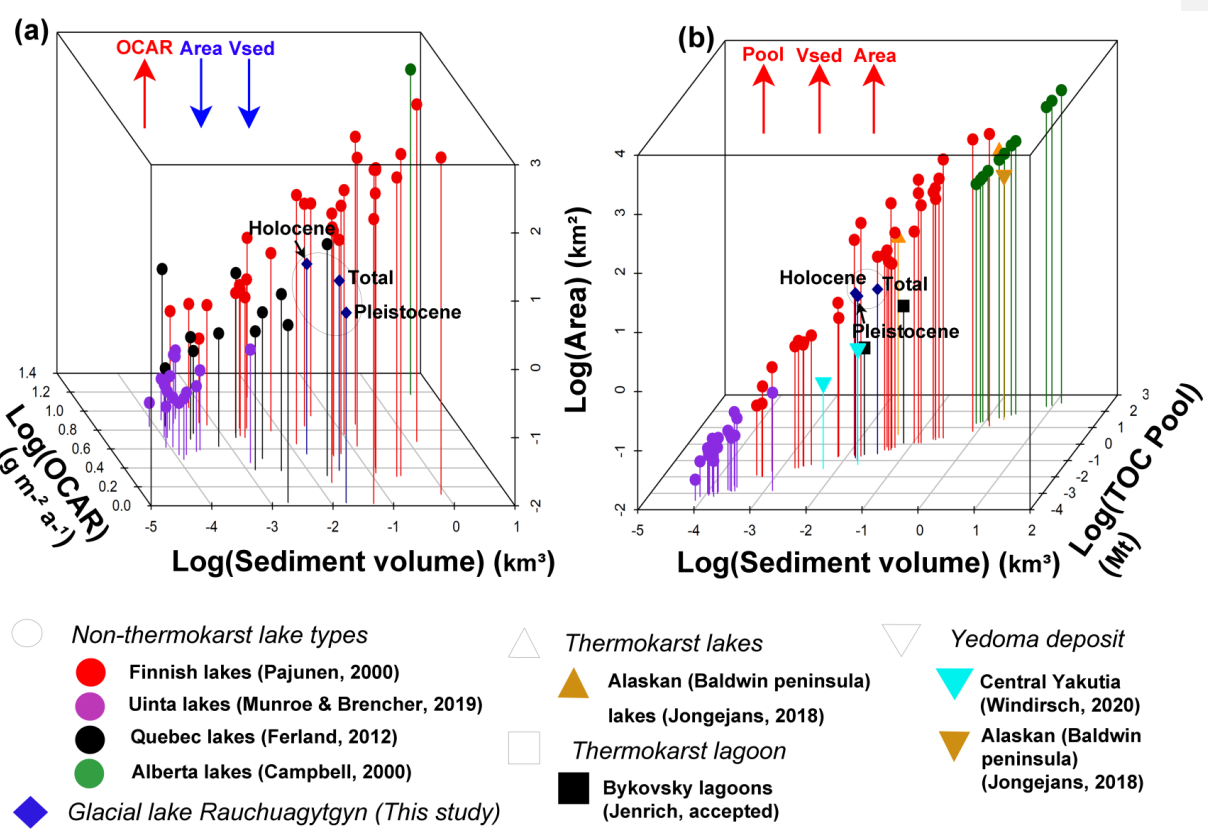
Figure 9. (a) 3D log scatter plot of organic carbon accumulation rate (OCAR) vs lake sediment volumes and surface areas. The average carbon accumulation rate for the Holocene at Lake Rauchaugytgn closely resembles that of Holocene-age Finnish and Quebec lakes and generally lies on a trajectory of increasing OCAR with decreasing sediment volume and area. (b) 3D log scatter plot of Carbon pool vs sediment volume and area. The Rauchaugytgn data-points are highlighted with ellipses in both plots. Rauchaugytgn displays similar carbon pools to Finnish lakes, Bykovsky thermokarst lagoons and Central Yakutian Yedoma-yedoma deposits. Rauchaugytgn Sediments-sediments possess however significantly lower carbon pools relative to volume and area than Alaskan (Baldwin Peninsula thermokarst lake and yedoma deposits and Alberta lakes.
