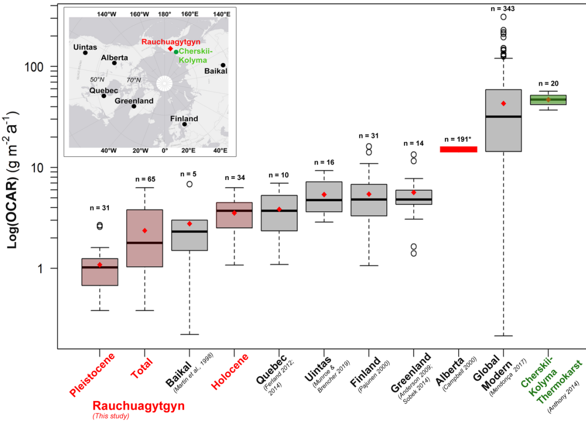
Figure 8. Comparison Log-boxplot of average organic carbon accumulation rates (OCARs) for Lake Rauchaugytgn with carbon accumulation rates from other regions. Rauchaugytgn OCARs include a total of 65 downcore points and plot close to Boreal-boreal lake sites and to Lake Baikal (ESRI 2020). The global modern dataset of Mendonça et al., 2017 included OCARs-OCARs from 343 globally distributed lake sites (see Text S1). Only the average OCAR across Alberta lakes was provided in Campbell et al. 2000 and hence the average is displayed as a red bar. Study references are quoted below the study regions.
