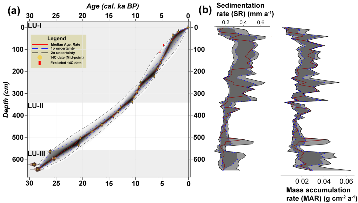
Figure 4. (a) High-resolution age-depth model for sediment core EN 18218 created from 23 radiocarbon dates with sigma uncertainty range. (b) Sedimentation and mass accumulation rates (dark red lines) and 1 and 2σ uncertainty ranges (dark and light grey ribbons).
