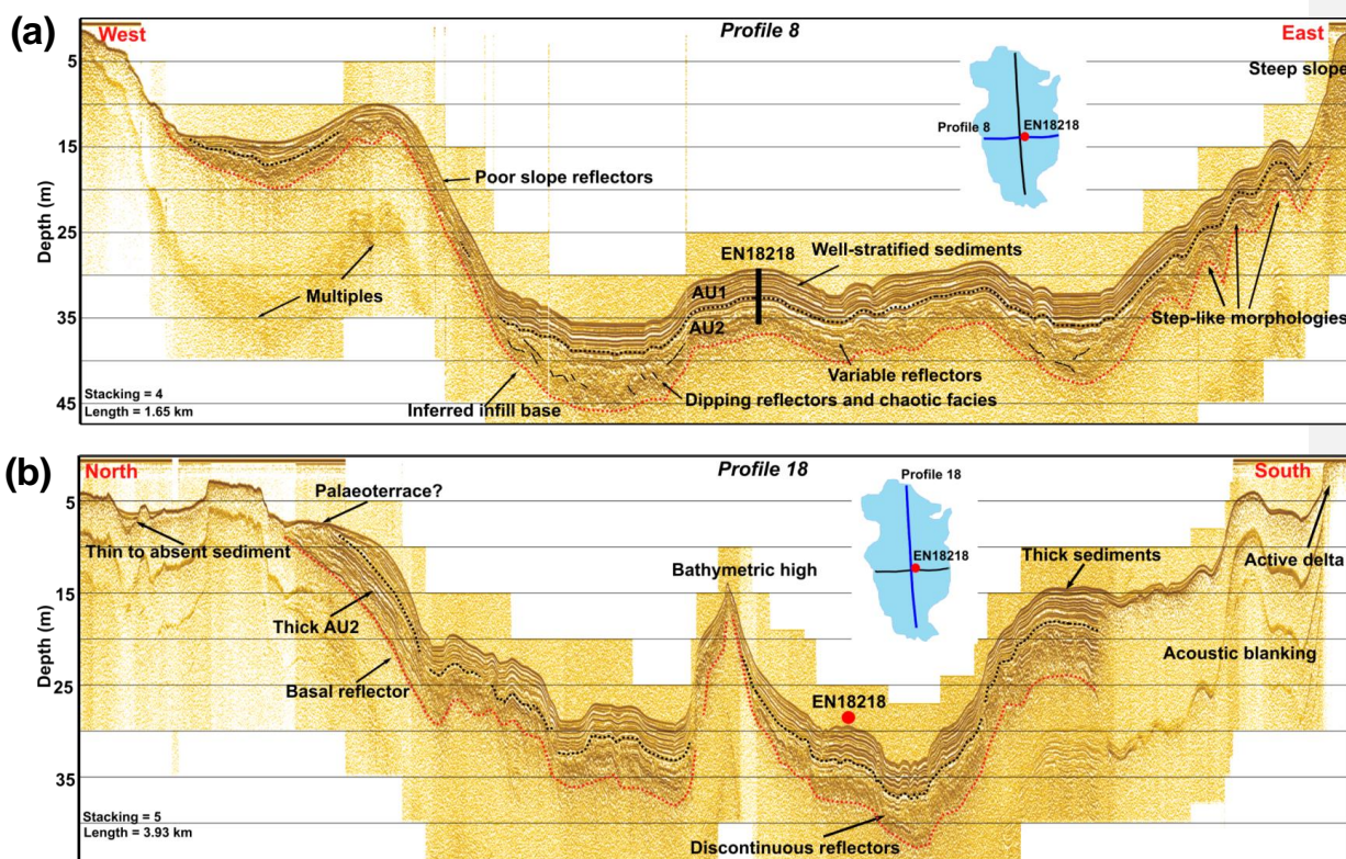
Figure 2. Interpreted hydro-acoustic profiles from Lake Rauchaugytyn (Profile 8 and Profile 18). Both profiles pass close to the drilling location of EN18218. Shown are inferred major hydroacoustic boundaries defined that are connected with major lithological changes recorded by EN18218 and interpreted across the basin.
