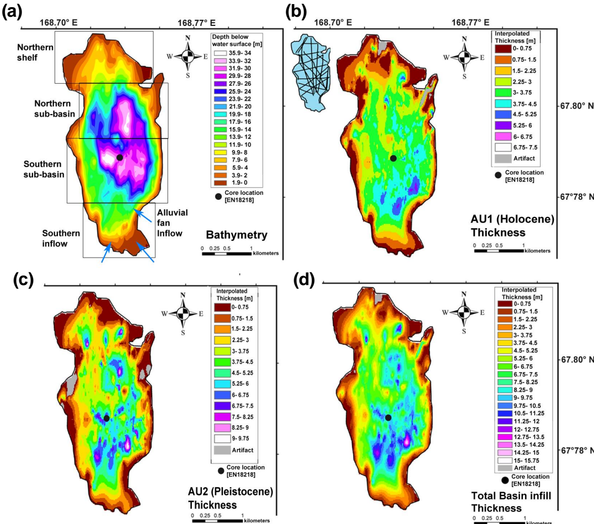
Figure 3. (a) Interpolated high-resolution lake bathymetry with morphological regions denoted by black boxes. (b) Interpolated AU1 thicknesses. Blue and pink colors denote the thickest sediment within the southern sub-basin. (c) Interpolated sediment thicknesses within AU2. Similarly to AU1, the greatest thicknesses are predominantly located in the southern sub-basin but with other locations in the northern-sub basin showing thick sediments too. (d) Whole sediment package interpolated thickness. Thin sediment is found proximal to the basin margins and at the north-western shelf. The sediment distribution generally reflects sediment focussing into the deeper lake at greater water depths. Interpolation artefacts are attributed to data sparsity and difficulties in tracing reflectors in some regions due to acoustic blanking that led to erroneous interpolation, with larger artefacts being hence excluded.
