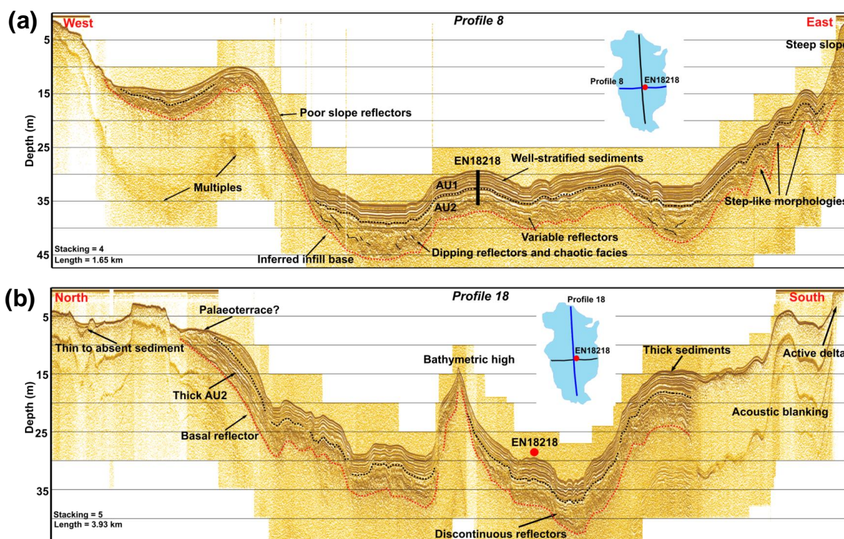
Figure 2. Interpreted hydro-acoustic profiles from Lake Raachuagtygyn (Profile 8 and Profile 18). Both profiles pass close to the drilling location of EN18218. Shown are inferred major hydroacoustic boundaries defined that are connected with major lithological changes recorded by EN18218 and interpreted across the basin.
