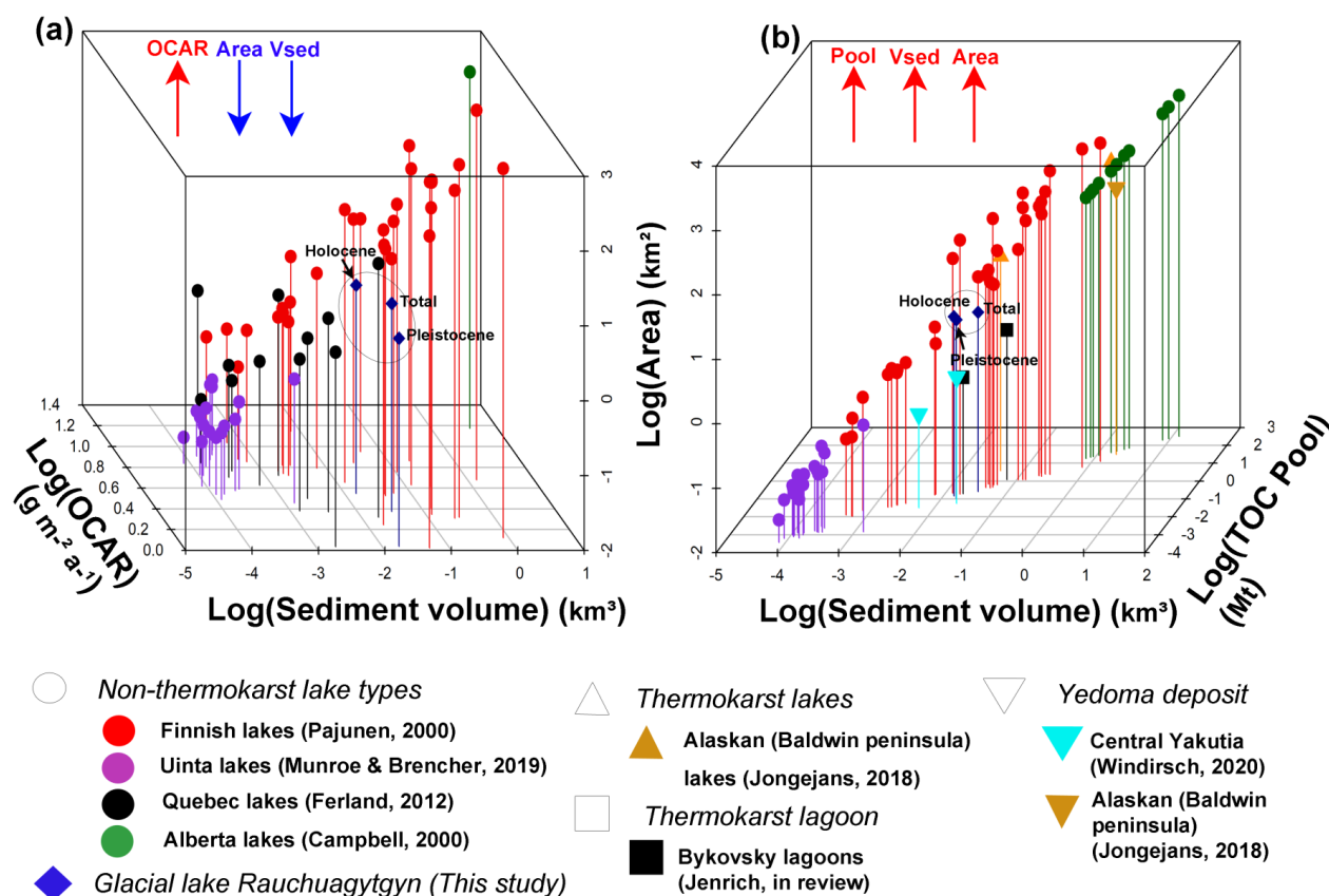
Figure 9. (a) 3D log scatter plot of organic carbon accumulation rate (OCAR) vs lake sediment volumes and surface areas. The average carbon accumulation rate for the Holocene at Lake Rauchaugytgyn closely resembles that of Holocene-age Finnish and Quebec lakes and generally lies on a trajectory of increasing OCAR with decreasing sediment volume and area. (b) 3D log scatter plot of Carbon pool vs sediment volume and area. The Rauchaugytgyn data-points are highlighted with ellipses in both plots. Rauchaugytgyn displays similar carbon pools to Finnish lakes, Bykovsky thermokarst lagoons and Central Yakutian Yedoma deposits. Rauchaugytgyn Sediments possess however significantly lower carbon pools relative to volume and area than Alaskan (Baldwin Peninsula) thermokarst lake and yedoma deposits and Alberta lakes.
