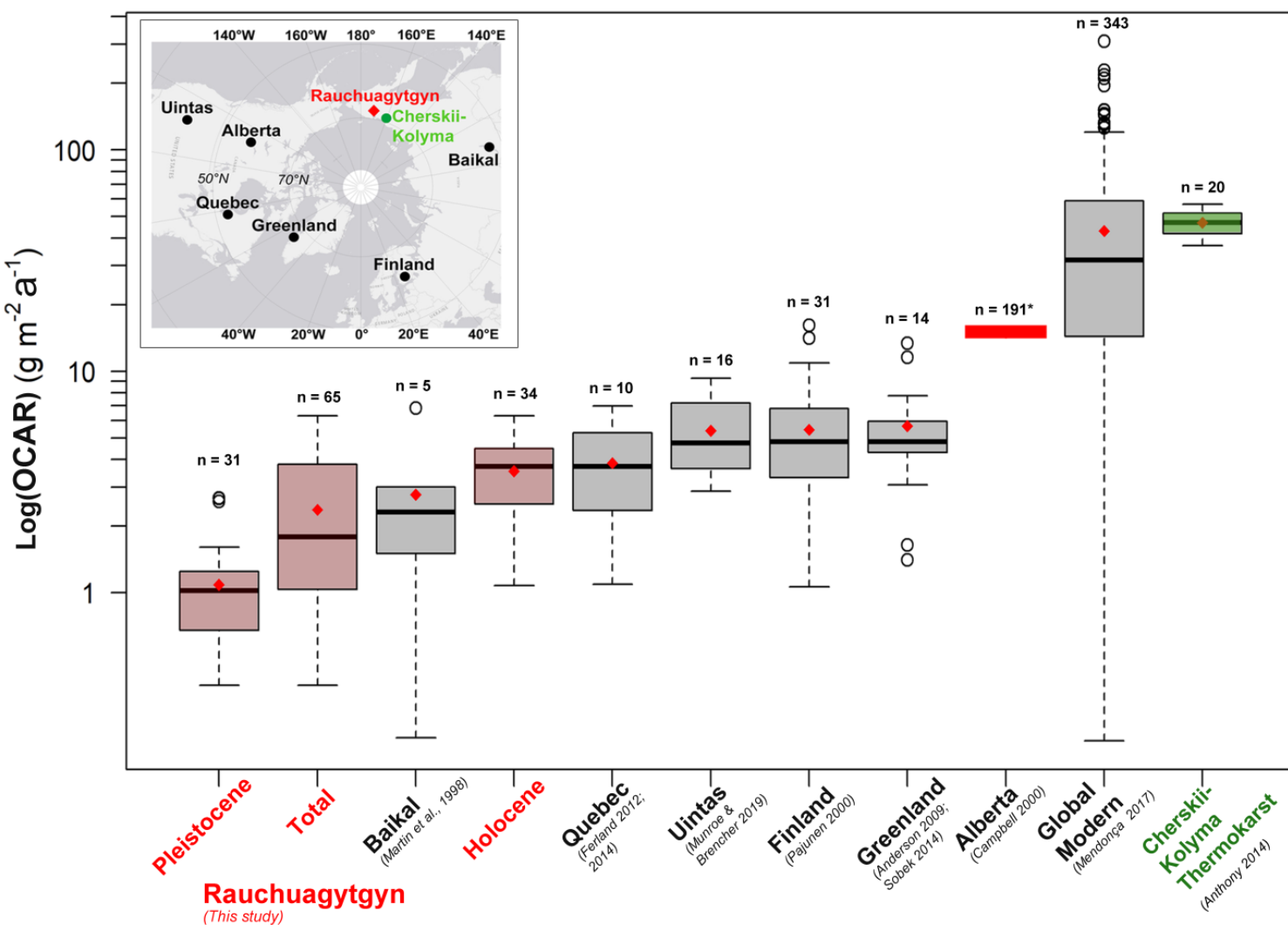
Figure 8. Comparison Log-boxplot of average organic carbon accumulation rates (OCARs) for Lake Rauchaugytgyn with carbon accumulation rates from other regions. Rauchaugytgyn OCARs include a total of 65 downcore points and plot close to boreal lake sites and to Lake Baikal (ESRI 2020). The global modern dataset of Mendonça et al., 2017 included OCARs from 343 globally distributed lake sites (see Text S1). Only the average OCAR across Alberta lakes was provided in Campbell et al. 2000 and hence the average is displayed as a red bar. Study references are quoted below the study regions.
