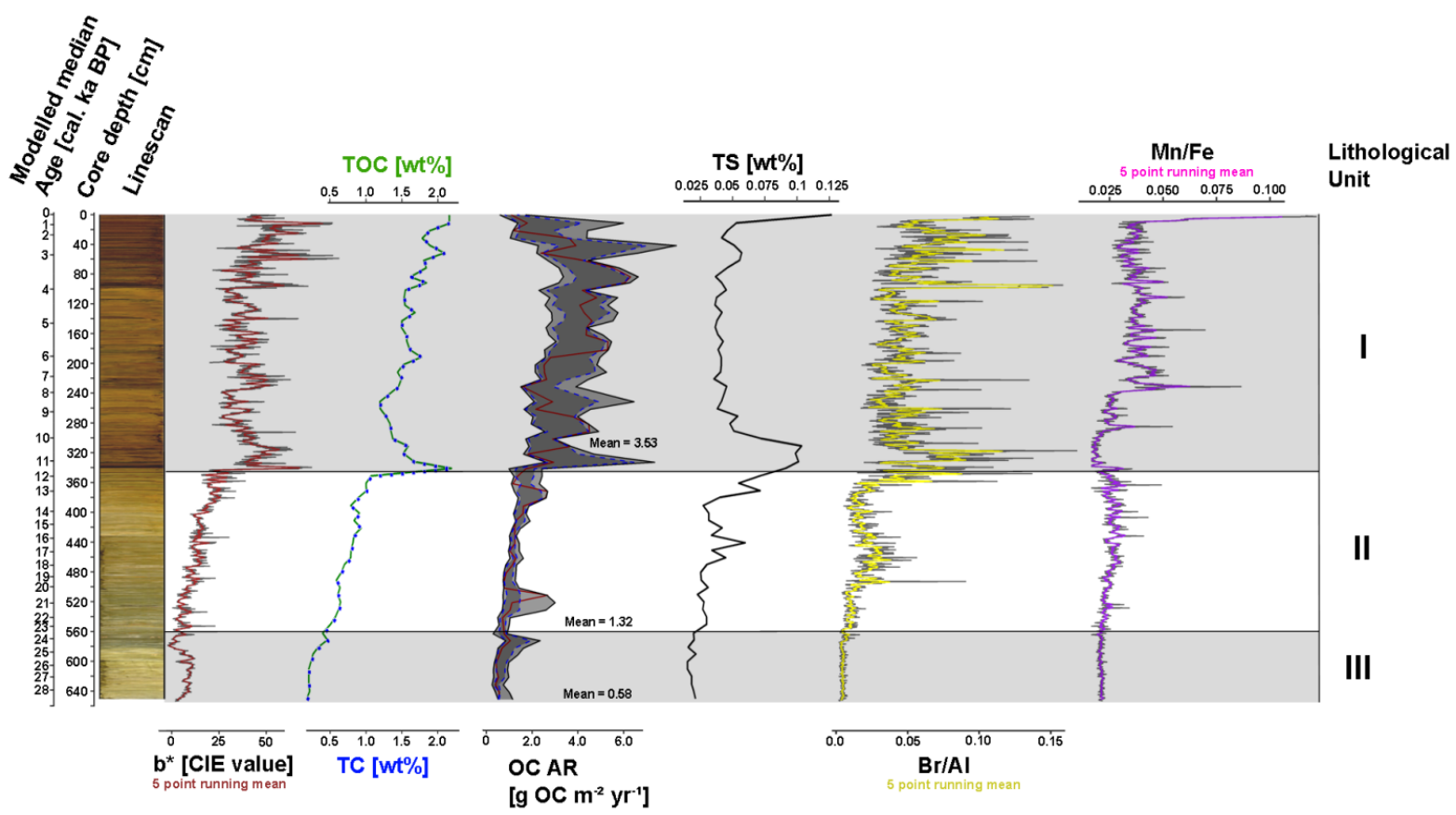
Figure 6. Biogeochemical proxies measured from samples obtained from core EN18218 (TOC, TC, TS) as well as from XRF (Br/Al, Mn/Fe) and line-scanning (b*). Average OCAR (Red line) is plotted alongside sigma uncertainty ranges (grey ribbons) synonymous with descriptions in Figure 4.
