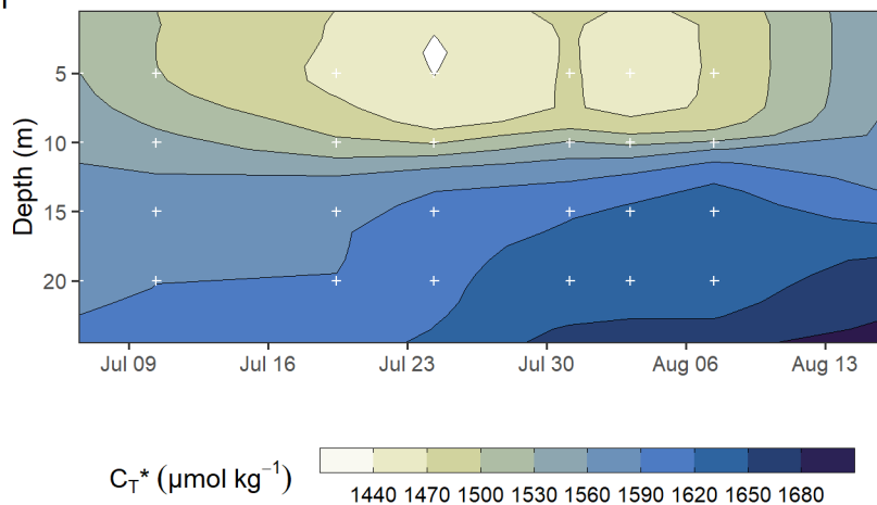
Figure 4. (a) Temperature and (b) C_T^* between July 6 and August 16 displayed as (1) Hovmoeller plots and (2) profiles of cumulative changes since the first cruise on July 6. Mean cruise dates are indicated by the horizontal position of white symbols in (a1) and (b1), and the compensation depth of 12 m is indicated as a red, horizontal line in (a2) and (b2).
