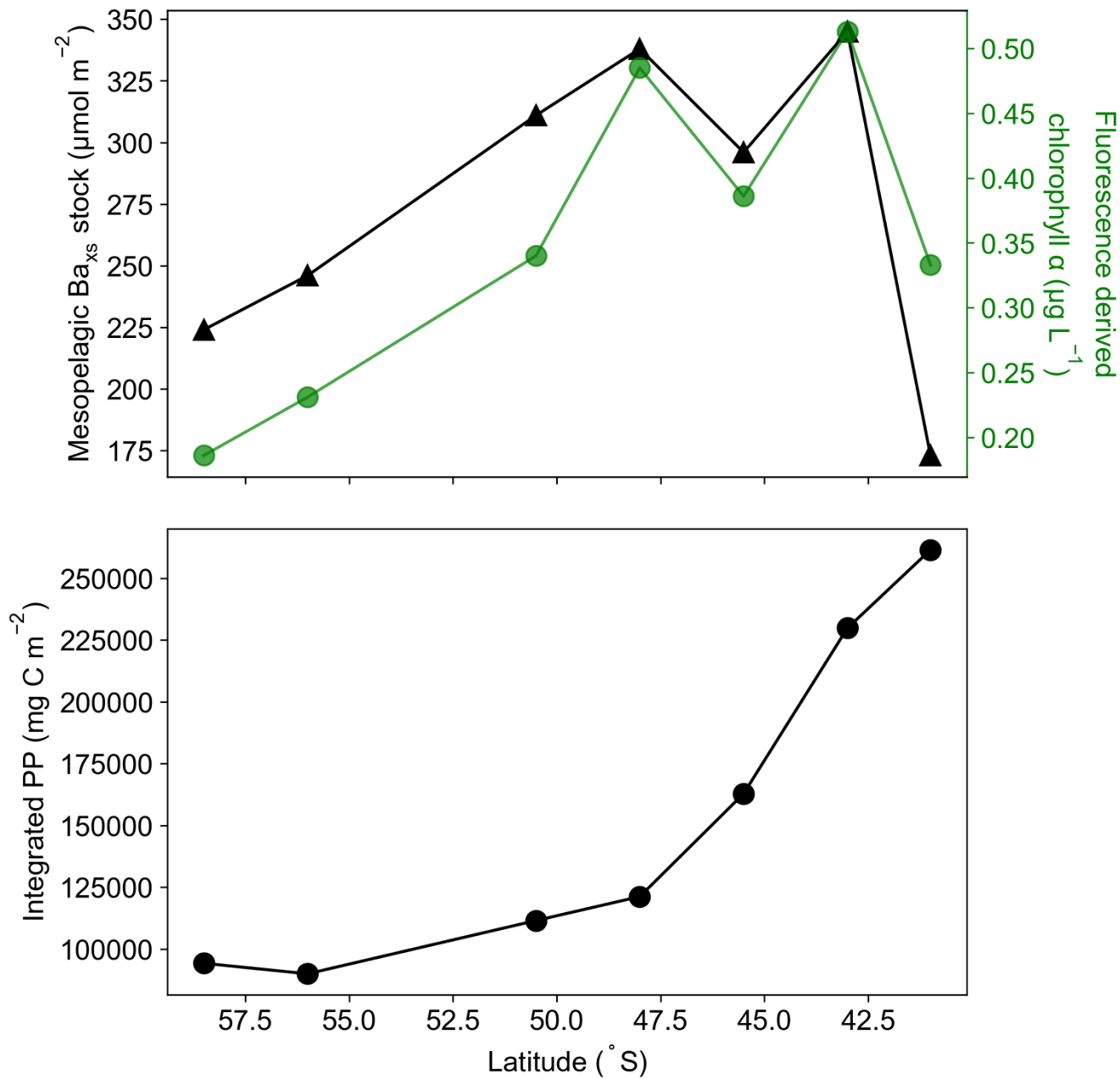
0 1 Figure S1: Top panel is the latitudinal trend, south to north, left to right, of winter integrated mesopelagic Ba xs stock concentrations 2 (black triangles) and surface fluorescence derived chlorophyll a concentrations (green circles) at the time of sampling. The bottom 3 panel is the latitudinal trend of the corresponding integrated remote sensing CbPM PP (black circles)
