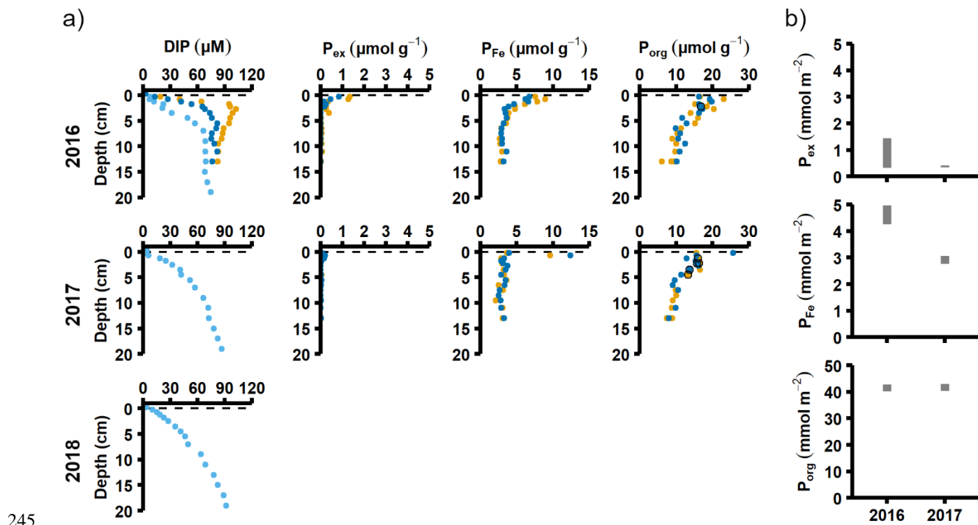
Figure 3. Pore-water and sediment solid phase data from station F. (a) Profiles of pore-water DIP, solid-phase exchangeable or loosely-sorbed P (P ex ), easily-reduced or reactive iron-bound P (P Fe ) and organic P (P org ). Profiles with light blue markers are from big sediment cores (inner diameter 9.9 cm); profiles with dark blue and orange markers are from replicate small sediment cores (inner diameter 6 cm). Markers with black edges are missing data that have been replaced with average concentrations from the slices directly above and below (see appendix B). (b) Excess inventories (min – max range) of P ex and P Fe , and inventories of P org in the top 5 cm.
