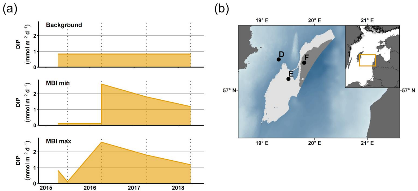
Figure 5. Upscaling of DIP release. (a) DIP release at station F according to three different scenarios: Background, MBI min and MBI max. The lines show the DIP flux according to the different scenarios, the shaded area represents the total DIP release during the period. (b) Sediment areas (western flank of the EGB) used for upscaling calculations. The DIP flux per m 2 in the light grey area (150-190 m) is assumed to be the same as at station E, while the dark grey area (> 190 m) is represented by station F. Bathymetric data from the Baltic Sea Bathymetry Database (version 0.9.3), the map was created using the software ArcMap TM (v. 10.6) by Esri.
