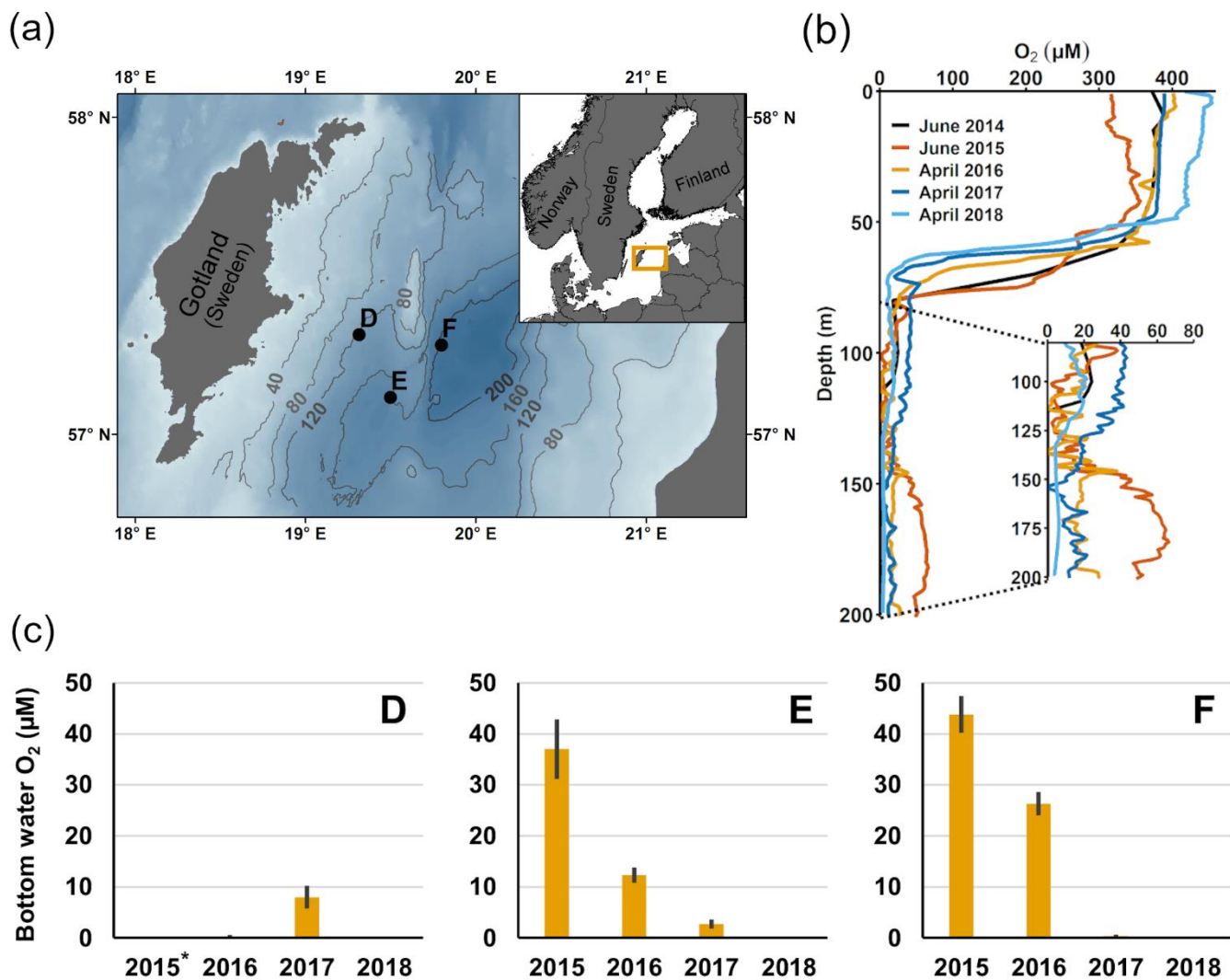
Figure 1. Description of sampling sites and oxygen conditions. (a) Map of the sampling sites in the Eastern Gotland Basin, Baltic Sea. Bathymetric data from the Baltic Sea Bathymetry Database (v. 0.9.3), the map was created using the software ArcMap™ (v. 10.6) by Esri. (b) Water-column profiles of oxygen ( O_2 ). Data from SMHI (SMHI, 2021; 2014, station BY15), Hall et al. (2017; 2015, station F) and van de Velde et al. (2020b; 2016-2018, station F). (c) Bottom-water oxygen ( O_2 ) concentrations at stations D-F measured by optodes on the benthic chamber lander (average \pm standard deviation) \sim 0.2 m above the sediment. The detection limit was 0.5 \mu M . Data from Hall et al. (2017) and van de Velde et al. (2020b). *no measurement.
