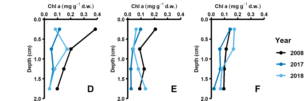
Figure D1. Chlorophyll a profiles. Profiles of chlorophyll a (Chl a) in the top 2 cm of the sediment.
