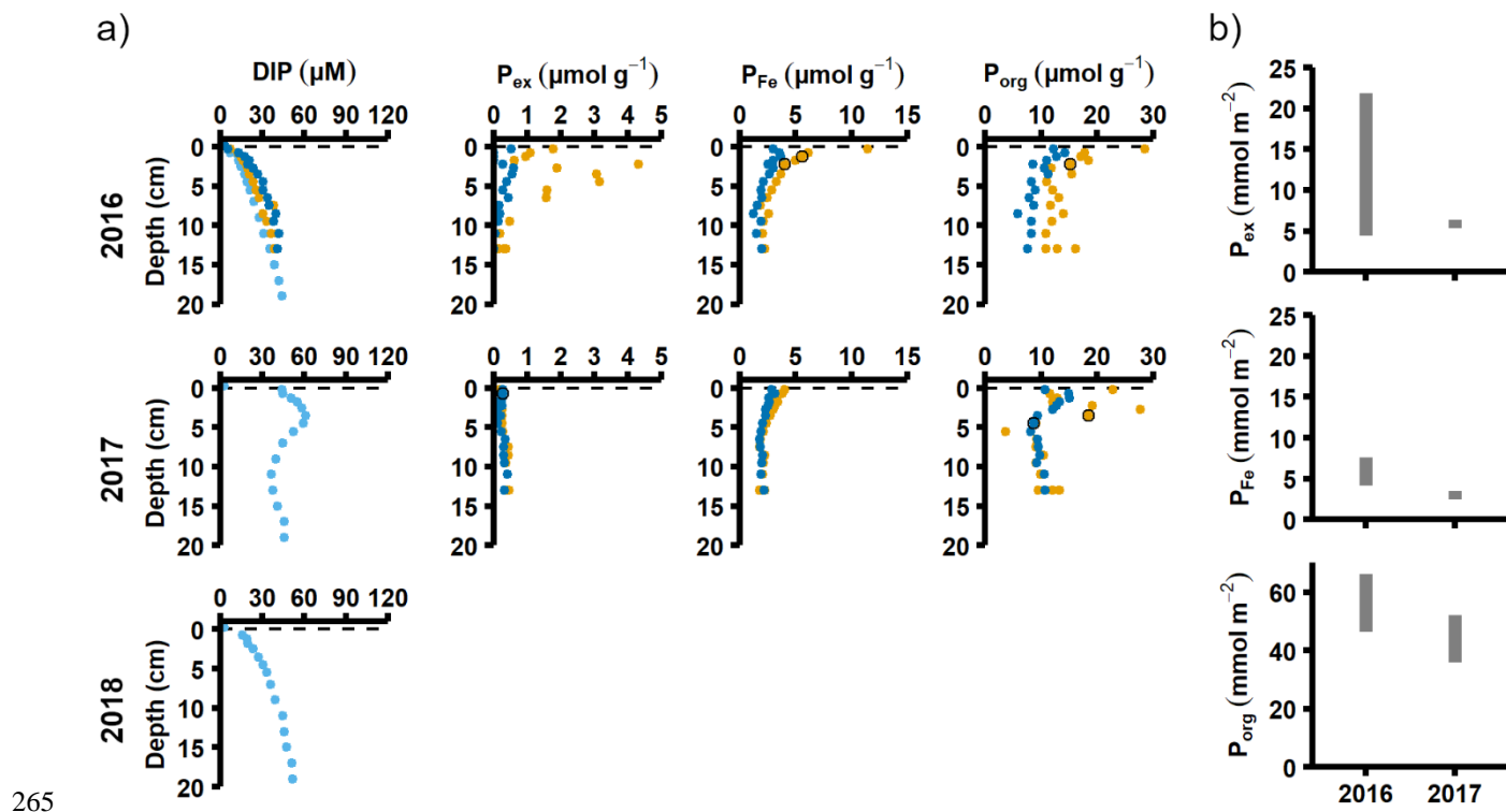
Figure 4. Pore-water and sediment solid phase data from station D. (a) Profiles of pore-water DIP, solid-phase exchangeable or loosely-sorbed P ( P_{ex} ), easily-reduced or reactive iron-bound P ( P_{Fe} ) and organic P ( P_{org} ). Profiles with light blue markers are from big sediment cores (inner diameter 9.9 cm); profiles with dark blue and orange markers are from replicate small sediment cores (inner diameter 6 cm). Markers with black edges are missing data that have been replaced with average concentrations from the slices directly above and below (see appendix B). (b) Excess inventories (min – max range) of P_{ex} and P_{Fe} , and inventories of P_{org} in the top 5 cm.
