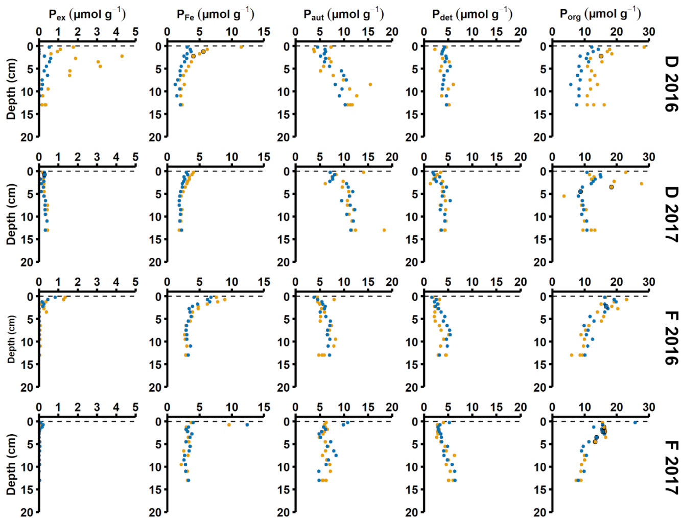
Figure A4. Solid phase phosphorus speciation. P_{ex} – exchangeable or loosely sorbed P, P_{Fe} – easily reduced or reactive iron bound P, P_{aut} – authigenic P, P_{det} – detrital P, P_{org} – P associated with organic matter. The blue and orange markers represent replicate small sediment cores (inner diameter 6 cm).
