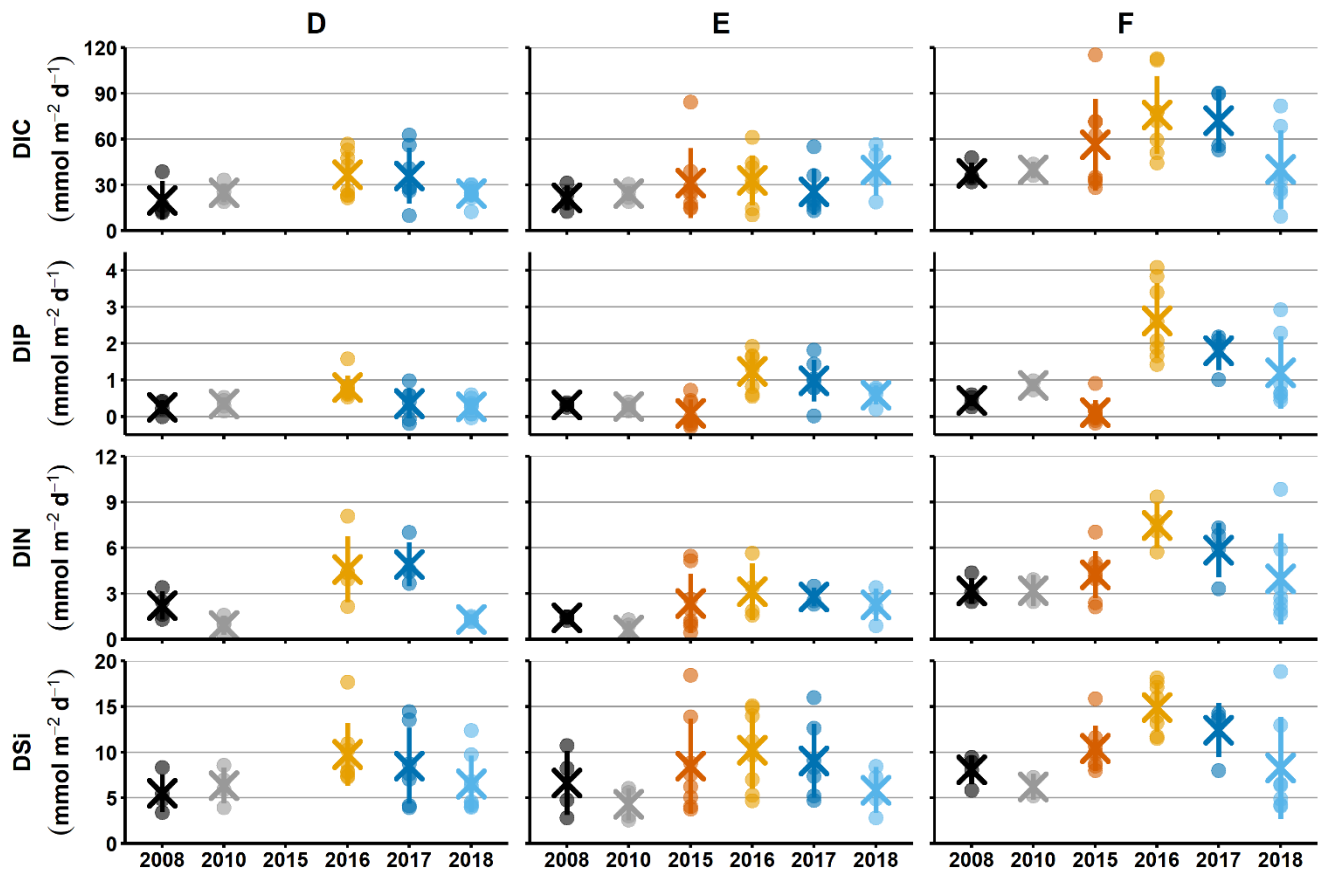
470 Figure A2. Sediment-water fluxes measured with the benthic chamber lander. Flux data are from before the inflow (2008, 2010; Hall et al., 2017; Nilsson et al., 2019; Viktorsson et al., 2013), right after the inflow (2015; Hall et al., 2017) and post inflow (2016-2018; this study). There are no data from station D in 2015.
