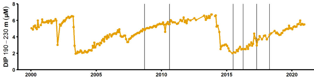
Figure A8. Dissolved inorganic phosphorus concentrations in the deep layer the SMHI station BY15 (SMHI, 2021). The grey lines indicate when samplings for this study were conducted (2008, 2010: August/September; 2015: early July; 2016-2018: April).
