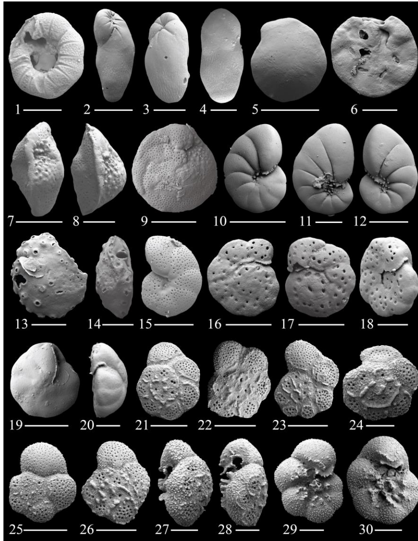
Figure 8. 1. Glabratella mirabilis Seiglie and Bermúdez; 2–4. Elongobula parallela (Cushman and Parker, 1931); 5–6. Eoponidella pulchella (Parker, 1952); 7–8. Amphistegina lessonii (d’Orbingy, 1826); 9. Amphistegina radiata (Fichtel and Moll, 1892); 10–12. Nonionides grateloupii (d’Orbingy, 1826); 13–14. Svratkina acuta (Sidebottom, 1918); 15. Anomalinulla glabrata (Cushman, 1924); 16–20. Anomalinulla sp 1.; 21–30. Pararotalia cananeaensis Debenay, Duleba, Bonetti De Melo e Souza & Eichler, 2001. Scale bar is 100 \mu\text{m} and 50 \mu\text{m} for Figs.1, 3-4, 6-9, 13-14, 18-20, 24, 27-30.
