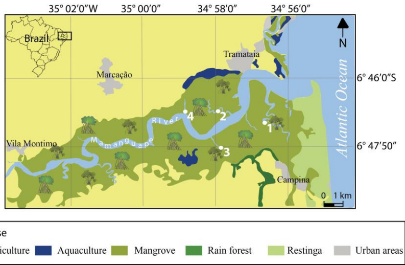
Figure 1. Map of the Mamanguape River Estuary with location of sample sites (modified from Dolbeth et al., 2016).
