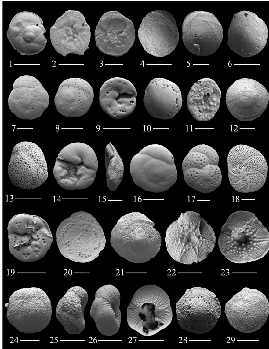
5 Figure 7. 1–3. Orbitina carinata Sellier de Civrieux, 1977; 4–6. Rotorbis auberii (d’Orbigny, 1839); 7–9. Neoconorbina sp. 1; 10–11. Neoconorbina radiatogranulata Parker, 2009; 12. Neoconorbina terquemi (Rzehak, 1888); 13–15. Rosalina bradyi (Cushman, 1915); 16. Rosalina sp. 1; 17–19. Rosalina sp. 2; 20–23. Glabratella carinata Seiglie and Bermúdez, 1965; 24–27. Glabratella mirabilis Seiglie and Bermúdez, 1965; 28–29. Glabratella carinata Seiglie and Bermúdez, 1965. Scale bar is 100 \mu\text{m} and 50 \mu\text{m} for Figs. 3-5, 7, 10-12, 14-15, 17, 20-29.
