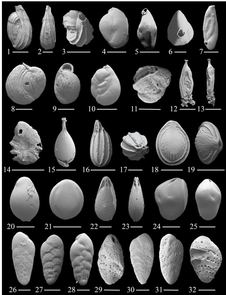
Figure 5. 1–3. Quinqueloculina cf. Q. carinatastriata Wiesner, 1923; 4–6. Quinqueloculina sp. 3; 7. Quinqueloculina cf. Q. boschiana d’Orbigny, 1839; 8–9. Miliolinella webbiana d’Orbigny, 1839; 10. Miliolinella sp. 1; 11. Hauerina atlantica Cushman, 1946; 12–13. Inaequalina sp. 1; 14. Laevipeneroplis bradyi Cushman, 1930; 15. Procerolagena oceanica (Albani, 1974); 16–17. Cushmanina bricei McCulloch, 1981; 18–19. Fissurina colomboensis McCulloch, 1977; 20. Fissurina bispinata Ujjié, 1963; 21. Fissurina sp. 2; 22–23. Fissurina semimarginata Reuss, 1870; 24–25. Fissurina? sp. 1; 26–28. Bolivina densipunctata Sellier de Civrieux, 1976; 29–32. Bolivina ordinaria Phleger and Parker, 1952. Scale bar is 100 \mu\text{m} and 50 \mu\text{m} for Figs. 2, 6–7, 17, 20, 22–25, 26, 28–32.
