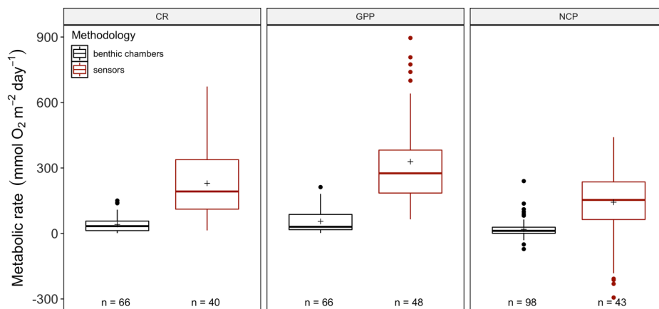
Figure 2. Comparison between benthic chamber- (black) and sensor data (red) for CR, GPP and NCP ( \text{mmol O}_2 \text{ m}^{-2} \text{ day}^{-1} ) for the full dataset. Upper and lower hinges correspond to the upper and lower quartiles, the line inside the boxes correspond to the median, the mean is marked by a crosshair and the error bars are based on minimum and maximum standard deviation for each parameter. We found differences for CR, GPP and NCP ( p<0.0.001 ).
