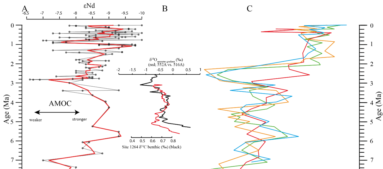
Figure 12: Comparison of seawater Neodymium isotope evolution ( \epsilon\text{Nd} ), a proxy for the strength of the AMOC, and the maximum axial length of Globorotalia menardii . (A) Dausmann et al. (2017): \epsilon\text{Nd} at Site 1088 in the southern Atlantic Ocean. The thin black line shows the original data, the red line a smoothed version, produced with the RStudios' command 'smooth.spline' at the value of 0.35. (B) AMOC strength reconstruction by Karas et al. (2017): the red line represents the \delta^{18}\text{O} seawater gradient of the Sites 552A and 516A, while the black one is the benthic \delta^{13}\text{C} curve from Site 1264. (C) Maximum axial length ( \delta Y ) versus age (Ma). The green line represents the size evolution of Hole 667A (eastern tropical Atlantic; this study), orange of Hole 925B (western tropical Atlantic; Knappertsbusch, 2016), blue of Site 502 (Caribbean Sea) and red from Site 503 (eastern tropical Pacific) (Knappertsbusch, 2007).
