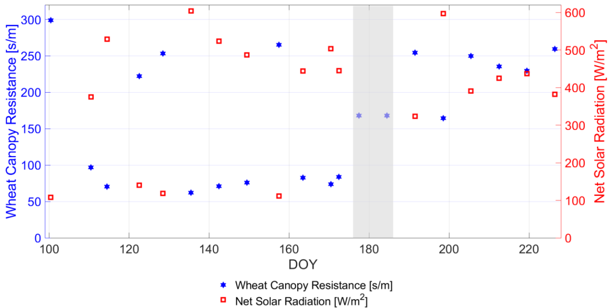
390 395 Figure 7: Comparison of the in situ measured net solar radiation [ W/m^2 ] and the calculated stomata resistance R_{ST} [ s/m ] of the winter wheat canopy from the model of Choudhury and Idso (1985) under incorporation of VWP -observations (cf. Figure 1) along days of year (DOY); The gray area indicates two dates where no net solar radiation measurement were available and the resistance values for the canopy are set to fixed values of 168 [ s/m ].
