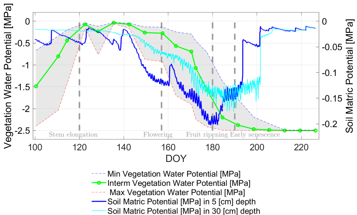
510 Figure 12: Comparison of in situ-based soil matrix (both blueish curves) and radiometer-based vegetation water (green solid and small dashed curves) potentials ( SMP [MPa] & VWP [MPa]) in the growing period of 2017 along days of year (DOY) at the winter wheat field. The gray-shaded area indicates the potential variability of the estimated VWP depending on applied relationship in (3) (cf. Fig. 3). Vertical dashed lines indicate major phenological phases of the winter wheat.
