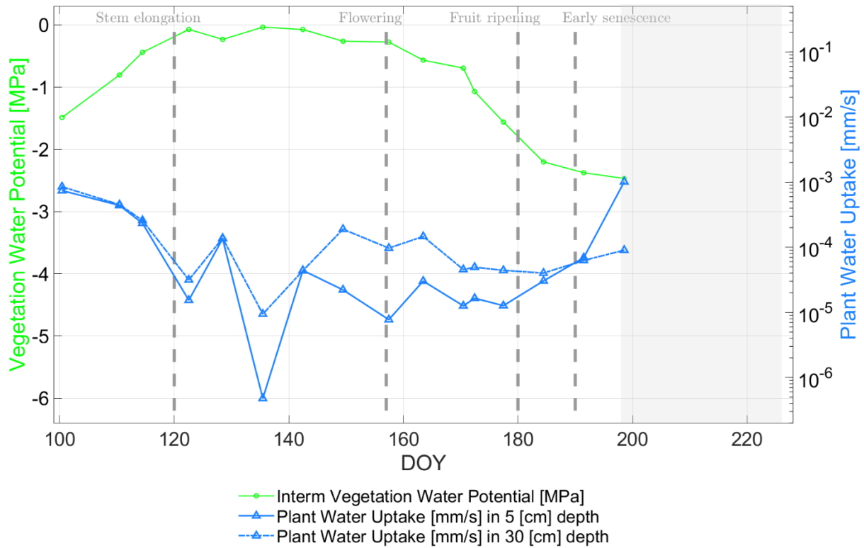
550 Figure 13: Comparison of radiometer-based plant water uptake PWU [mm/s] (blueish-colored curves with variable soil resistance at 5 [cm] and 30 [cm] soil depth) and vegetation water (green solid curve) potential VWP [MPa] along the growing season of 2017 for days of year (DOY) at the winter wheat field in Selhausen, Germany. The gray-masked area indicates the senescence phase where the water uptake estimates are not valid anymore due to simplifying assumptions in calculus of the root-xylem resistance. Vertical dashed lines indicate major phenological phases of the winter wheat.
