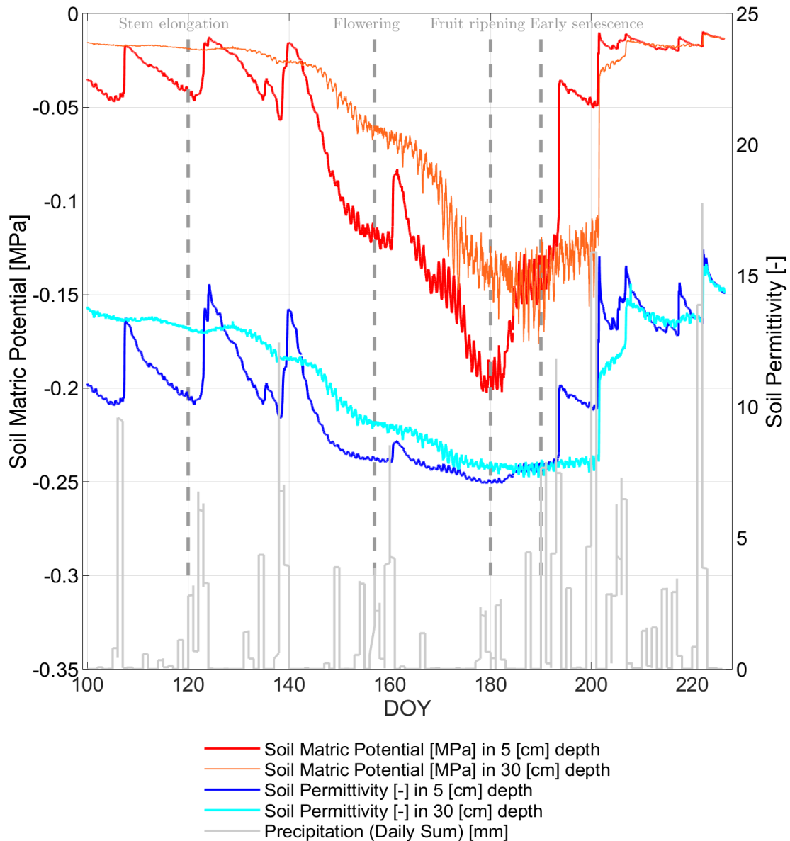
450 Figure 9: Comparison of the temporal evolution of soil matric potential ( SMP ) [ MPa ], calculated after Campbell (1974) & Clapp and Hornberger (1978) in 5 [ cm ] (red curve) and 30 [ cm ] (orange curve) soil depth from in situ measured soil permittivity [-] in 5 [ cm ] (blue curve) and 30 [ cm ] (cyan curve) throughout growing season of 2017 in days of year (DOY). Gray bars indicate the daily sum of precipitation [ mm ] at the winter wheat field in Selhausen, Germany.
