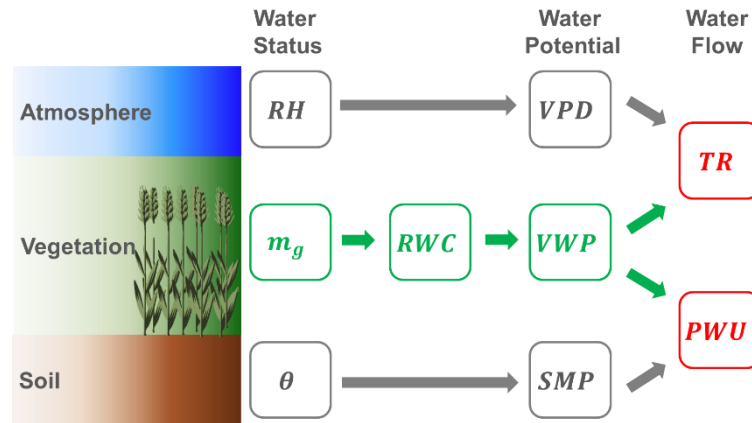
205 Figure 2: Processing workflow for estimation of soil, vegetation and atmosphere water potentials ( SMP = soil matric potential, RWC = relative water content of vegetation , VWP = vegetation water potential, VPD = vapor pressure deficit) and water fluxes ( PWU = plant water uptake, TR = transpiration rate) from storage variables ( \theta = soil moisture, m_g = vegetation water content (gravimetric), RH = relative air humidity); Green variables are derived from radiometer observations, while gray ones are calculated from in situ measurements; Red variables are derived jointly from radiometer and in situ observations.
