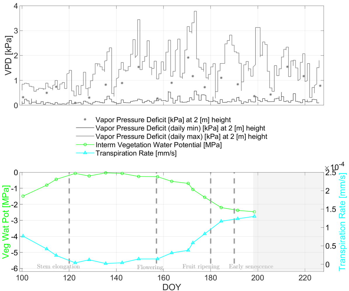
605 Figure 14: Top: Minimum and maximum of the vapor pressure deficit ( VPD ) [ kPa ] for atmospheric water need shown with gray lines. The asterisks indicate the VPD -values at time of radiometer measurement. The x-axis labels are the same as for the bottom plot.
