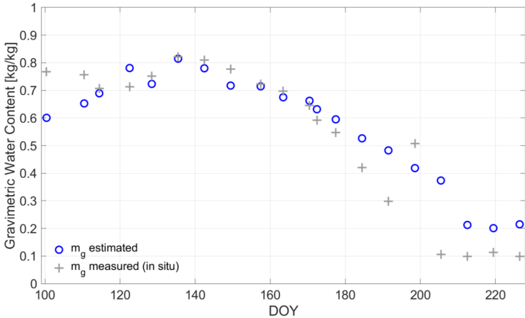
470 Figure 10: Measured (gray crosses) and radiometer-derived (blue circles) gravimetric vegetation water content ( m_g ) [kg/kg] of winter wheat along days of year (DOY) in the growing season of 2017 at the field laboratory in Selhausen, Germany (Meyer et al., 2019).
