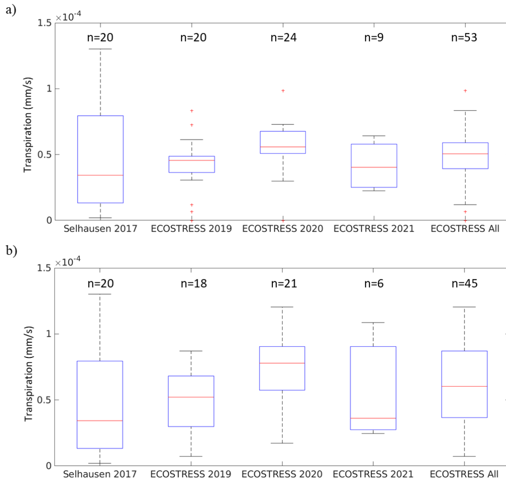
Figure 15: Boxplots of estimated transpiration rates TR [ mm/s ] comparing the field-based estimates presented for the Selhausen field-test site (see Fig. 14) and (a) the space-borne ECOSTRESS daily product and (b) the instantaneous product. The number of samples ( n ) is indicated at the top of each box. For each box, the red line shows the median, top and bottom edges are percentiles 75 and 25, respectively, top and bottom whiskers are percentiles 95 and 5, respectively, and red crosses indicate outliers.
