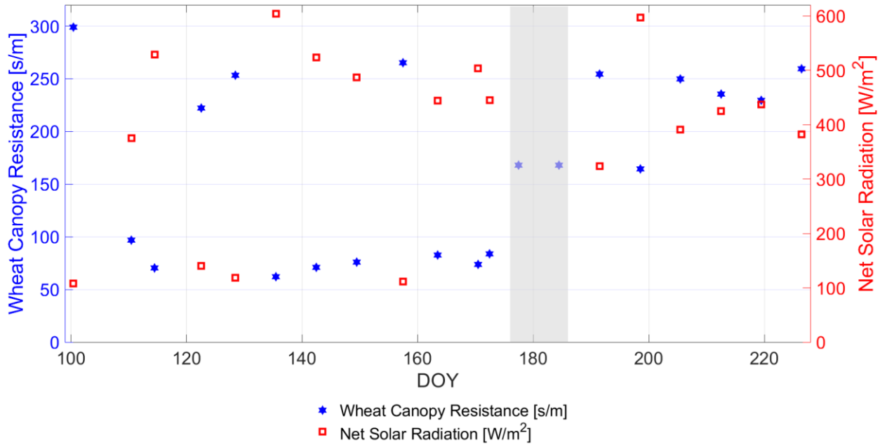
Figure 7: Comparison of the in situ measured net solar radiation [ W/m^2 ] and the calculated stomata resistance R_{ST} 385 [ s/m ] of the winter wheat canopy from the model of Choudhury and Idso (1985) under incorporation of VWP - observations (cf. Figure 1) along days of year (DOY); The gray area indicates two dates where no net solar radiation measurement were available and the resistance values for the canopy are set to fixed values of 168\ [s/m] .
