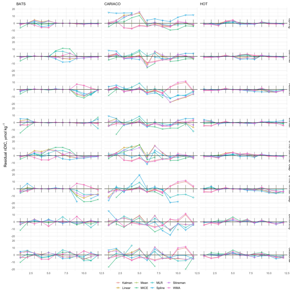
Figure 13A. Residuals between climatological monthly means calculated from observed time series and reconstructed time series of nDIC from BATS, CARIACO, and HOT. Monthly means were calculated from the time series (individual residuals shown in Figs. 10A-B) values infilled by the eight imputation models. Black sticks represent the combined uncertainty for the observations at each site.
