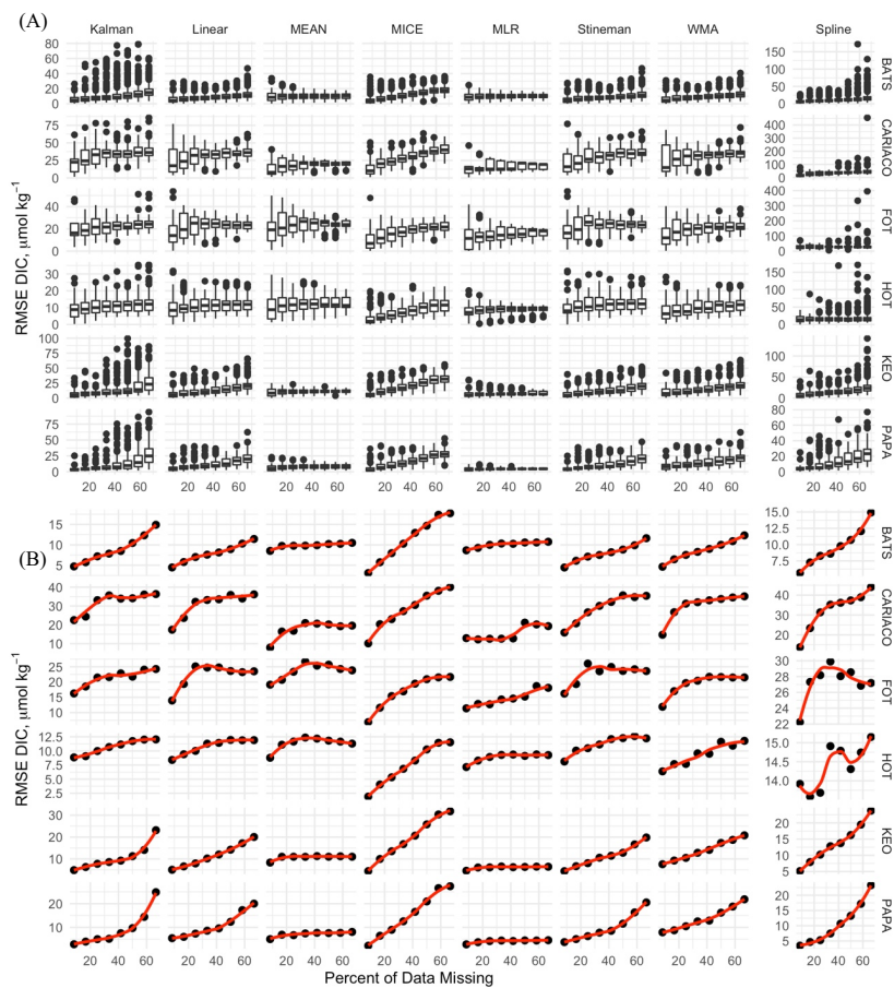
960 Figure 9. (A) Boxplots of RMSE for each gap assessment corresponding to 8.33%, 16.67%, 25%, 33.33%, 41.67%, 50%, 58.33% and 66.67% data missing rates. Box and whisker plots are composed of the median (solid line), lower and upper quartiles (box), the minimum and maximum values beyond the 25 th and 75 th quantile but < 1.5 interquartile range (whiskers) and values > 1.5 interquartile range (dots). Points above box and whiskers indicate the distribution of outliers for each model. (B) Loess fit (red line) of the median error for each gap assessment, indicating the sensitivity of the model to increasing data loss. Scales adjusted per site.
