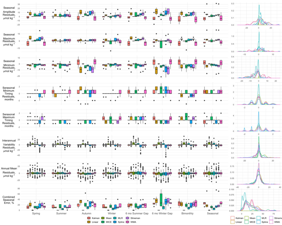
1035 Figure 14. Boxplots of the residuals between gap-filled and observed time series for: seasonal amplitude (difference between seasonal 1040 maximum and minimum); the seasonal maxima and minima, and their respective timing (the month when maxima and minima are observed); interannual variability (the standard deviation of the seasonal means); and the annual means. Combined Seasonal Error represents the combined absolute percent errors of the seasonal amplitude, maximum, minimum, and timing (see Eq.10). Box and whisker plots are composed of the median (solid line), lower and upper quartiles (box), the minimum and maximum values beyond the 25 th and 75 th quantile but < 1.5 interquartile range (whiskers) and values > 1.5 interquartile range (dots). The right-hand column shows the kernel density curves for each seasonal metric, pooled across all synthetic gap filters. Peaks in the density plots represents modes where mean errors for each model as associated with each gap filter.
