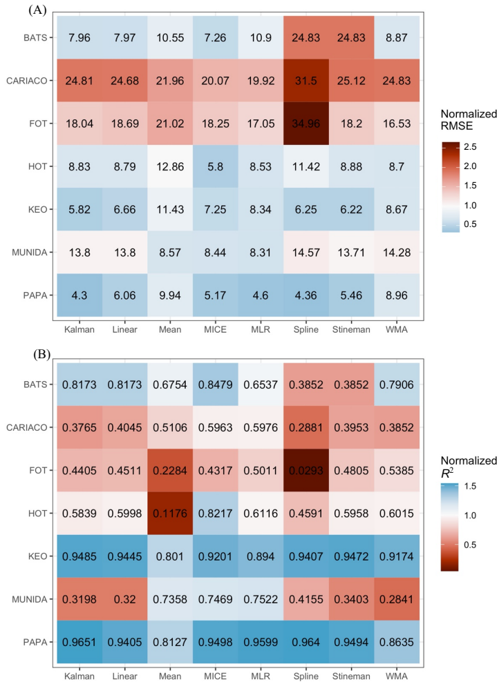
955 Figure 8. Tile plots showing (A) the RMSE (black text in tiles) for each cross validated imputation methods at each site. Tiles are colored according to RMSE normalized to the mean value across all methods and sites; and (B) the same format but for the squared correlation coefficient. Note errors at or below average performance do not equate to correlation that are average or better, e.g. Munida and HOT.
