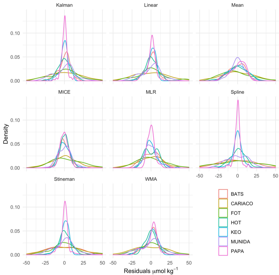
950 Figure 7. Kernel density curves of the DIC residuals between gap-filled and observed time series for each imputation model using Leave One Out Cross Validation, for all observations after Aug 1997 coinciding with availability of remotely sensed chlorophyll data. Density curves are scaled so area under the curve equals one. Plots show the probability distribution of the residuals for each model. Skewness and modalities away from 0 indicate biasing.
