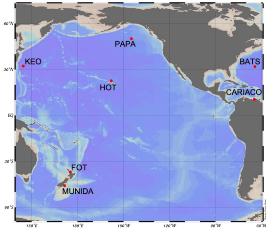
915 Figure 1. Location map of seven ocean carbon time series sites utilized for estimating DIC using an empirical multiple linear regression model and other empirical and statistical approaches for imputing carbonate time series, including Bermuda Atlantic Time-series (BATS), Carbon Retention In A Colored Ocean (CARIACO), Firth of Thames (FOT), Hawaiian Ocean Time-series (HOT), Kuroshio Extension Observatory (KEO), Munida Time-series (Munida), and Ocean Site Papa (Papa). See Table 1 for additional information about each sampling site.
