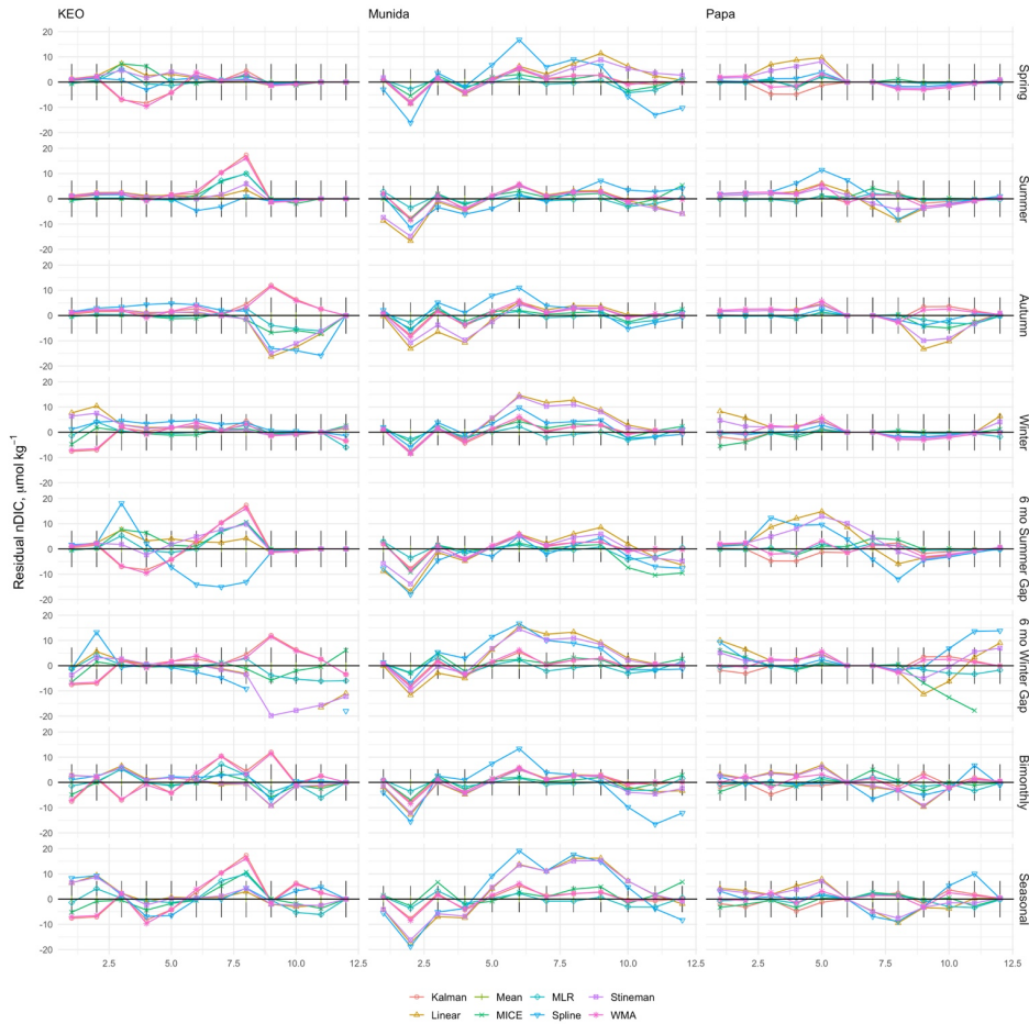
Figure 14. Residuals between climatological monthly means calculated from observed time series and reconstructed time series of nDIC from KEO, Munida, and Papa. Monthly means were calculated from the time series (individual residuals shown in Figs. 10A-B), values infilled by the eight imputation models. Black sticks represent the combined uncertainty for the observations at each site.
