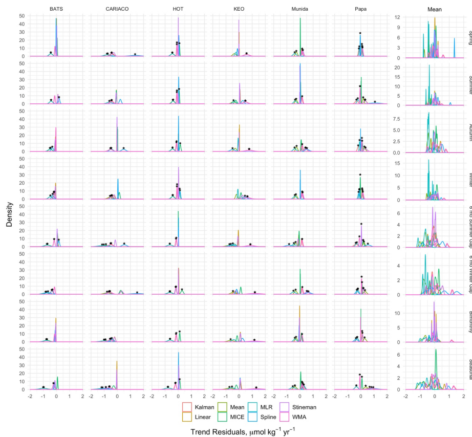
Figure 122. Kernel density curves of the nDIC residuals between the trends calculated from observed and gap-filled time series for each site and synthetic gap filter tested (see also Figs 10-11). Residuals pooled across sites are shown as the Mean column on the right-hand side. Residuals that exceeded the uncertainty bounds for the observed trend are denoted with a black asterisk. Peaks to either side of 0 indicate positive or negative biasing in the imputation method resulting in changes in the apparent trend for the reconstructed time series.
