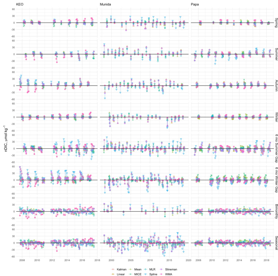
Figure 10B. Residuals between imputed and observed nDIC from KEO, Munida and Papa. Observations were selectively removed using eight gap filters: 3-month sequential seasonal filters for Spring, Summer, Autumn, and Winter; 6-month sequential gaps centered on summer and winter; and bimonthly (odd months) and seasonal (1 max, 1 min, and 2 transition samples) sampling regimes and gaps were filled using Kalman filter with a state space model, linear interpolation, mean imputation, empirical multiple linear regression (MLR), multiple imputation by chained equations (MICE), spline interpolation, Stineman interpolation and exponential weighted moving average (WMA).
