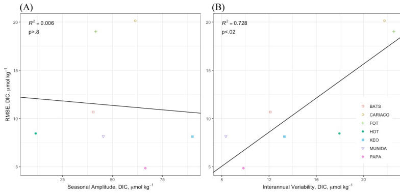
Figure 5. Correlations between RMSE and (A) seasonal amplitude and (B) interannual variability across sites
