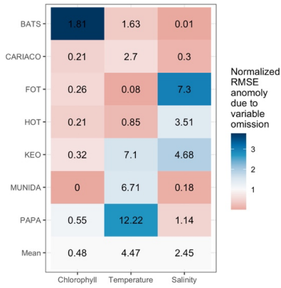
945 Figure 6. Tile plot showing the change in RMSE per site due to the selective omission of input variables and refitting of the MLR. Tiles are colored to normalized error anomalies for visualization of relative differences, while RMSE anomalies are given in each tile for the effect of omitting the predictor variable at each site.
