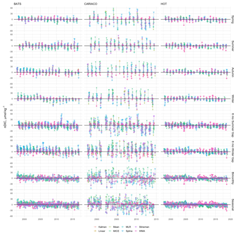
Figure 10A. Residuals between imputed and observed nDIC from BATS, CARIACO and HOT. Observations were selectively removed using eight gap filters: 3-month sequential seasonal filters for Spring, Summer, Autumn, and Winter; 6-month sequential gaps centered on summer and winter; and bimonthly (odd months) and seasonal (1 max, 1 min, and 2 transition samples) sampling regimes and gaps were filled using Kalman filter with a state space model, linear interpolation, mean imputation, empirical multiple linear regression (MLR), multiple imputation by chained equations (MICE), spline interpolation, Stineman interpolation and exponential weighted moving average (WMA).
