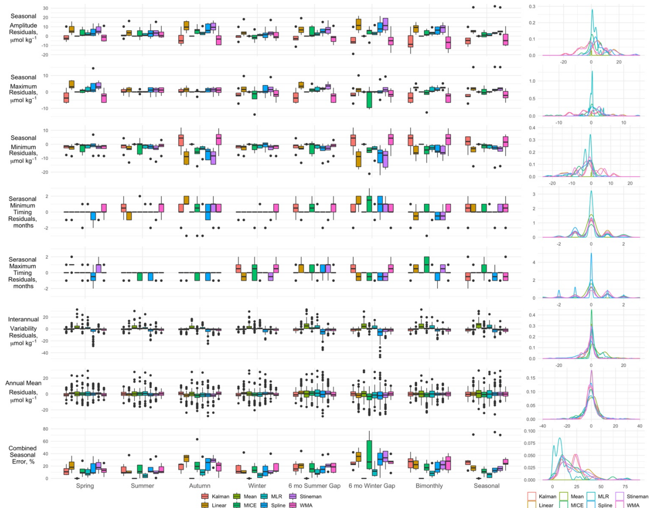
940 Figure 14. Boxplots of the residuals between gap-filled and observed time series for: seasonal amplitude (difference between seasonal maximum and minimum); the seasonal maxima and minima, and their respective timing (the month when maxima and minima are observed); interannual variability (the standard deviation of monthly means); and the annual means. Combined Seasonal Error represents the combined absolute percent errors of the seasonal amplitude, maximum, minimum, and timing (see Eq.10). Box and whisker plots are composed of the median (solid line), lower and upper quartiles (box), the minimum and maximum values beyond the 25 th and 75 th quantile but < 1.5 interquartile range (whiskers) and values > 1.5 interquartile range (dots). The right-hand column shows the kernel density curves for each seasonal metric, pooled across all synthetic gap filters. Peaks in the density plots represents modes where mean errors for each model as associated with each gap filter.
