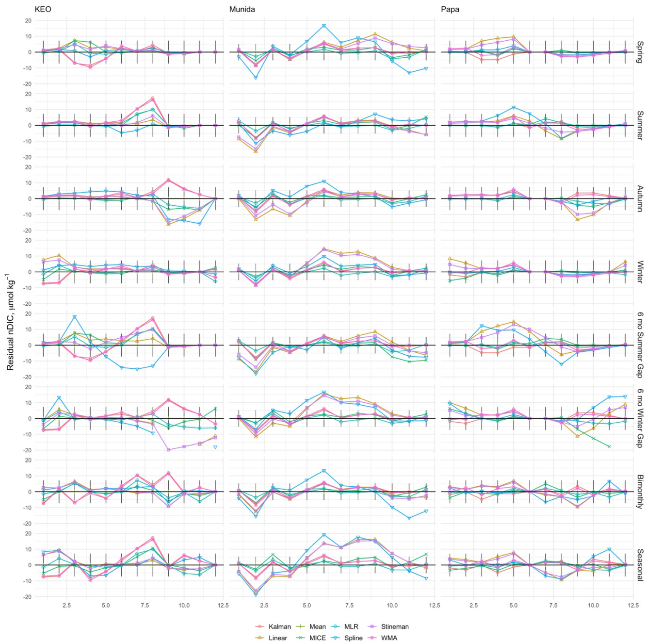
935 Figure 14. Residuals between climatological monthly means calculated from observed time series and reconstructed time series of nDIC from KEO, Munida, and Papa. Monthly means were calculated from the time series (individual residuals shown in Figs. 10A-B) values infilled by the eight imputation models. Black sticks represent the combined uncertainty for the observations at each site.
