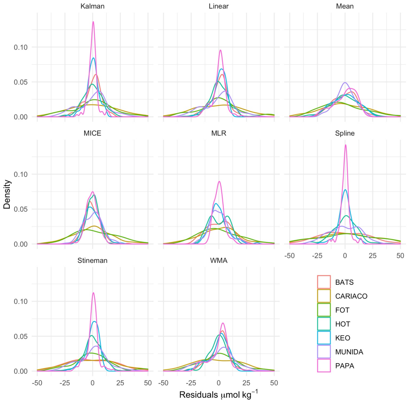
885 Figure 7. Kernel density curves of the DIC residuals between gap-filled and observed time series for each imputation model using Leave One Out Cross Validation, for all observations after Aug 1997 coinciding with availability of remotely sensed chlorophyll data. Density curves are scaled so area under the curve equals one. Plots show the probability distribution of the residuals for each model. Skewness and modalities away from 0 indicate biasing.
