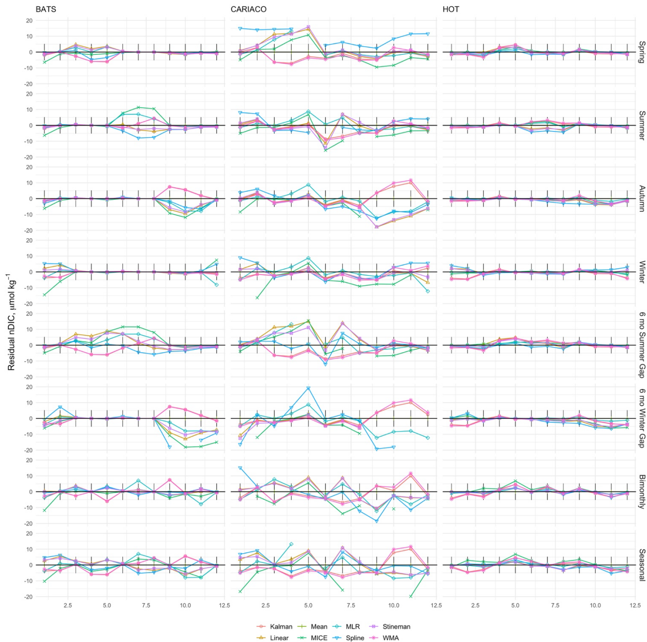
930 Figure 13A. Residuals between climatological monthly means calculated from observed time series and reconstructed time series of nDIC from BATS, CARIACO, and HOT. Monthly means were calculated from the time series (individual residuals shown in Figs. 10A-B) values infilled by the eight imputation models. Black sticks represent the combined uncertainty for the observations at each site.
