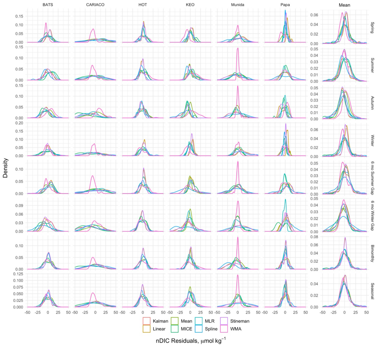
Figure 11. Kernel density curves of the nDIC residuals between gap-filled and observed values for each site and synthetic gap filter tested (see also Fig. 10). Residuals pooled across sites are shown as the Mean column on the right-hand side. Density curves are scaled so area under the curve equals one. Plots show the probability distribution of the residuals. Skewness and modalities away from 0 indicate biasing.
