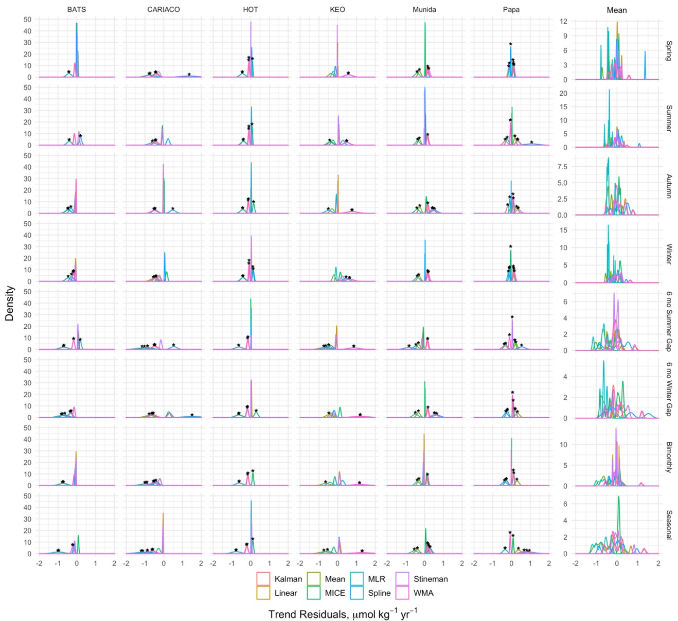
925 Figure 12. Kernel density curves of the nDIC residuals between the trends calculated from observed and gap-filled time series for each site and synthetic gap filter tested (see also Figs 10-11). Residuals pooled across sites are shown as the Mean column on the right-hand side. Residuals that exceeded the uncertainty bounds for the observed trend are denoted with a black asterisk. Peaks to either side of 0 indicate positive or negative biasing in the imputation method resulting in changes in the apparent trend for the reconstructed time series.
