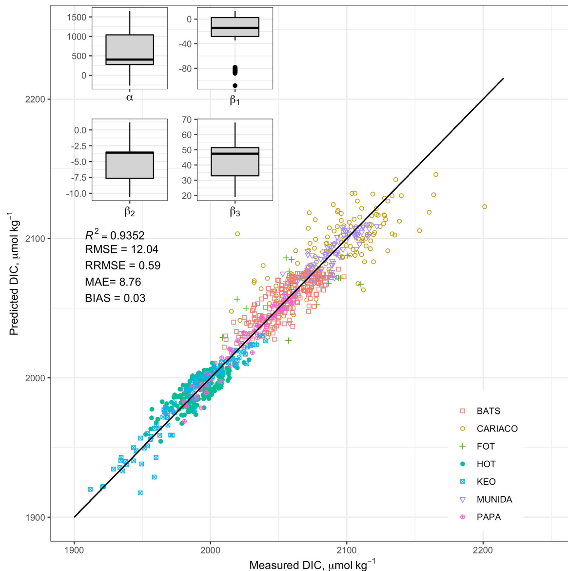
870 Figure 4. Composite of predicted and measured DIC using a multiple linear regression model based on measured temperature, salinity and remotely sensed chlorophyll pooled from test sites: Bermuda Atlantic Time-series Study (BATS); Carbon Retention In A Colored Ocean (CARIACO); Firth of Thames (FOT); Hawaiian Ocean Time-series (HOT); Kuroshio Extension Observatory (KEO); Munida Time-series (Munida); Ocean Site Papa (Papa). Box and whisker plots for predictor variable coefficients \alpha , \beta_1 , \beta_2 and \beta_3 are composed of the median (solid line), lower and upper quartiles (box), the minimum and maximum values beyond the 25 th and 75 th quantile but < 1.5 interquartile range (whiskers) and values > 1.5 interquartile range (dots). 875
