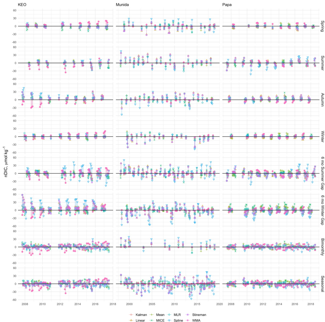
910 Figure 10B. Residuals between imputed and observed nDIC from KEO, Munida and Papa. Observations were selectively removed using eight gap filters: 3-month sequential seasonal filters for Spring, Summer, Autumn, and Winter; 6-month sequential gaps centered on summer and winter; and bimonthly (odd months) and seasonal (1 max, 1 min. and 2 transition samples) sampling regimes and gaps were filled using Kalman filter with a state space model, linear interpolation, mean imputation, empirical multiple 915 linear regression (MLR), multiple imputation by chained equations (MICE), spline interpolation, Stineman interpolation and exponential weighted moving average (WMA).
