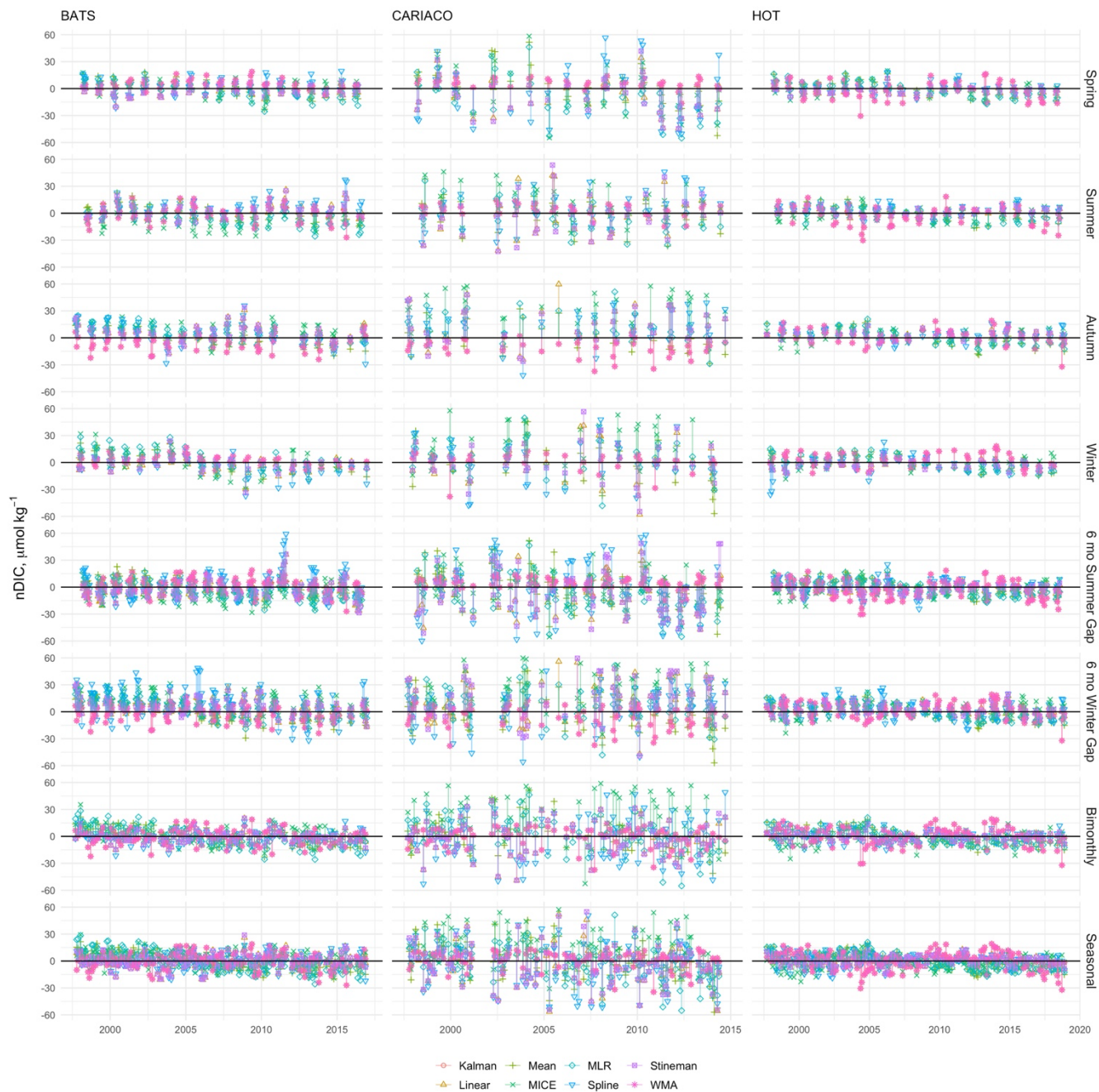
905 Figure 10A. Residuals between imputed and observed nDIC from BATS, CARIACO and HOT. Observations were selectively removed using eight gap filters: 3-month sequential seasonal filters for Spring, Summer, Autumn, and Winter; 6-month sequential gaps centered on summer and winter; and bimonthly (odd months) and seasonal (1 max, 1 min. and 2 transition samples) sampling regimes and gaps were filled using Kalman filter with a state space model, linear interpolation, mean imputation, empirical multiple linear regression (MLR), multiple imputation by chained equations (MICE), spline interpolation, Stineman interpolation and exponential weighted moving average (WMA).
