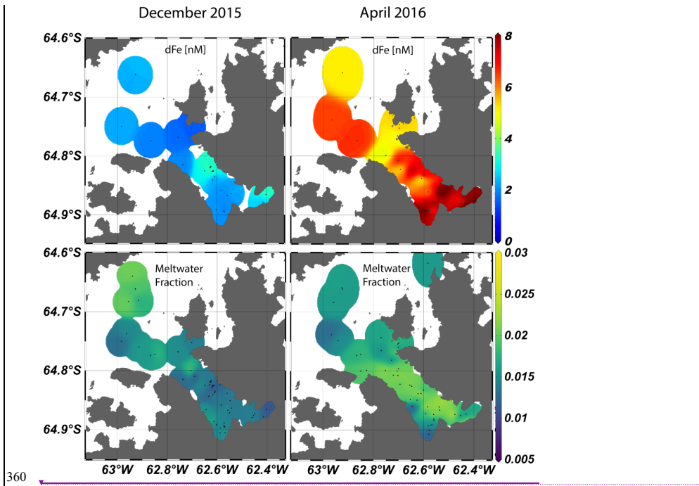
Figure 3. Surface (<20m) dissolved Fe (top) and meltwater fraction (bottom) for late Spring (left two panels) and Fall (right two panels). Plots were made with Ocean Data View visualization software (Schlitzer, 2002, Ocean Data View, last access: 1 February 2021).
