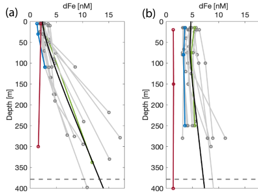
365 Figure 4. Depth profiles of dissolved Fe [nM] sampled in the Andvord Bay region for December 2015 (A) and April 2016 (B). The colored lines indicate highlighted profiles: the geometric mean of the linearly interpolated data points within Andvord Bay (black), Station B on the continental shelf (red, see Fig. 1), Station GS (Gerlache Strait, blue) and Station S3 (green). Other Andvord Bay stations are shown in grey. The dashed line is the average bottom depth within the fjord.
