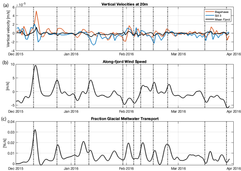
910 Figure 9. (a) Modeled vertical velocities at 20 m for the following locations: Bagshawe Glacier (IBA), Sill 3 and the fjord region 915 average. 24 hr gaussian filter applied to time series of along-fjord wind velocity (b) and relative meltwater export out of the fjord (c). Wind events exceeding an absolute velocity of 8 \text{ m s}^{-1} are indicated by vertical dashed lines. Wind speed data is based on bias- corrected RACMO model output for the center of the fjord, used to force the ROMS model. The transport of meltwater dye is shown relative to the total amount of meltwater dye within Andvord Bay to focus on the physical dynamics and not the changes in volume of dye present in the fjord.
