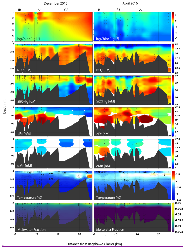
305 Figure 2. Seasonal phytoplankton, macro-, micronutrient, temperature, and meltwater distributions plotted as sections extending from the inner basin (IB, left) towards Gerlache Strait (GS, right). Plots were made with Ocean Data View visualization software (Schlitzer, 2002, Ocean Data View, last access: 1 February 2021).
