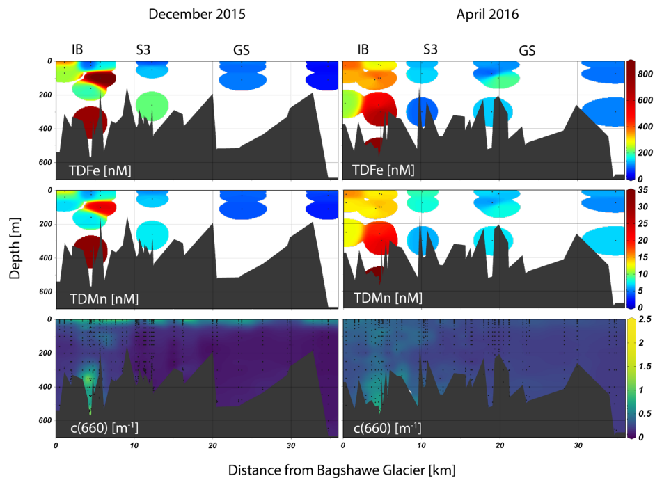
400 Figure 6. Total dissolvable trace metals and beam attenuation coefficient c(660) for both seasons. The transects are plotted as distance from the Bagshawe Glacier terminus. Plots were made with Ocean Data View visualization software (Schlitzer, 2002, Ocean Data View, last access: 1 February 2021).
