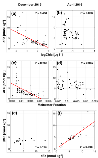
Figure 5. Dissolved trace metals plotted against observed and derived variables for December 2015 (a, c, e) and April 2016 (b, d, f). Dissolved Fe (a-b) versus logChlorophyll-a concentrations. Dissolved Fe (c-d) versus meltwater fraction. Dissolved Mn (e-f) versus dissolved Fe. Least-squares regression lines are shown where they are statistically significant ( p < 0.005 ).
