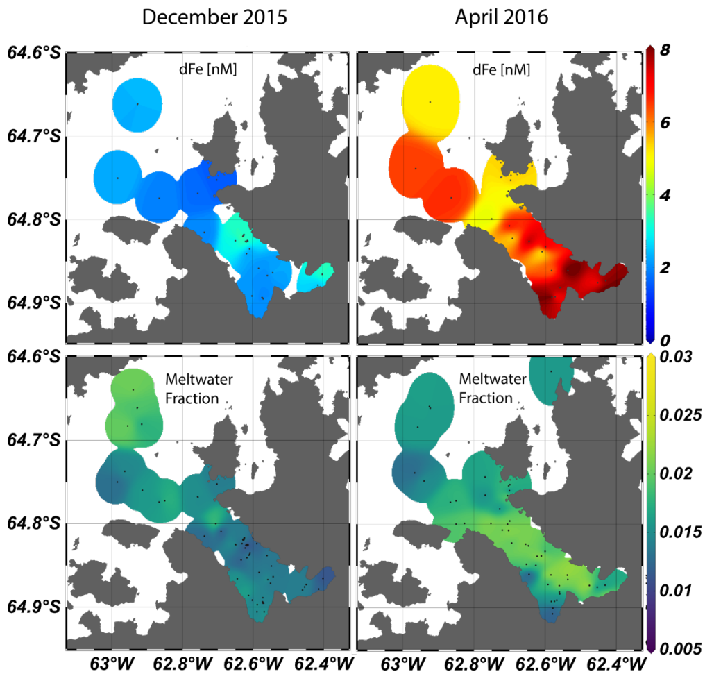
Figure 3. Surface (<20m) dissolved Fe (top) and meltwater fraction (bottom) for late Spring (left two panels) and Fall (right two panels). Plots were made with Ocean Data View visualization software (Schlitzer, 2002, Ocean Data View, last access: 1 February 2021).
