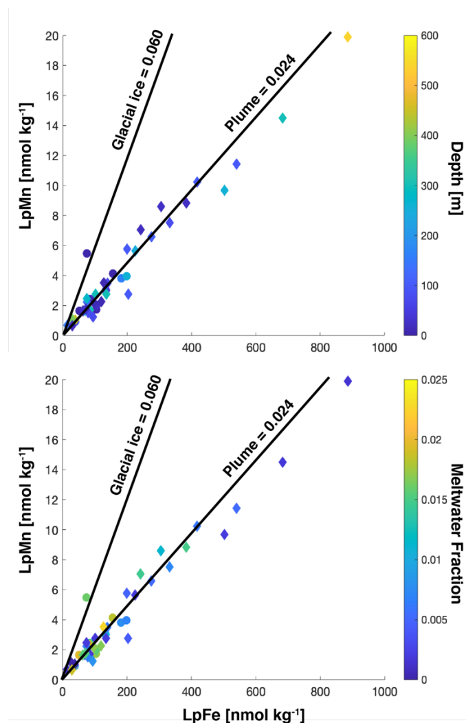
610 Figure 8. Labile particulate Fe and Mn plotted for water column samples. The colorbar shows the influence of depth (top panel) or meltwater fraction (bottom panel). For both panels, December 2015 cruise is indicated by filled circles and the April 2016 cruise is indicated by filled diamonds. The lines indicate the average ratio of Mn:Fe determined from candidate sources.
