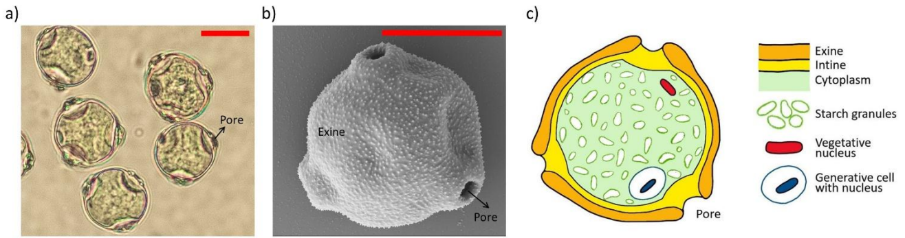
700 Figure 1: Different views of birch pollen grains. a) Light microscope image of pollen grains in water. b) Electron microscope image of a single pollen grain. c) Schematic sectional view with the main components of a birch pollen grain. Red scale bar is 10 \mu\text{m} .
