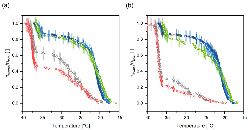
Figure 8. Results of the unfolding experiment and enzymatic digestion of extracted INMs (sample B) at 37 °C using subtilisin A (from Bacillus licheniformis ) and urea after (a) 1 h and (b) 6 h incubation time. Filled, blue squares correspond to sample B in Tris buffer at room temperature prior to treatment and hollow, blue squares to the control sample. Green circles show the treatment with subtilisin A, grey triangles (cone up) with urea and red triangles (cone down) represent the treatment using a mixture of subtilisin A and urea. Vertical lines represent the counting error.
