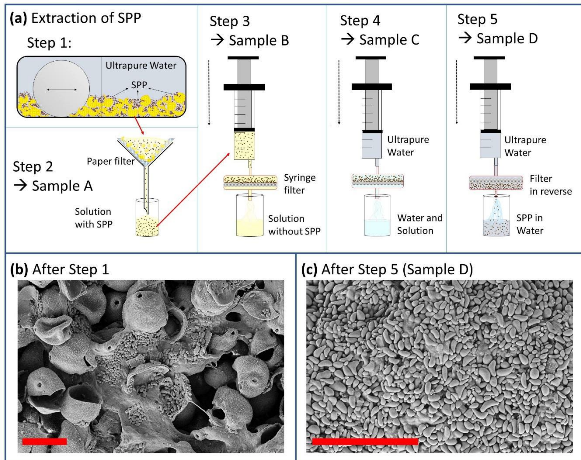
710 Figure 2: a) Extraction process of SPP. Step 1: Entire pollen grains mixed with ultrapure water are crushed in a mixer mill (MM400, Retsch GmbH, Haan, GER). Step 2: The sample is filtered so that entire pollen grains and large outer shells are excluded. Step 3: Filtration with a 0.2 \mu\text{m} pore sized filter. Step 4: The filter including the SPP is rinsed with ultrapure water to wash off soluble material. Step 5: The filter is reversed and the SPP are extracted with ultrapure water. b) Crushed pollen grains, cytoplasmic material and SPP (starch granules) after step 1. c) Extracted SPP after step 5. Red scale bar = 20 \mu\text{m} .
