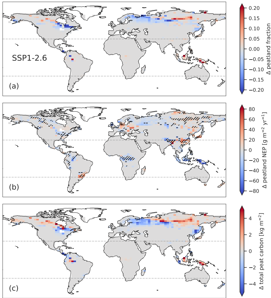
Figure 7. Simulated median anomalies under the SSP1-2.6 scenario in the year 2300 in (a) peatland area fraction, (b) peatland NEP, and (c) total peat carbon as defined in section 2.2. Anomalies are calculated between 20-year averages spanning 1995-2014 and 2291-2310. Gridcells where NEP becomes negative are marked with a minus. Hatched areas in (b) indicate a positive area anomaly, which in the model can lead to an increase in NEP through the dilution of soil carbon and a corresponding reduction in soil carbon respiration per area
