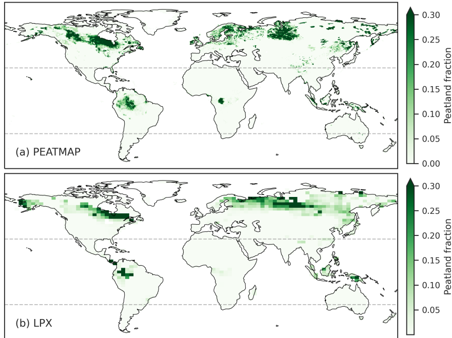
Figure 3. Global peatland area fraction as (a) estimated by PEATMAP (Xu et al., 2018b), shown here in a 0.5^\circ \times 0.5^\circ gridded version and (b) simulated by LPX in the year 1975 after a transient simulation from the Last Glacial Maximum
