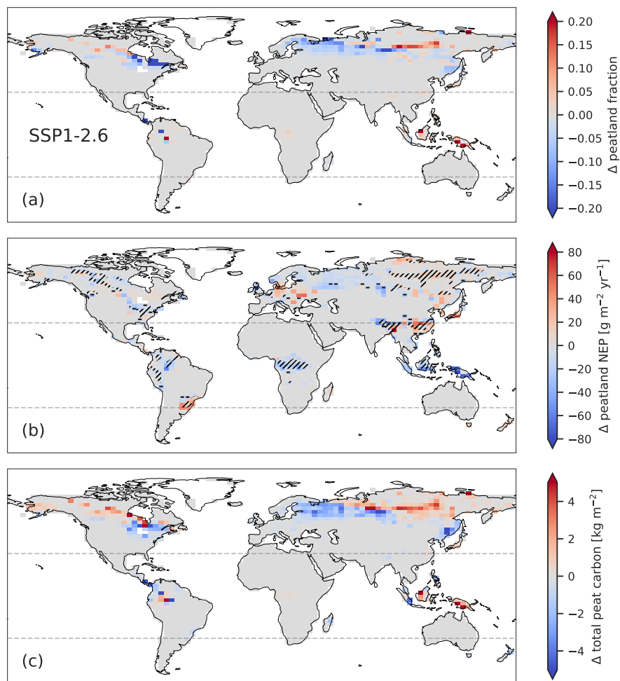
Figure 7. Simulated median anomalies under the SSP1-2.6 scenario at the year 2300 in (a) peatland area fraction, (b) peatland NEP, and (c) total peat carbon as defined in section 2.2. Anomalies are calculated between 20 year averages spanning 1995-2014 and 2291-2310. Gridcells where NEP becomes negative are marked with a minus. Hatched areas in (b) indicate a positive area anomaly, which in the model can lead to an increase in NEP through the dilution of soil carbon and a corresponding reduction in soil carbon respiration per area
