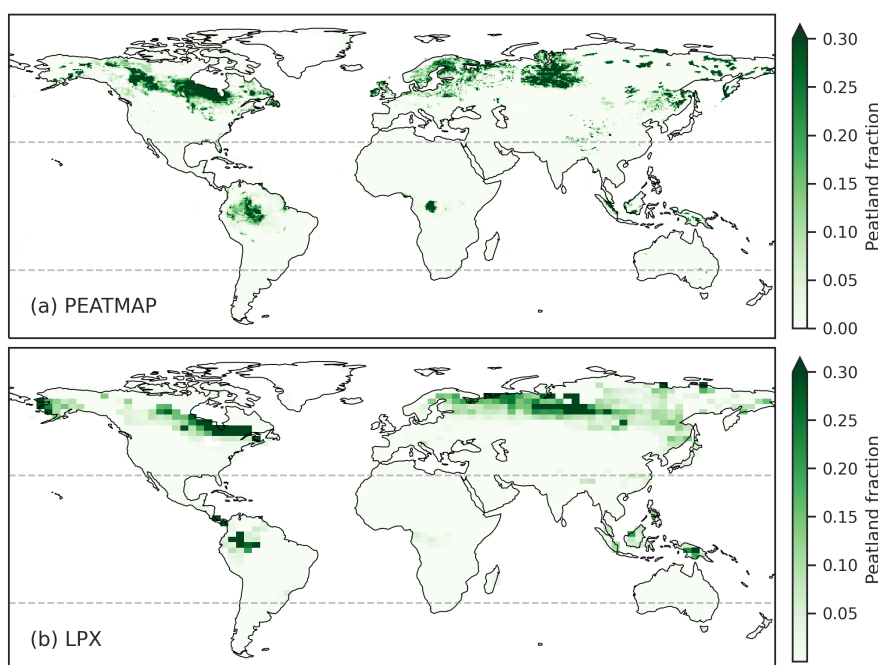
Figure 3. Global peatland area fraction as (a) estimated by PEATMAP (Xu et al., 2018b), shown here in a 0.5° × 0.5° gridded version and (b) simulated by LPX at the year 1975 after a transient simulation from the Last Glacial Maximum
