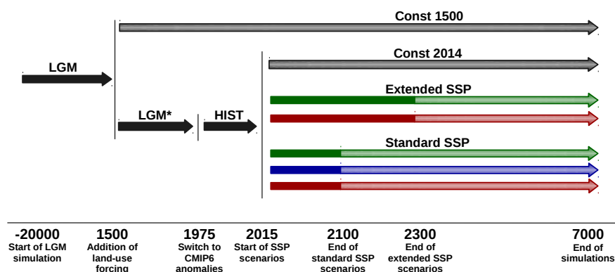
Figure 1. Diagramm of the simulation setup. A transient simulation from the LGM to 1975 and with additional land-use forcing after 1500 (LGM*) is followed by short historical simulations until 2014 (HIST) and subsequent standard and extended SSP scenario simulations forced by CMIP6 climate anomalies. After the end of the transient forcing (full arrows), SSP scenarios are continued with constant forcing (transparent arrows). Additional commitment simulations with constant boundary conditions start at 1500 and 2014
