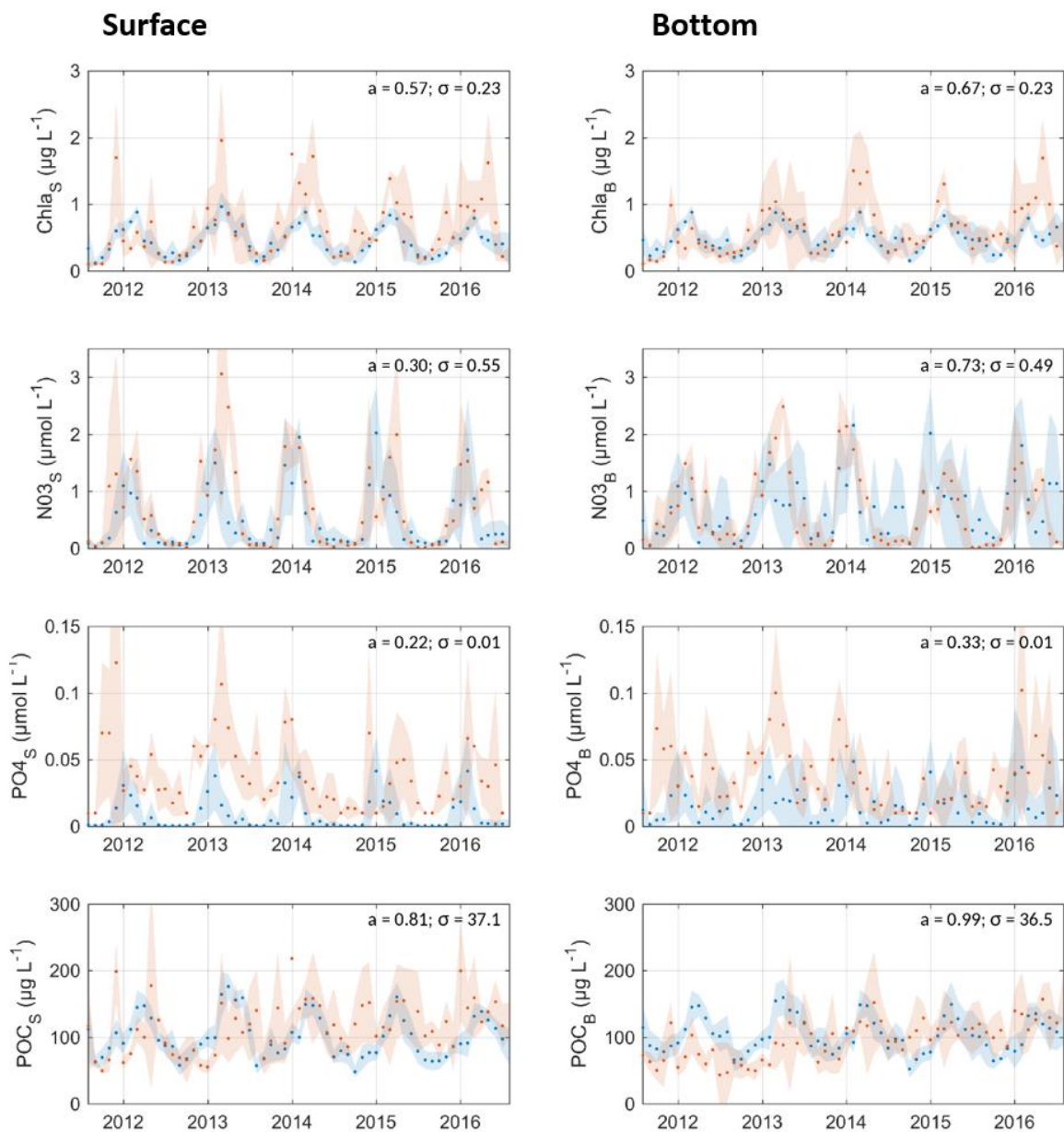
Figure 3: Comparison of monthly averaged simulated (blue) and measured (orange - SOMLIT Banyuls station) concentration of (from top to bottom) Chl- a ( \mu\text{g Chl-}a \text{ L}^{-1} ), NO 3 ( \mu\text{mol N L}^{-1} ), PO 4 ( \mu\text{mol P L}^{-1} ), and POC ( \mu\text{g C L}^{-1} ) from the surface (left) and bottom (right) waters. Standard deviations are shown by shaded areas. The slope of the linear relation model to observation (a) and the mean standard deviation ( \sigma ) are specified. Note that here the bacteria and mesozooplankton concentrations are excluded from the POC calculation to fit with the measurement method.
