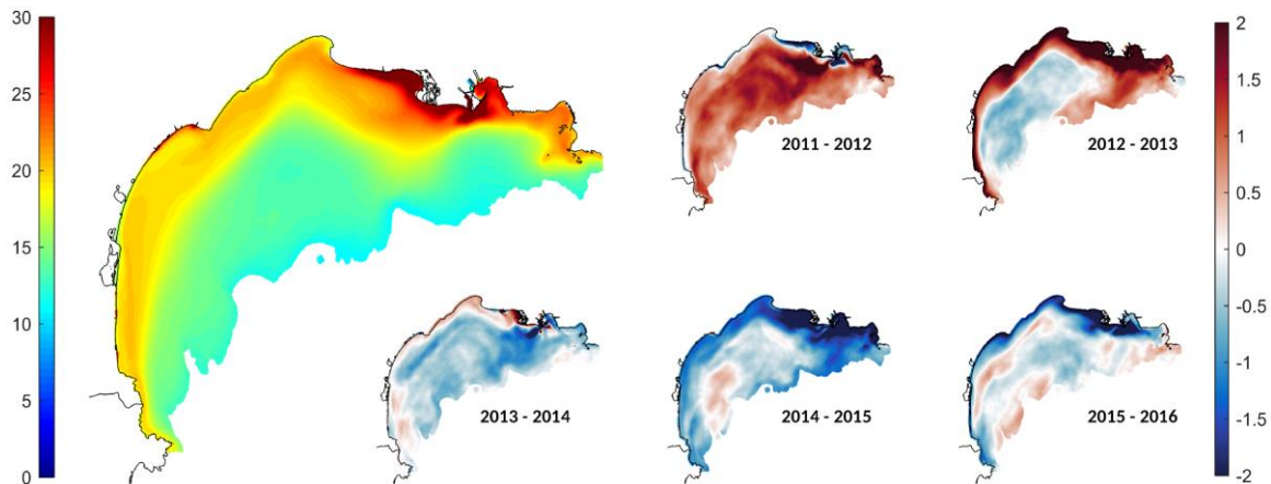
435 Figure 12: Left: Mean POC deposition over the shelf (in \text{g C m}^{-2} \text{ yr}^{-1} ) for the 2011-2016 period. Right: Annual anomalies in the POC deposition (in \text{g C m}^{-2} \text{ yr}^{-1} ).
