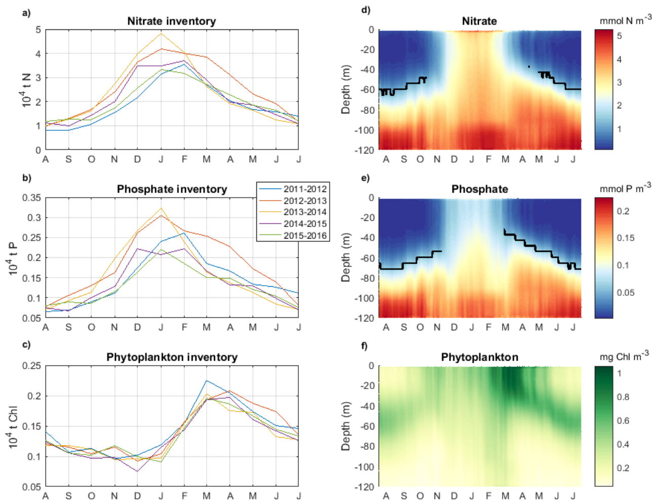
Figure 9: Time series for the five simulated years of depth-integrated monthly averaged inventory of a) nitrate ( 10^4 t N), b) phosphate ( 10^4 t P), c) chlorophyll- a ( 10^4 t Chl- a ), and for climatological vertical section of daily concentrations of d) nitrate ( \text{mmol N m}^{-3} ), e) phosphate ( \text{mmol P m}^{-3} ) and f) chlorophyll- a ( \text{mg Chl-}a \text{ m}^{-3} ). Black lines on panels E and F represent nutriclines ( 1 \text{ mmol N m}^{-3} and 0.05 \text{ mmol P m}^{-3} ).
