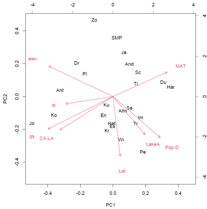
1075 Figure 2: Correlation matrix PCA biplot illustrating the spatial association of lake properties in the data set. For site abbreviations see Fig. 1 caption
