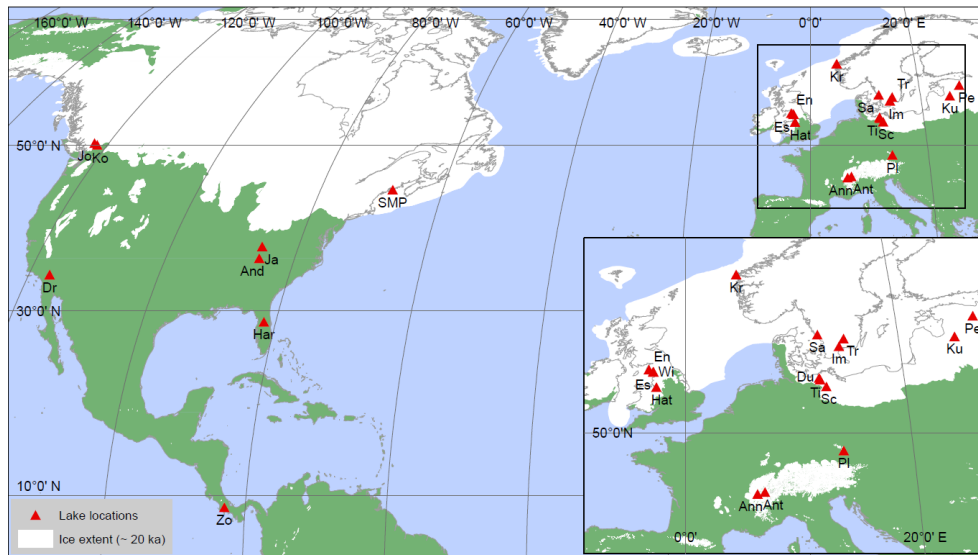
1070 Figure 1: Spatial distribution of the 24 lake sites: Lac D’Anney (Ann), Plesne Lake (Pl), Hatchmere, (Hat), Peipsi (Pe), Sargent Mountain Pond (SMP), Dudinghauser (Du), Schulzensee (Sc), Tiefer (Ti), Lac D’Anterne (Ant), Lake Harris (Har), Jackson Pond (Ja), Anderson Pond (And), Dry Lake (Dr), Kokwaskey Lake (Ko), Windermere (Wi), Ennerdale (En), Esthwaite (Es), Kråkenesvatn (Kr), Laguna Zoncho (Zo), Lower Joffre Lake (Jo), Sämbošjön (Sa), Trummen (Tr), Immeln (Im), Kūzi (Ku)
