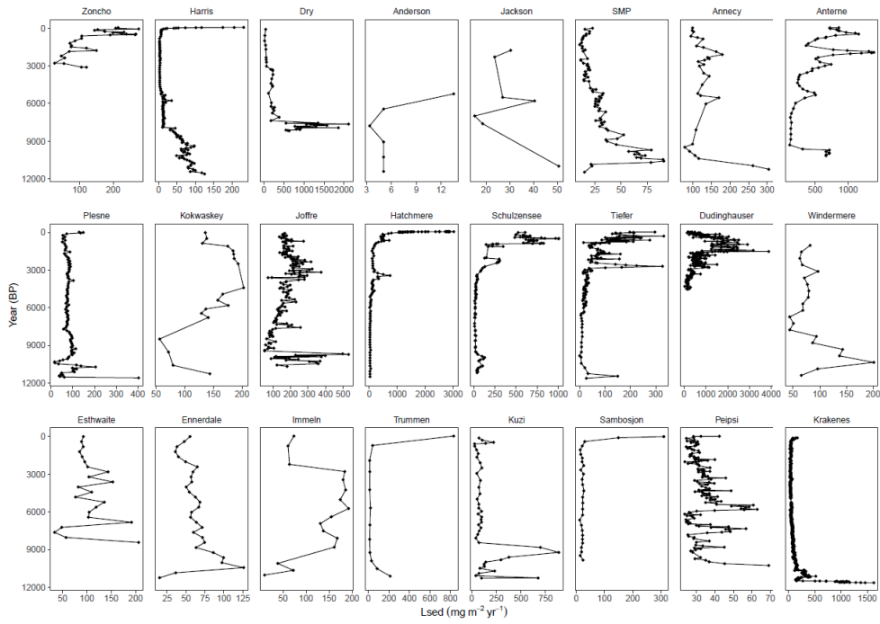
1080 Figure 4: The sediment inferred lake-wide sediment P loading ( L_{sed} ) records for all 24 lakes
