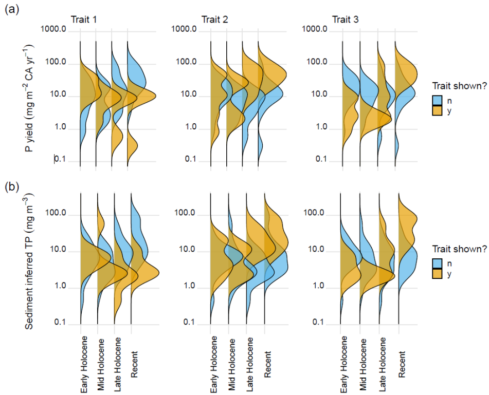
1100 Figure 10: Density distribution curves of (a) sediment mean P yield and (b) sediment inferred mean lake water TP showing changes in the three traits throughout the Holocene. Note Dudinghauser was removed for this analysis (see Sect. 3)
