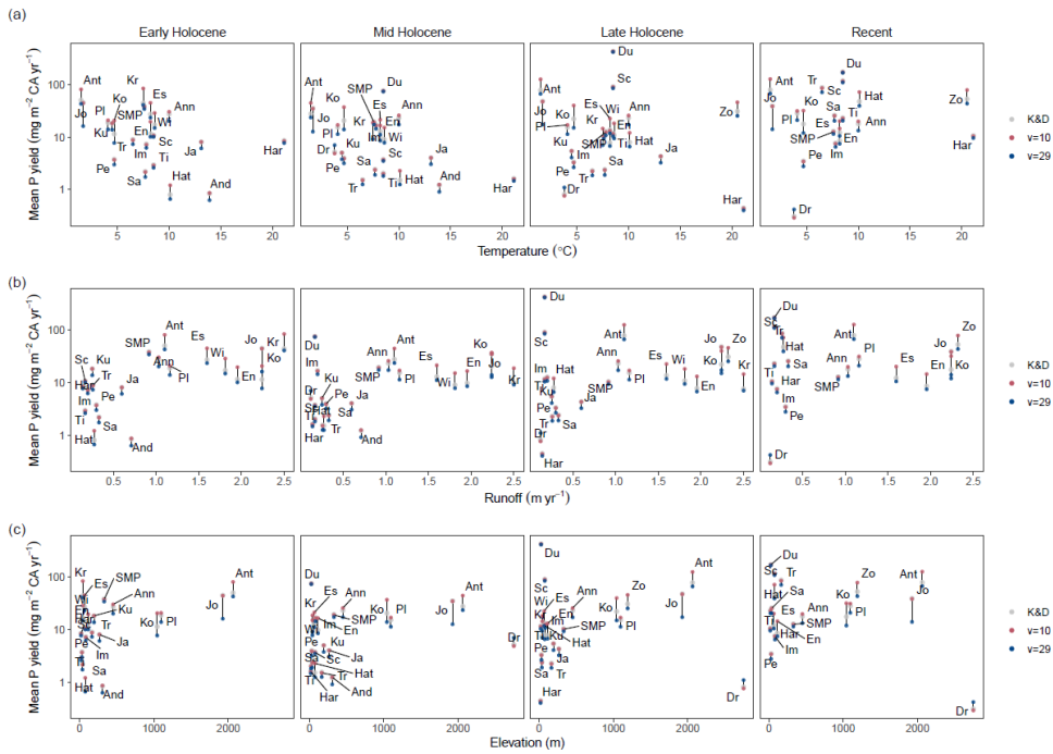
Figure 9: Association of mean sediment inferred P yield for each site with (a) modern mean annual temperature, (b) modern mean annual runoff , and (c) lake elevation for the four Holocene time intervals. Mean sediment inferred P yield is estimated using three values of R_p . For site abbreviations see Fig. 1 caption and for correlations see Tables 1 and 2
