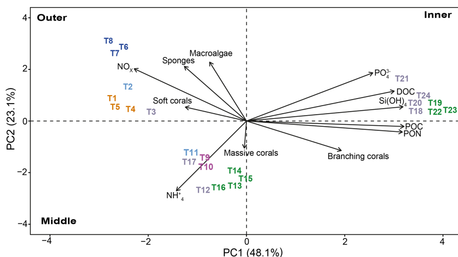
Figure 11. Principal component analysis (PCA) between benthic community (macroalgae, sponges, corals, branching corals, and massive corals) data and environmental parameters (PON, POC, DOC, \text{Si(OH)}_4 , \text{PO}_4^{3-} , \text{NO}_x , and \text{NH}_4^+ ) measured for each transect ( n = 24 ). The length of the vectors indicates the contribution of each parameter. The first dimension explains 48.1 % of the variance, and the second dimension explains 23.1 % of the variance. Colors refer to the cluster subdivision (Fig. 10).
