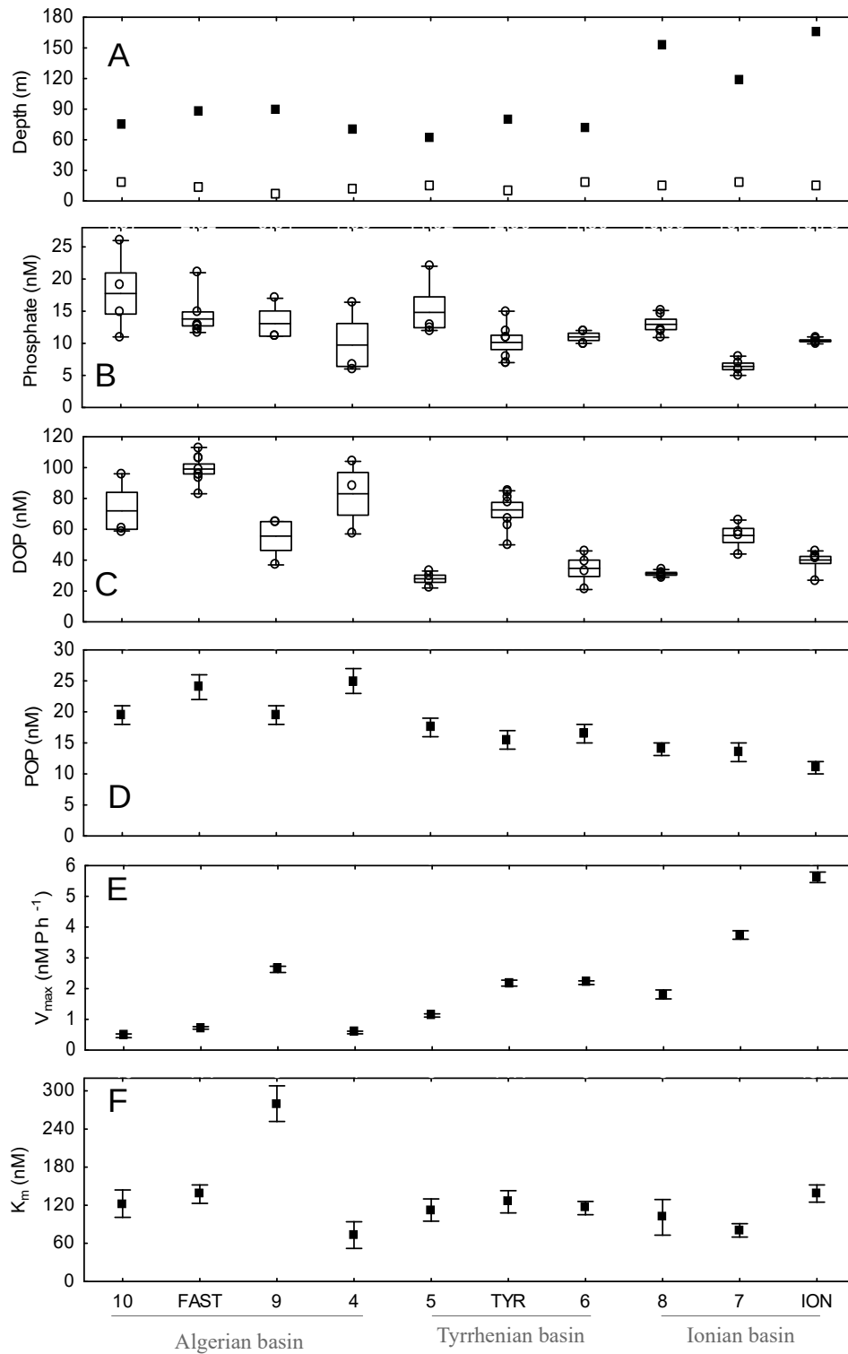
Figure 2. Depth of the mixed layer (empty symbols) and the phosphocline (filled symbols, see section 2.5 for details on the calculations) across the transect (panel A). Longitudinal variability inside the phosphate depleted layer of phosphate concentration (panel B), DOP concentration (panel C), particulate organic phosphorus (panel D), and AP Michaelis Menten parameters, V_{max} and K_m (panels E and F). Phosphate and DOP data are represented as box plots (average, standard error and min-max values inside the PDL) as well as raw data (empty symbols). For POP, V_{max} and K_m , data shown were measured at 5 m depth and error bars correspond to measurement precision (POP) and fitting model standard errors ( V_{max} and K_m ).
