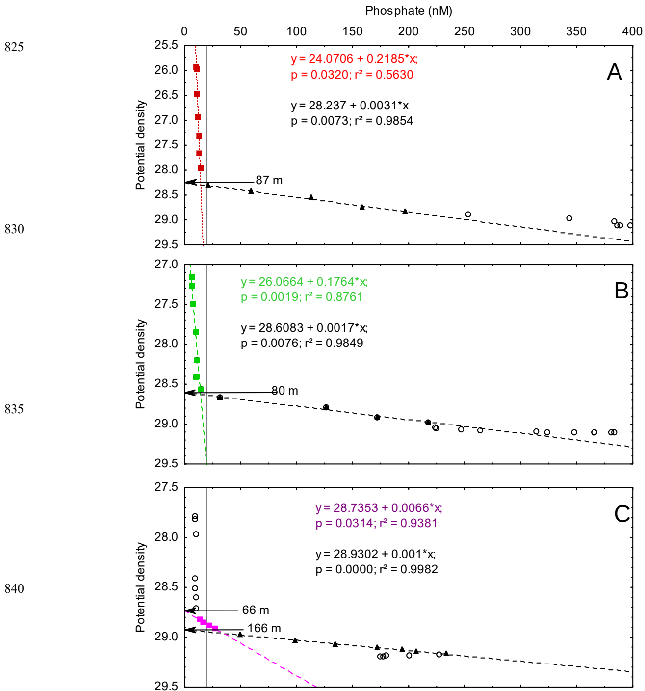
845 Figure 3. Diagrams of phosphate concentration versus density at FAST (panel A), TYR (panel B) and ION (panel C) from the surface to the bottom and linear regressions between phosphate concentration and density through the phosphacline (black symbols) and inside the PDL (colored symbols). Results of the regression analyses can be found in Table 2 and plots from short stations can be found in Supplementary Fig S1. Vertical grey lines (phosphate concentration = 20 nM) mark the threshold between the nanomolar and micromolar phosphate dataset.
