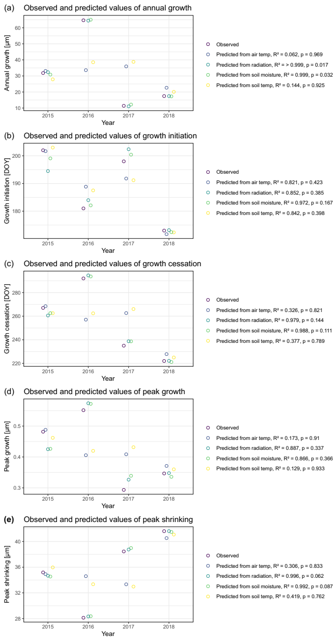
325 Figure 4: Observed and predicted values of total annual growth, defined as growth-induced, irreversible stem increment compared to the previous year, timing of growth (growth initiation and cessation), peak growth, defined as the maximum daily growth rate, and peak shrinking, defined as the maximum stem shrinking during the winter months. Predictions were obtained from the respective mean of four micro-environmental drivers and the Julian day at which their maximum occurred.
