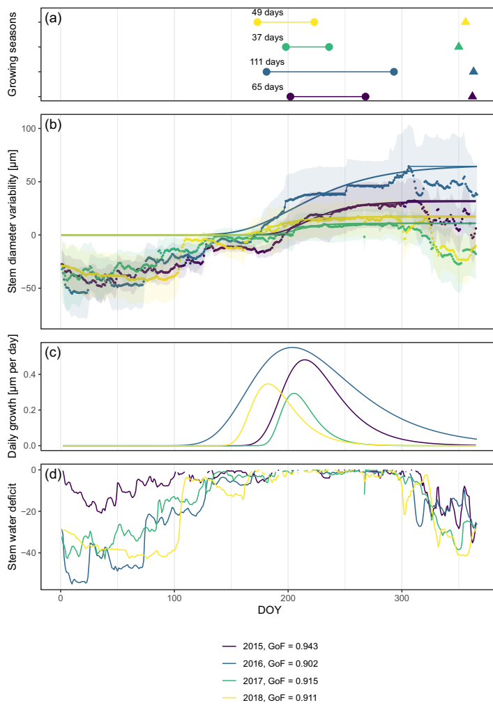
250 Figure 1: Observed and modelled variability in stem diameter. (a) Growing seasons derived from fitted Gompertz models and timing of peak shrinking defined as the maximum stem water deficit (triangles). (b) Averaged measured daily stem diameter variability and fitted Gompertz models (a goodness-of-fit (GoF) measure was calculated using the least-squares method). Models were fitted to zero growth curves derived from the original measurements as cumulative maxima (thin lines), assuming zero growth during phases of prolonged stem shrinkage. In this way, annual growth and, consequently, growth start is directly linked to growth during the previous year and additional rehydrating processes before the start of the main growing season are excluded. Shaded areas indicate standard deviation showing the variability among the specimens. (c) Daily growth rates derived from 255 Gompertz models. (d) Stem water deficit defined as reversible radial stem variability at times when no growth-induced irreversible stem expansion was measured.
