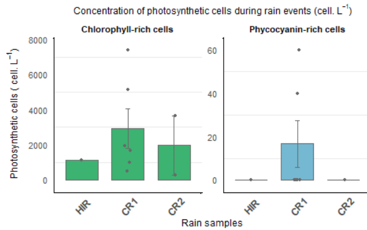
405 Fig. 5: (A) Inorganic anion and cation concentrations (mg. L -1 ) and (B) Photosynthetic cell concentrations (cell. L -1 ) in HIR, CR1 and CR2. The significance level from the Dunn test is shown to compare the nutrient concentration between rain events.
