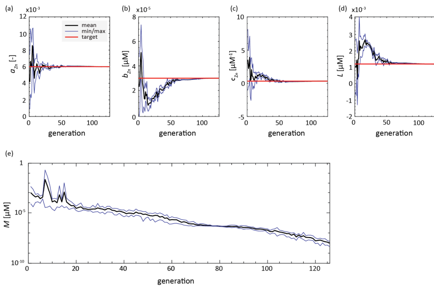
1340 Figure 3. Evolution of parameter values and misfit (RMSE) in experiment TWIN_ALL. Red lines indicate the target parameter values. Black trajectories show the mean parameter value over all individuals in each generation of ten individuals, while blue lines mark maximum and minimum parameter values in the generation.
