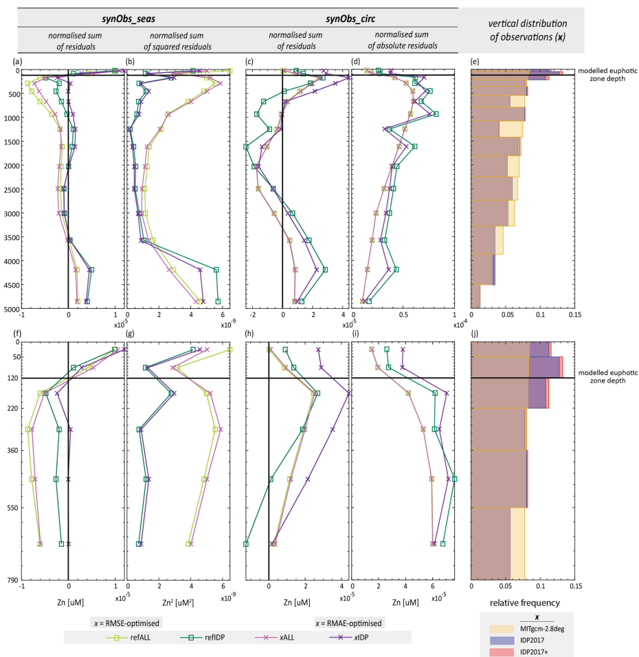
1375 Figure 10. (a, c) Integrated reference residuals (i.e. Zn_{reference} - Zn_{target} ) and residuals of optimised model over each model depth level. (f, h) are zoom-ins of (a, c). (b, g) and (d, i) are the same as (a, f) and (c, h) but the integration is done with residuals being squared and with absolute values of residuals respectively. In order to make results obtained with the two data situations comparable, all results are normalised by the total number of observations. Note that positive and negative residuals within the same depth level can cancel each other out, and that the sum is influenced by the number of model cells located in the corresponding model depth level, whereof the distribution is shown in (e, j). Panel (e) shows relative frequency distributions of the vertical distribution of three different observational sets, which are the non-reduced observations, i.e. MITgcm-2.8deg, IDP2017, and IDP2017+ and panel (j) represents a zoom-in thereof. 1380
