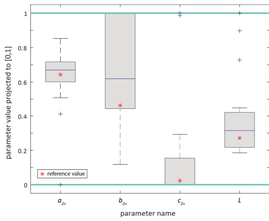
1345 Figure 4. Boxplots of optimised parameter values obtained in all synObs_experiments, presented in parameter space rescaled to the interval [0,1], i.e. turquoise lines at 0 and 1 correspond to boundary values for each parameter. Red stars indicate the reference parameter values.
