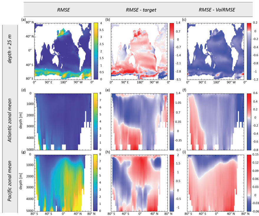
1365 Figure 8. Maps of surface Zn concentration (a-c), and zonal mean Zn concentration for the Atlantic (d-f) and the Pacific (g-i), showing the RMSE-optimised Zn field obtained in synObs_ALL_circ (first column), the difference between this field and the target field (second column), and the difference between this field and the VoIRMSE-optimised model Zn field from the same experiment (third column). Note the different colour scales in column 2 and 3. All results are interpolated to the grid of MITgcm-ECCO.
