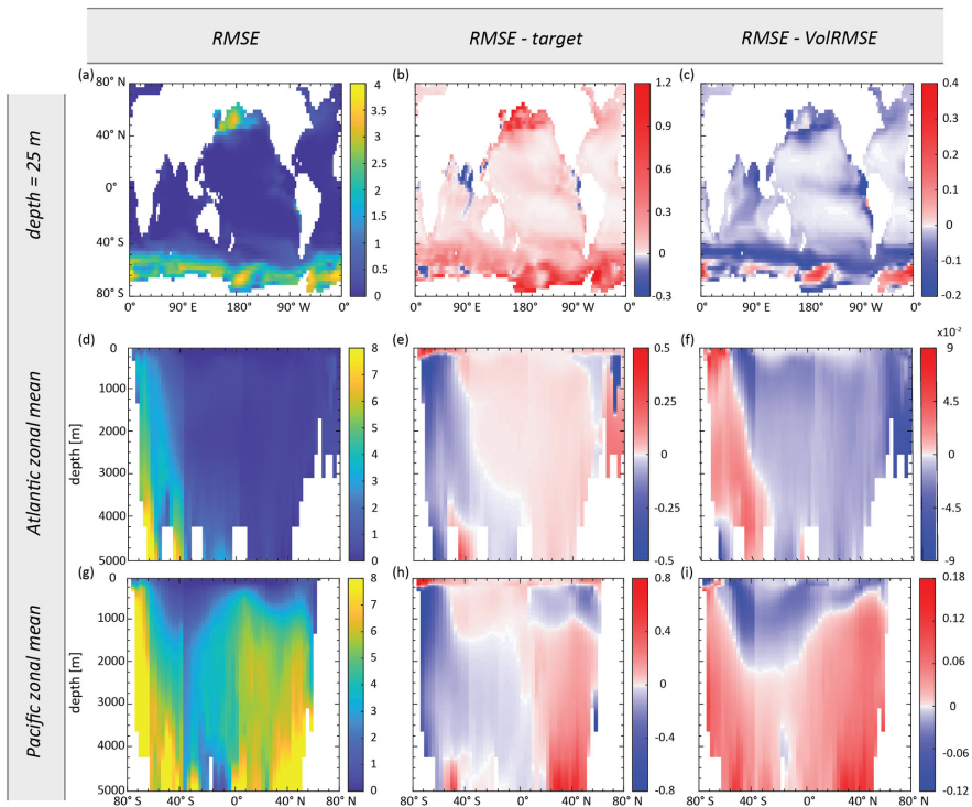
Figure 7. Maps of surface Zn concentration (a-c), and zonal mean Zn concentration for the Atlantic (d-f) and the Pacific (g-i), showing the RMSE-optimised Zn field obtained in synObs_ALL_seas (first column), the difference between this field and the target field (second column), and the difference between this field and the VoIRMSE-optimised model Zn field from the same experiment (third column). Note the different colour scales between column 2 and 3.
