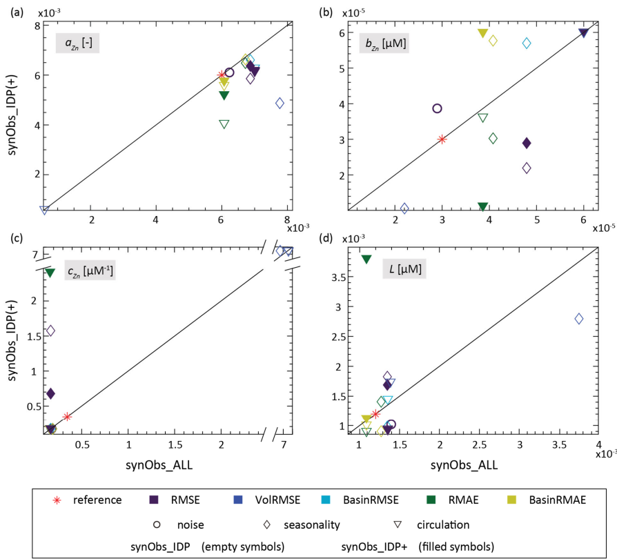
1370 Figure 9. Comparison of parameter values obtained in synObs_IDP (empty symbols) or synObs_IDP+ (filled symbols) with those from the corresponding synObs_ALL experiment. Symbols indicate the experiment type.
