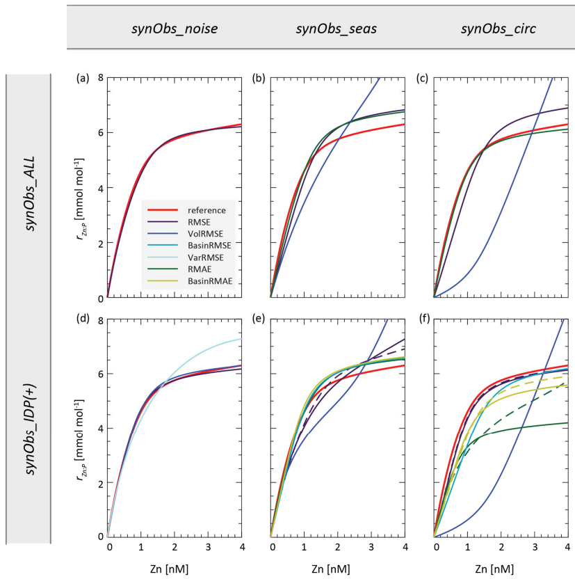
1355 Figure 6. Zn uptake systematics resulting from optimised parameter sets obtained in synObs experiments. Dashed lines in (e) and (f) are results obtained with the IDP+ data coverage (see text).
