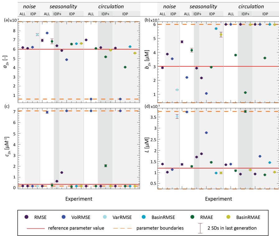
1350 Figure 5. Results from the last generation of all synObs experiments. Error bars represent 2 standard deviations calculated using the 10 individuals of the last generation. Dots represent parameter values resulting in minimum misfit within the prescribed boundaries during optimisation, coloured according to misfit metric.
