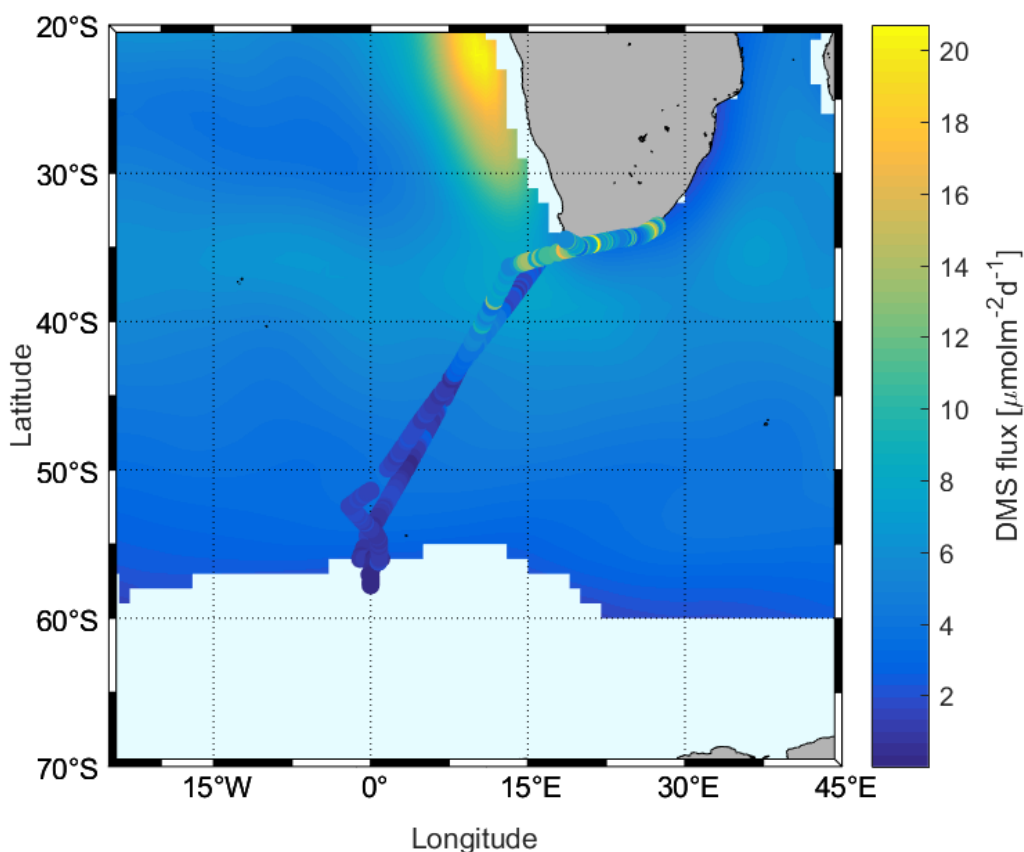
460 Figure 9: Comparison between calculated fluxes using N00 during the SCALE cruise (cruise track trace) and those in the Lana et al. (2011) climatology (background) for August.
