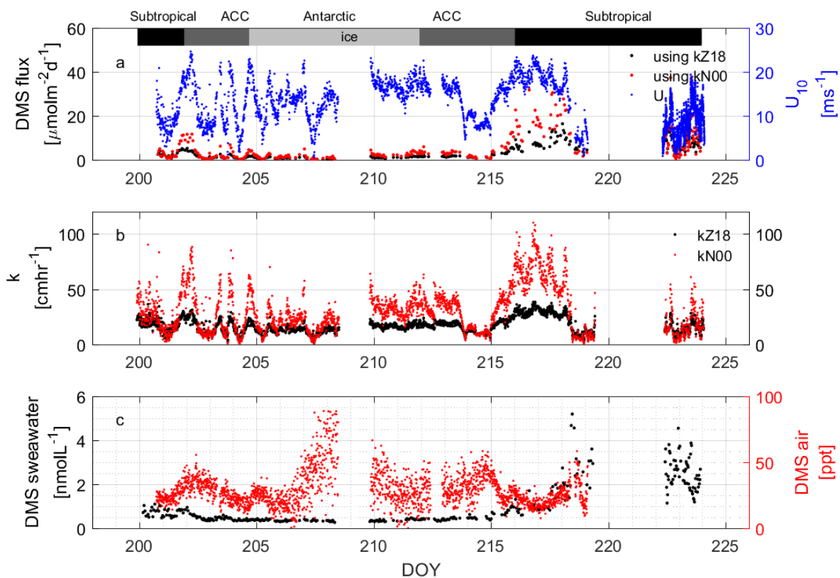
455 Figure 8: Calculated DMS fluxes (a) that depend on the indicated wind speeds ( U from 10 m) using two different k values (b). The measured water and air values that were used to compute the concentration difference are shown in c. The bars across the top of the figure denote the different hydrographic regions discussed throughout the text.
