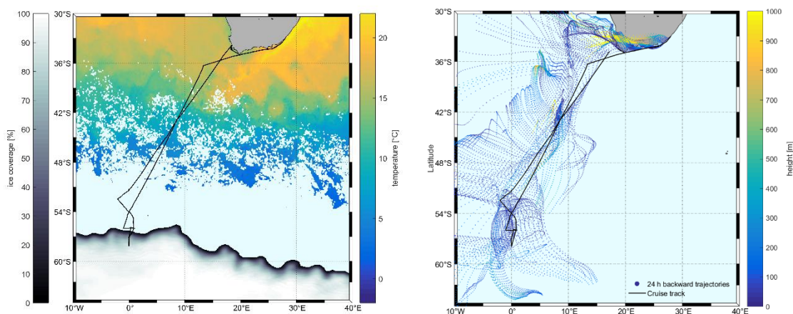
Figure 1: The cruise track (black) superimposed on satellite data. Left panel – Sea surface temperature (SST) and ice coverage (%). SST and sea ice data are derived from satellite (12 July to 12 August 2019; SST - Naval Oceanographic Office, 2008; Sea ice data - UK Met Office, 2012.). Right panel – 24h air mass back trajectories starting at 50 m height from HYbrid Single Particle Lagrangian Integrated Trajectory (HYSPLIT) using the meteorological fields from the National Centers for Environmental Prediction - Global Data Assimilation System (NCEP-GDAS). The colour shows the average height of the trajectory.
