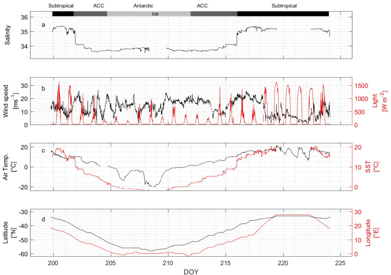
295 Figure 3: Auxiliary parameters - in situ measurements of salinity (a), wind speed at 18 m (b, black), light levels (b, red), air temperature (c, black) and SST (c, red), cruise track latitude (d, black), and cruise track longitude (d, red) averaged over 10 minutes. The bars across the top of the figure denote the different hydrographic regions discussed throughout the text.
