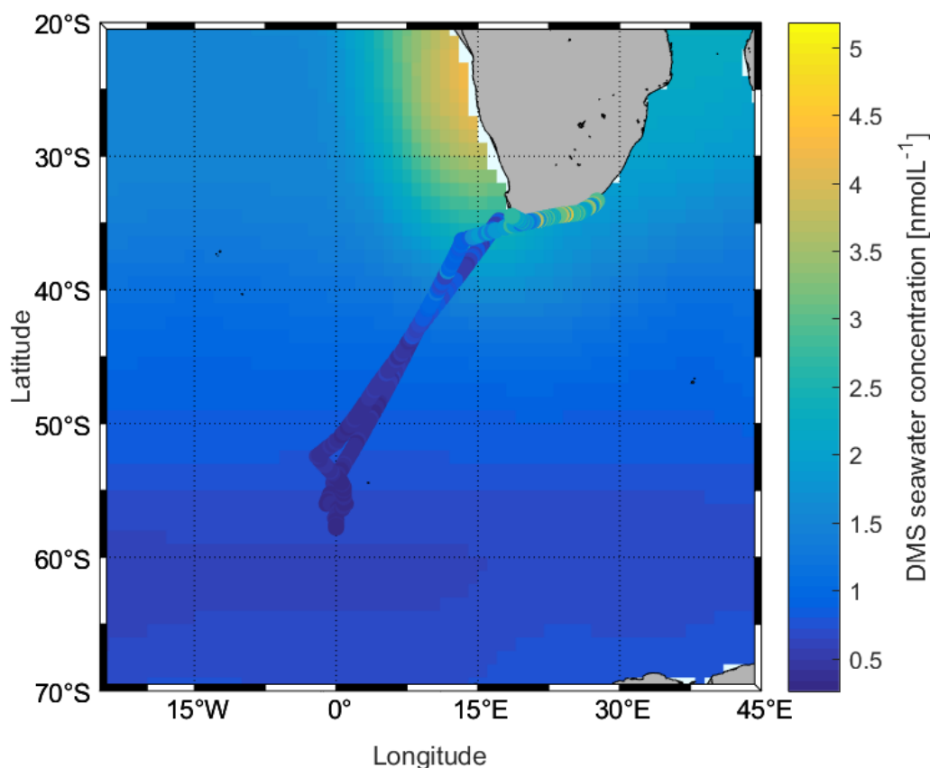
345 Figure 5: Comparison between measured DMS concentrations (cruise track trace) and those in the Lana et al. (2011) climatology (background) for August.
