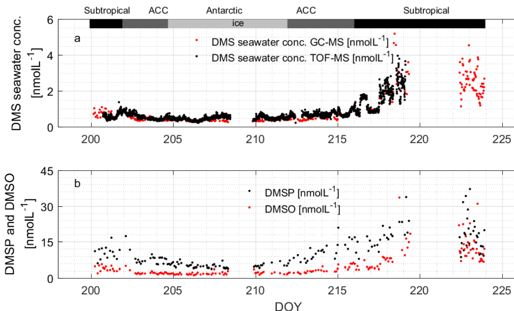
325 Figure 4: (a) Measured DMS concentrations in seawater using both instruments. (b) Measured DMSP and DMSO concentrations in the sea surface using the GC-MS. The bars across the top of the figure denote the different hydrographic regions discussed throughout the text.
