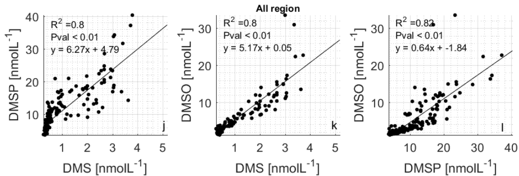
Figure 6: Correlations between measured DMSP and DMS (the left column of the figure), DMSO and DMS (the middle column of the figure) and DMSO and DMSP (the right column of the figure); a-c) subtropical region (black points); d-f) ACC region; g-i) Antarctic region; and j-l) entire cruise. The red points in a-c are data from open ocean in the subtropical area and the blue points are data from the subtropical area near the coast. The results of the correlation analysis between DMS and DMSP are: R^2=0.81 , Pval < 0.01 , y = 8.14x + 5.01 for open ocean waters; R^2=0.38 , Pval < 0.01 , y = 7.13x + 1.9 for coastal waters. The results of the correlation analysis between DMS and DMSO are: R^2=0.77 , Pval < 0.01 , y = 3.61x + 1.12 for open ocean waters; R^2=0.61 , Pval < 0.01 , y = 6.02x + -2.04 for coastal waters. The results of the correlation analysis between DMSP and DMSO are: R^2=0.76 , Pval < 0.01 , y = 0.37x + -0.11 for open ocean waters; R^2=0.5 , Pval < 0.01 , y = 0.49x + 3.26 for coastal waters.
