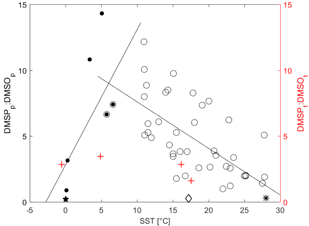
400 Figure 7: Average DMSPt:DMSOt vs SST (red) and average DMSPp:DMSOp vs SST (black). Mean ratios for individual campaigns are recalculated from the data listed in Simó and Vila-Costa (2006). We added data points consisting of the mean DMSPp:DMSOp and SST (given in parenthesis) from the East China Sea (0.27, 17.2 °C, open diamond) (Yang and Yang, 2011), the northern Baffin Bay (0.20, estimated 0 °C; closed pentagram) (Bouillon et al., 2002) and the western Pacific Ocean (0.22, 28 °C, open asterisk) (Zindler et al., 2013). The linear correlations are y = -0.35x + 11.13 ( R^2 = 0.45 , open 405 circles) and y = 1.03x + 2.82 ( R^2 = 0.57 , solid circles). Our Southern Ocean, ACC, and subtropical open ocean and coastal areas are the red plus signs.
