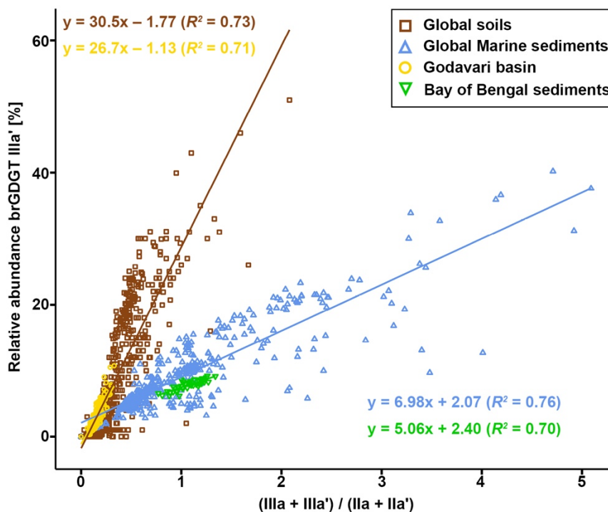
Figure 9 – Crossplot of the ratio (IIIa + IIIa') / (IIa + IIa') versus the relative abundance of IIIa' for globally distributed soils (square) and marine sediments (triangle) after Xiao et al. (2020) and Godavari basin samples, including soils, SPM and riverbed sediments collected the dry and wet seasons (circle) and the Bay of Bengal Holocene sediments (inverted triangle). The solid lines denote the linear fit, and the correlations and R 2 are shown.
