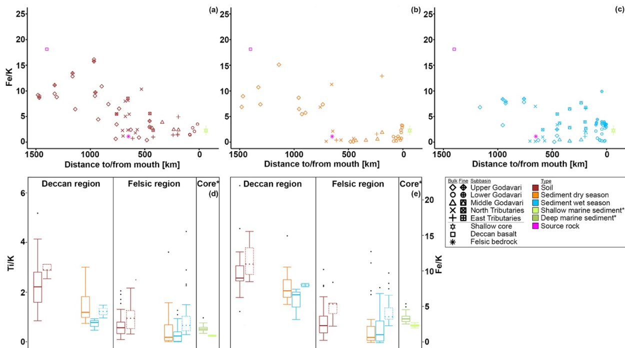
Figure A2. Fe/K ratios in (a) soils and riverbed sediments collected in the (b) dry and (c) wet season versus distance to/from the river mouth. The square and star (magenta) represent the end-member values for the Deccan basalts (Das and Krishnaswami, 2007) and felsic bedrocks (Archean Proterozoic Gneiss Complexes, APGC) (Moyen et al., 2003), respectively. The outlined star (greenyellow) represents the average of marine sediments retrieved from shallow cores in front of the Godavari mouth (0-48 cm below sea floor, ~300 yr.; Kalesha et al., 1980) (error bar represents the standard deviation: \pm 0.83 ). Box-and-whisker plots of (d) Ti/K and (e) Fe/K ratios for the Godavari basin soils and sediments collected in the Deccan basalts and felsic regions and in marine sediments in the Bay of Bengal. * Core data are retrieved from shallow (0-48 cm below sea floor, ~300 yr.; Kalesha et al., 1980) and deep marine sediments (0-300 m (NGHP-1-3B) and 0-184 m bsf (NGHP-1-5C), no age model used; Mazumdar et al., 2015). The box represents the first (Q1) and third (Q3) quartiles, and the line in the box represents the median value, the whiskers extent to 1.5 \times (Q3 - Q1) values and outliers are shown as points. Solid lines represent bulk data, dashed lines the fine fractions ( \leq 63 \mu\text{m} ). 905 910
