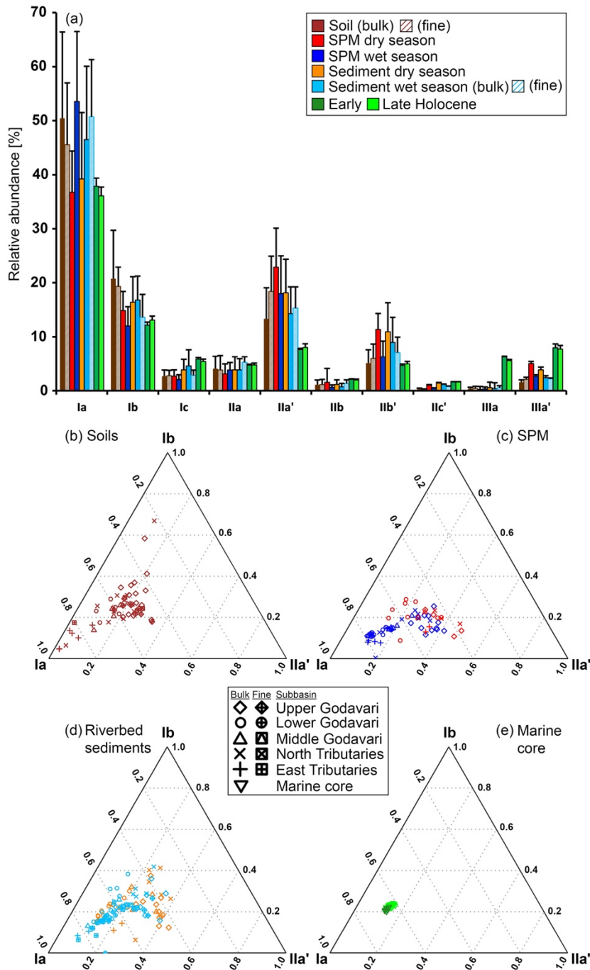
480 Figure 4 – BrGDGT distributions in the Godavari basin and in marine sediments from the Bay of Bengal. (a) Average relative abundances of brGDGTs in soils, SPM and riverbed sediments in the dry and wet season, and in Holocene marine sediments. The error bars represent the standard deviation. The fine fraction soils and sediments ( \leq 63 \mu\text{m} ) are striped. Proportions of major brGDGTs Ia, IIa' and Ib in (b) soils, (c) SPM, (d) riverbed sediments and in a (e) Holocene marine core. The symbols represent the different subbasins, with open symbols for the bulk soils and sediments and enclosed symbols for the fine fractions.
