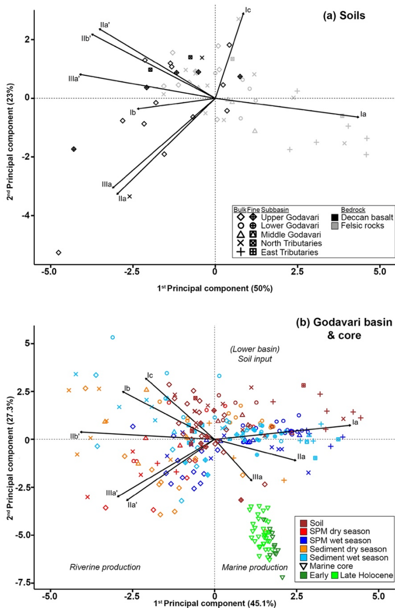
Figure 6 – Principal Component Analysis (PCA) of the eight major brGDGTs (i.e., Ia, Ib, Ic, IIa, IIa', IIb', IIIa and IIIa'). (a) PCA for soils formed on Deccan basalts (black) and felsic bedrocks (grey) (PC1 versus PC2). (b) PCA for SPM and bulk riverbed sediments collected in the wet and dry season (PC1 versus PC2), to which PCA scores of the bulk soils and Holocene riverbed sediments are added passively. The latter implies that the PCA calculation and biplot configuration is based on brGDGT distributions in river SPM and sediments (i.e., ‘active’ samples), to which the scores of soils and marine sediments (i.e., ‘passive’ samples) are added as an overlay. The vectors indicate the PCA scores of the individual brGDGTs. The symbols refer to the different subbasins and the different fractions (bulk and fine fractions \leq 63 \mu\text{m} ) (see legend a). The colours refer to the different sample types.
