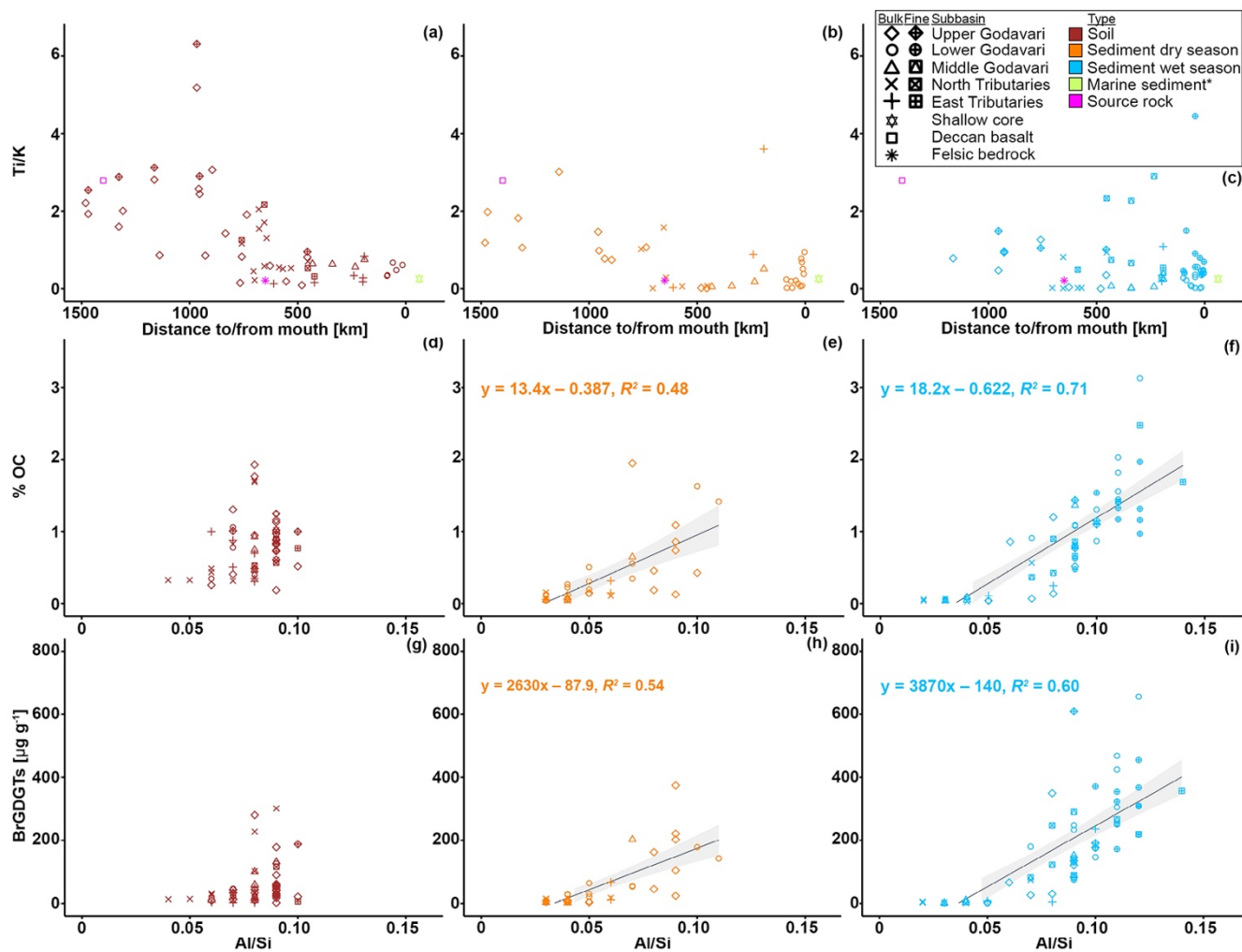
660 Figure 8 – Ti/K ratios in (a) soils and riverbed sediments collected in the (b) dry and (c) wet season versus distance to/from the river mouth. The square and star (magenta) represent the end-member values for the Deccan basalts (Das and Krishnaswami, 2007) and felsic bedrocks (Archean Proterozoic Gneiss Complexes, APGC) (Moyen et al., 2003), respectively. The outlined star (greenyellow) represents the average of marine sediments retrieved from * shallow cores in front of the Godavari mouth (0–48 cm below sea floor, ~300 yr.; Kalesha et al., 1980) (error bars representing the standard deviation ( \pm 0.02 ) are not visible as they are smaller than the symbol). %OC and brGDGT concentrations versus Al/Si ratios in soils (d, g) and riverbed sediments collected in the (e, h) dry and (f, i) wet season, respectively. Low Al/Si ratios indicate a bulk mineralogical composition with high proportions of quartz (coarse grained) and high ratios indicate high proportions of micas and clays (fine grained) (Galy et al., 2008, 2010). Linear correlations (solid line) and 95% confidence intervals (grey shading) are shown. The symbols refer to the different subbasins, and the different fractions (bulk and fine fractions \leq 63 \mu\text{m} ). The colours refer to the different sample types. 665
