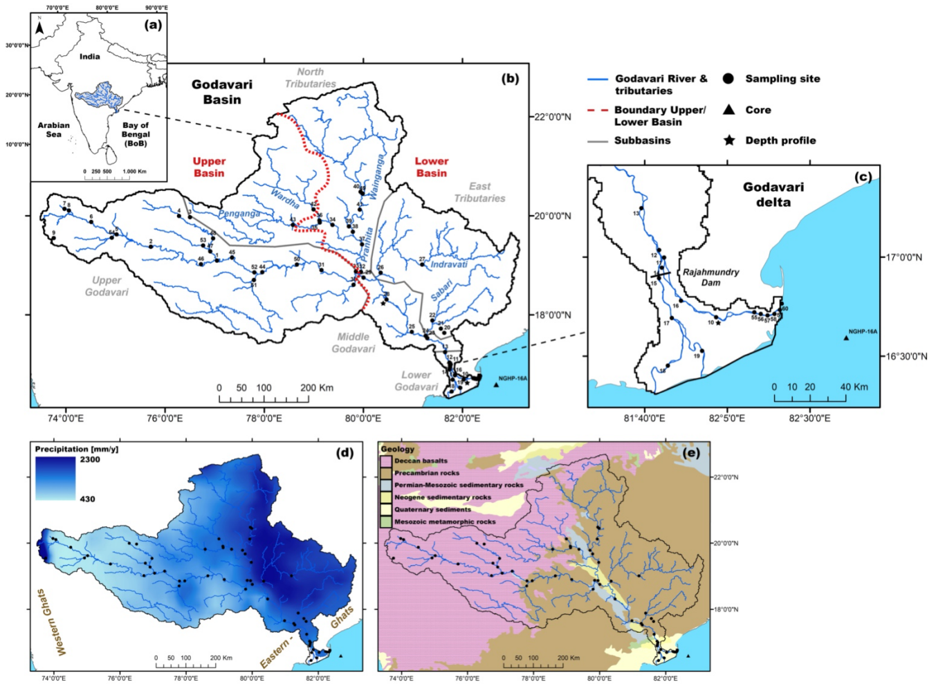
145 Figure 1 – (a) Location of the Godavari River basin in peninsular India, (b) Sampling sites along the river basin, with the different subbasins (grey) and upper and lower basin (red) shown. (c) Zoom for the Godavari delta and the Reservoir Dam at Rajahmundry. (d) Precipitation across the Godavari basin based on the APHRODITE data set (Asian Precipitation – Highly Resolved Observational Data Integration Towards Evaluation of Water Resources, V1101 Monsoon Asia) of mean annual precipitation for 30 years at a 0.25° grid resolution (Yatagai et al., 2009). (e) Geological context of the Godavari basin.
