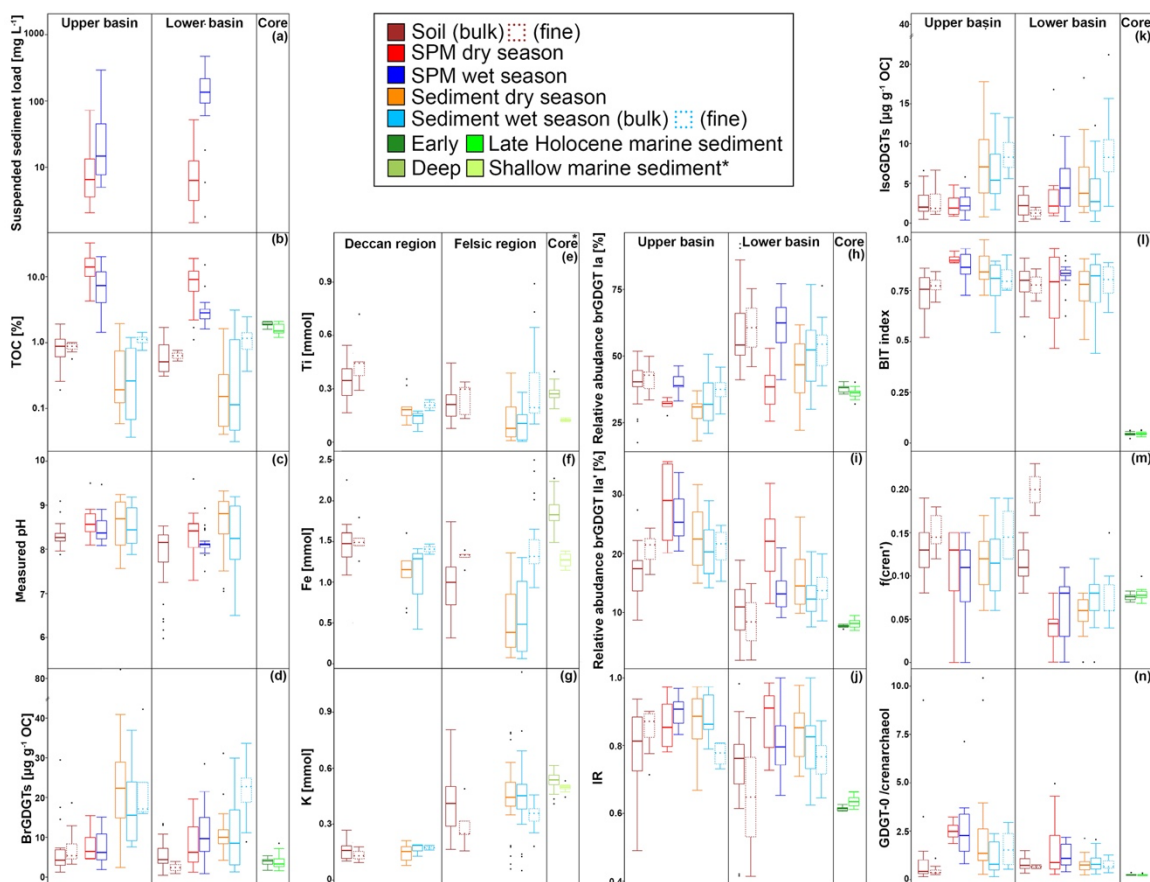
350 Figure 2 – Box-and-whisker plots of the organic, geochemical and GDGT data for the Godavari basin and marine sediments in the Bay of Bengal. (a) Suspended sediment load, (b) Total Organic Carbon (TOC), (c) measured pH, and (d) brGDGT concentrations normalised to %OC in the upper and lower basin and in Holocene marine sediments. (e) Ti, (f) Fe and (g) K amounts in the Deccan basalt and felsic bedrock regions, and * in shallow (0–48 cm below sea floor, ~300 yr.; Kalesha et al., 1980) and deep marine sediments (0–300 m (NGHP-1-3B) and 0–184 m bsf (NGHP-1-5C), no age model used; Mazumdar et al., 2015). (h) Relative abundance of brGDGT Ia, (i) Relative abundance of brGDGT Ila' and (j) Isomer Ratio (IR) values in the upper and lower basin and in Holocene marine sediments. (k) IsoGDGT concentrations normalised to %OC, (l) BIT index, (m) f(cren') and (n) GDGT-0/crenarchaeol in the upper and lower basin and in Holocene marine sediments. The box represents the first (Q1) and third (Q3) quartiles, and the line in the box represents the median value, the whiskers extent to 1.5×(Q3–Q1) values and outliers are shown as points. Solid lines represent bulk data, dashed lines the fine fractions (≤63 μm). The pH represents values measured in soil and sediment extracts and in surface water for SPM. 355 360
