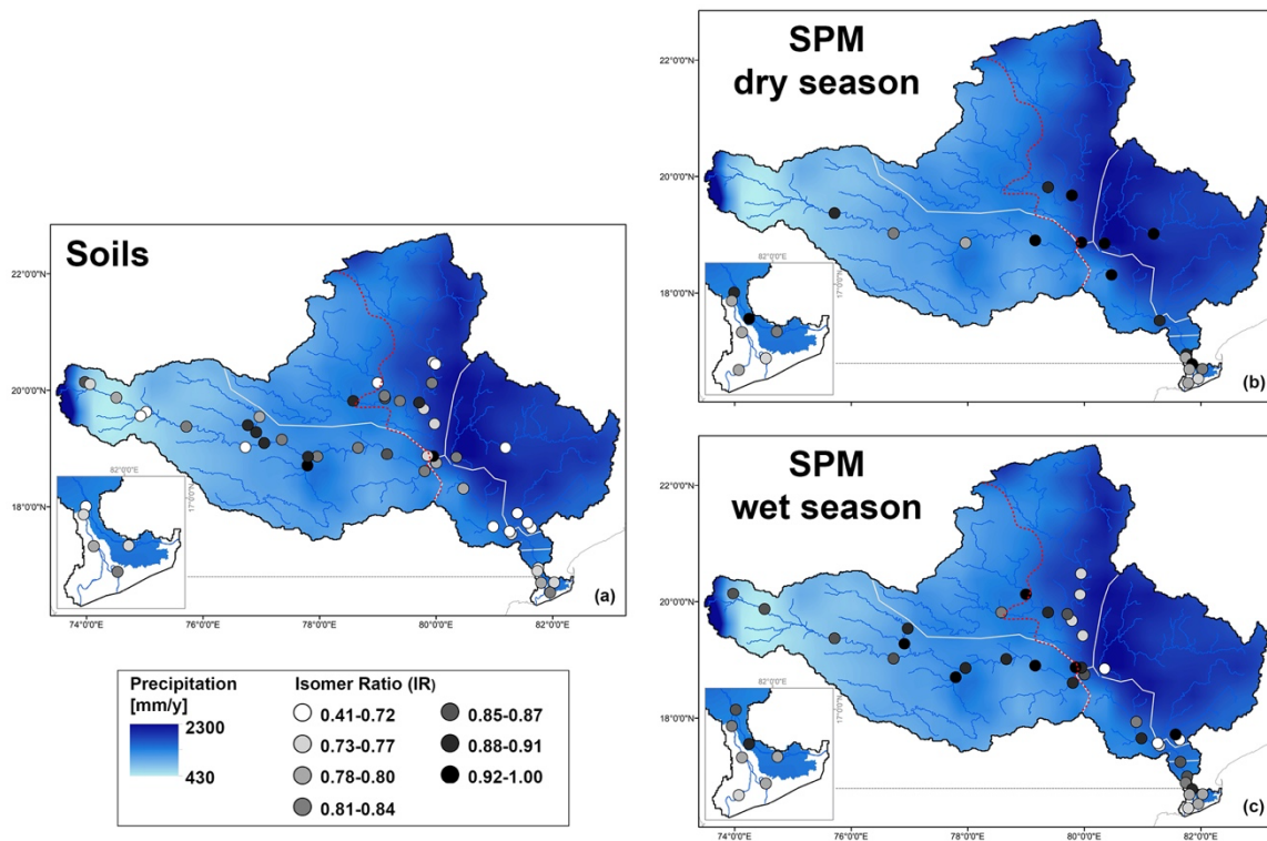
620 Figure 7 – Maps showing the spatial distribution of IR values for (a) soils and SPM collected in the (b) dry and (c) wet season. The main panel shows the whole basin, with a zoom for the delta region. The points refer to the IR values and the long-term average rainfall distribution is shown on the background.
