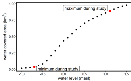
Figure 2. Hypsographic curve of the study area, in increments of 0.1 m. The red dots represent the observed range of the water level during the study. For a water level time series during the sampling period, see Figure A1.
