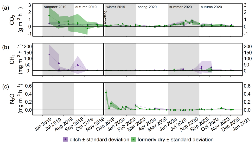
Figure 8. Time series of the mean (a) CO 2 , (b) CH 4 , and (c) N 2 O fluxes (± standard deviations) from June 2019 to December 2020. Fluxes of the permanently wet drainage ditch are shown in purple and those derived from the two methods employed in this study in green. The vertical black line indicates the rewetting event.
