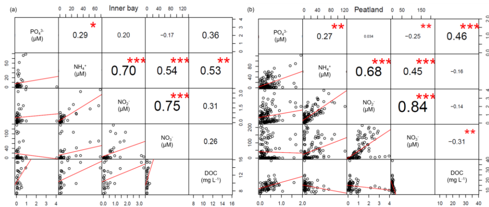
Figure D1. Cross plots of the measured nutrient (NH 4 + , NO 3 - , NO 2 - , PO 4 3- ) and DOC concentrations in (a) the inner bay and (b) the peatland across all seasons. Significant correlations are indicated by asterisks.
