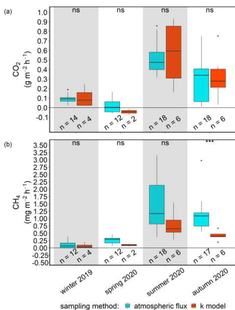
Figure C1. Seasonal post-rewetting fluxes of (a) CO 2 and (b) CH 4 at station BTD7 which is part of the GHG flux transect. Chamber-based atmospheric GHG fluxes are shown in blue and air-sea GHG fluxes from the k model in red. The methodological comparisons within seasons are based on a significance level of p < 0.05 . ns: not significant; *** p < 0.001 .
