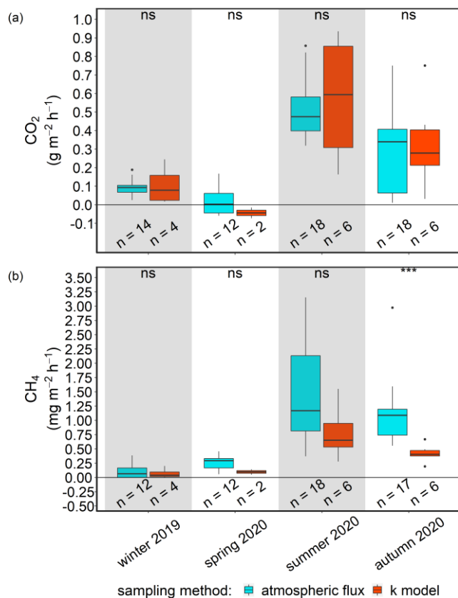
Figure C1. Seasonal post-rewetting fluxes of (a) CO 2 and (b) CH 4 at station BTD7 which is part of the GHG flux transect. Chamber-based atmospheric GHG fluxes are shown in blue and air-sea GHG fluxes from the k model in red. The methodological comparisons within seasons are based on a significance level of p < 0.05 . ns: not significant; *** p < 0.001 .
