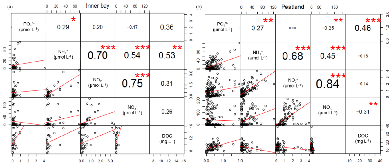
865 Figure D1. Cross plots of the measured nutrient (NH 4 + , NO 3 - , NO 2 - , PO 4 3- ) and DOC concentrations in (a) the inner bay and (b) the peatland across all seasons. Significant correlations are indicated by asterisks.
