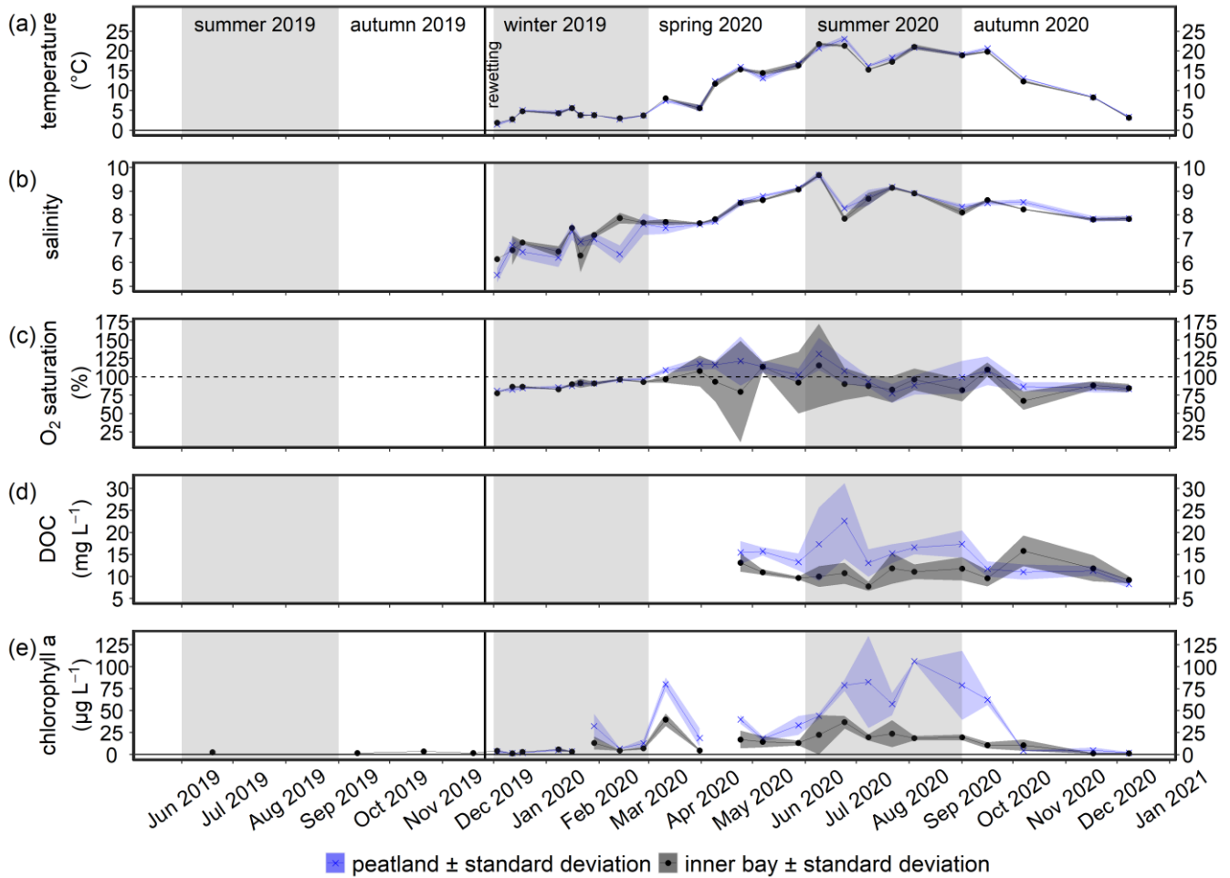
Figure 4. Time series of the mean (a) temperature, (b) salinity, (c) O 2 saturation, (d) DOC concentration and (e) chlorophyll a concentration ( \pm standard deviations) in the surface water from June 2019 to December 2020. Data from the flooded peatland ( n = 6 ) are shown in blue and data from the inner bay ( n = 2 or 3, as explained in Sect. 2.3) in black. The vertical black line indicates the rewetting event.
