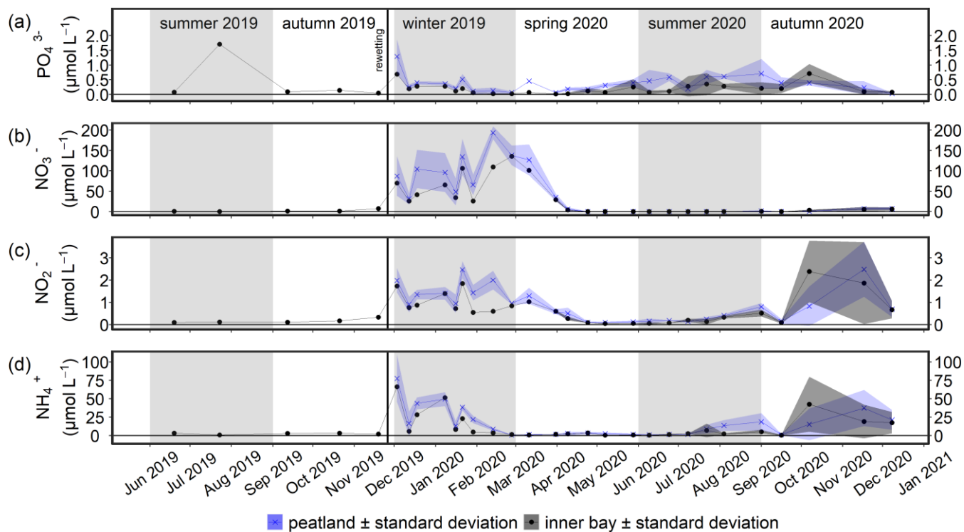
420 Figure 5. Time series of the mean (a) \text{PO}_4^{3-} , (b) \text{NO}_3^- , (c) \text{NO}_2^- , and (d) \text{NH}_4^+ concentrations ( \pm standard deviations) in the surface water from June 2019 to December 2020. Data from the flooded peatland ( n = 6 ) are shown in blue and data from the inner bay (until 11 March 2020: n = 1 , thereafter: n = 2 ) in black. The vertical black line indicates the rewetting event.
