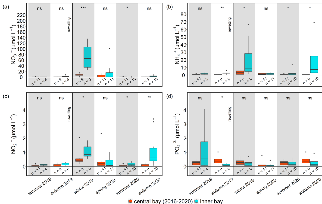
425 Figure 6. Seasonal nutrient concentrations of (a) \text{NO}_3^- , (b) \text{NH}_4^+ , (c) \text{NO}_2^- , and (d) \text{PO}_4^{3-} at the nearby monitoring station (central bay, red) and in the inner bay (inner bay, blue) from pre- to post-rewetting. The vertical black line indicates the rewetting event. Note that 5-year-data (2016–2020) are shown for the central bay (see Sect. 2.4.2). ns = not significant, * = p < 0.05 , ** = p < 0.01 , *** = p < 0.001 .
