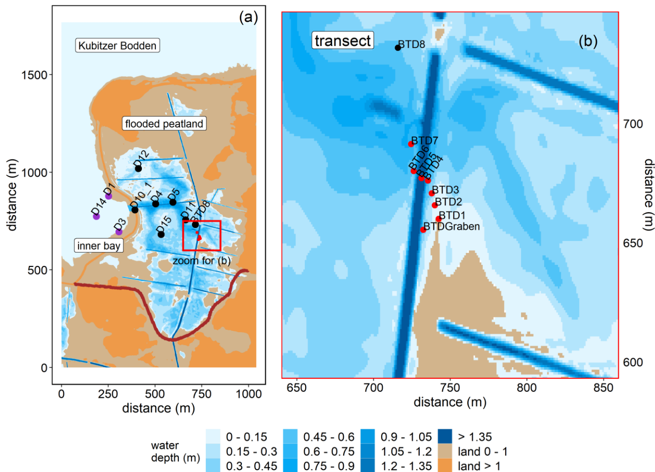
Figure 2. Topography of the study area and overview of the stations in the inner bay (purple), the flooded peatland (black) and along the transect of the GHG flux measurements (red). (a) Water coverage at mean sea level. The new dike is shown in dark red. (b) Transect stations that were sampled for atmospheric chamber-based GHG flux measurements (before and after rewetting) and for surface water GHG concentration measurements (after rewetting). Data from station BTD7 were used for a comparison of the chamber-based measurements with the calculated air-sea fluxes after rewetting. Topography data retrieved from AfGVK, LAiV MV.
