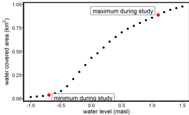
Figure 3. Hypsographic curve of the study area, in increments of 0.1 m. The red dots represent the observed range of the water level during the study. For a water level time series during the sampling period, see Figure A1.
