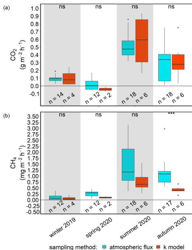
855 Figure C1. Seasonal post-rewetting fluxes of (a) CO 2 and (b) CH 4 at station BT7 which is part of the GHG flux transect. Chamber-based atmospheric GHG fluxes are shown in blue and air-sea GHG fluxes from the k model in red. The methodological comparisons within seasons are based on a significance level of p < 0.05 . ns: not significant; *** p < 0.001 .
