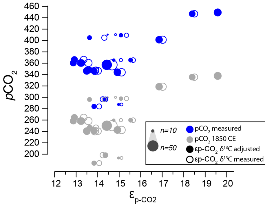
Figure 3. Effects of \delta^{13}\text{C} and p\text{CO}_2 corrections (see also Figure 2 and §3.2).
