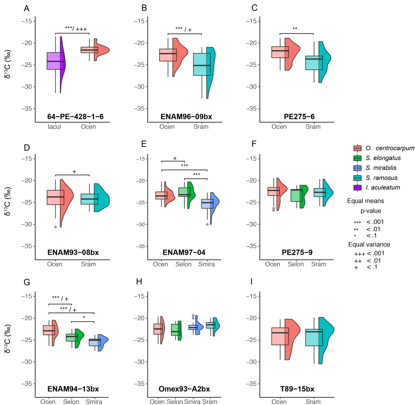
Figure 4. Carbon isotope measurements for multiple species; each panel represents a single sample after eliminating extremely small measurements sizes (<0.2 Vs), background correction and removing outliers ( \pm 2.5 interquartile range) (paragraph §3.2).
