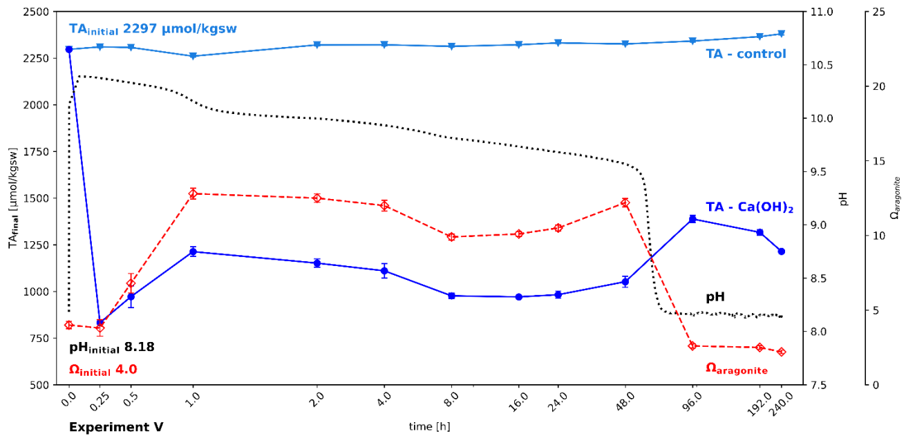
Figure 7: Partial recovery of alkalinity after carbonate precipitation; Change in alkalinity, pH and \Omega_{\text{aragonite}} after adding 0.66 g \text{Ca}(\text{OH})_2 / kgw/kgsw to North Sea water in a shaking bath (simulating wave processes to allow accelerated air-water- \text{CO}_2 -exchange). \text{Ca}(\text{OH})_2 dissolution is so fast, that it is hard to track. While the water gradually equilibrates with the atmosphere, a series of loss and gain of alkalinity can be observed.
