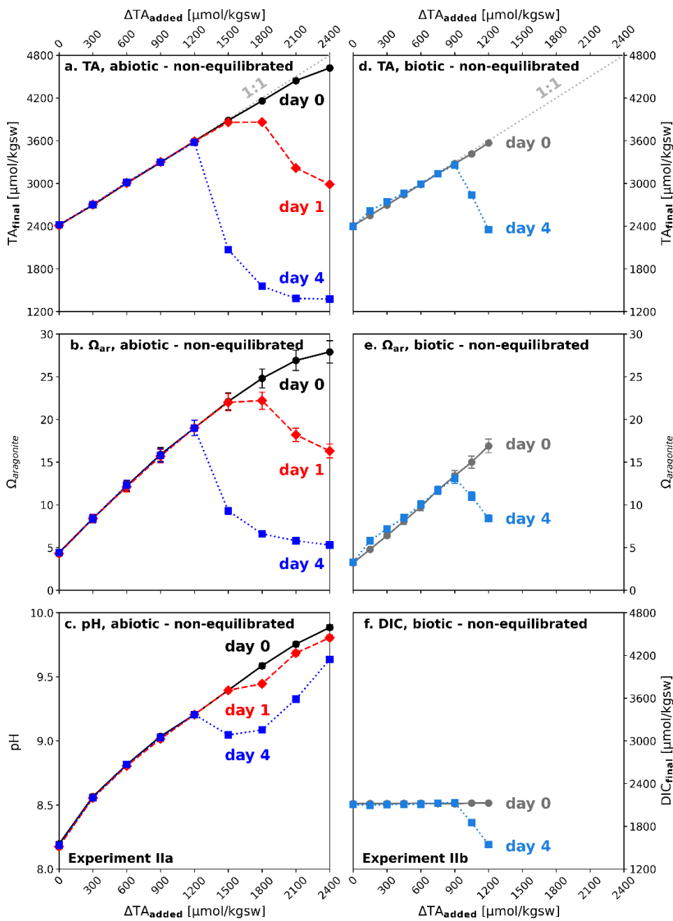
Figure 2: Temporal development after non-equilibrated alkalinisation: (a, b, c) experiment IIa, (d, e, f) experiment IIb; (a, d) \Delta TA_{added} vs. TA_{final} ; (b, e) aragonite saturation state ( \Omega_{aragonite} ) in relation to \Delta TA_{added} ; (c) pH in relation to \Delta TA_{added} ; (f) DIC_{final} in relation to \Delta TA_{added} . Black/grey symbols correspond to start of the experiment, red after 1 day and blue after 4 days. Note the different ranges of \Delta TA_{added} in the abiotic and biotic set-up. The slightly higher start \Omega_{aragonite} for the biotic treatment at day 4 compared to day 1 is because \Omega_{aragonite} was calculated by TA and DIC, while for the abiotic experiment using TA and pH.
