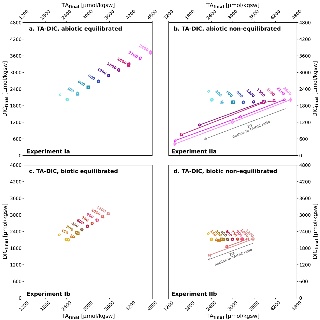
Figure 3: TA final versus DIC final at the start of the experiments I and II and after precipitation; (a-b) abiotic after 0, 1 and 4 days, (c-d) biotic after 0 and 4 days, equilibrated alkalinisation (left, experiment I), non-equilibrated alkalinisation (right, experiment II). The TA:DIC change ratio of 2:1 indicates that alkalinity loss was due to carbonate precipitation. Sampling days (0, 1 and 4) are written on top of each datapoint marker. Due to overlapping in case of no change in data, the marker description is set up to down. The grey arrows in b. and d. indicate an ideal 2:1 decline in TA:DIC.
