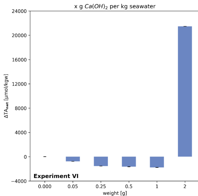
Figure 8: Change in alkalinity after adding \text{Mg}(\text{OH})_2 or \text{Ca}(\text{OH})_2 to North Sea water in a shaking bath (simulating wave processes to allow accelerated air-water- \text{CO}_2 -exchange). (a) Net loss occurs when alkalinity addition exceeds the critical saturation level of aragonite, while in (b) it is shown, using \text{Ca}(\text{OH})_2 that for high added amounts of solid the \Delta TA_{net} -loss can be turned into a gain. Note for data in 8b no pH values are available for calculation of aragonite saturation levels.
