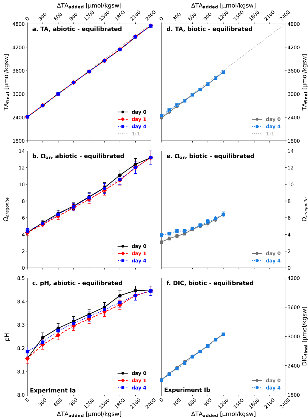
220 Figure 1: Temporal development after CO 2 equilibrated alkalisation: (a, b, c) experiment Ia, (d, e, f) experiment Ib; (a, d) \Delta TA_{\text{added}} vs. TA_{\text{final}} ; (b, e) aragonite saturation state ( \Omega_{\text{aragonite}} ) in relation to \Delta TA_{\text{added}} ; (c) pH in relation to \Delta TA_{\text{added}} ; (f) DIC_{\text{final}} in relation to \Delta TA_{\text{added}} . Black/grey symbols correspond to start of the experiment, red after 1 day and blue after 4 days. TA_{\text{initial}} conditions of used seawater: \Delta TA_0 \approx 2,411 \mu\text{mol/kgsw} , \Omega_{\text{Ar}} = 3.542 , pH = 8.0715.
