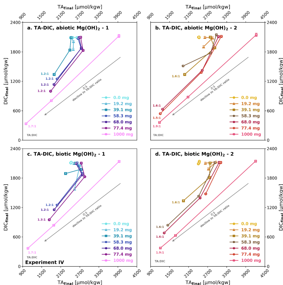
Figure 6: Development of TA_{final} versus DIC_{final} during brucite dissolution in experiment IV; (a, b) abiotic after 0, 1 and 4 days, (c, d) biotic after 0 and 4 days. The days of sampling (0, 1 and 4) are written on top of each data point marker. TA:DIC change ratios for brucite I (1.2:1) and brucite II (1.6:1) are indicating simultaneous precipitation and dissolution, while their difference could be described by their differing dissolution characteristics. The grey arrows indicate an ideal 2:1 decline in TA:DIC.
