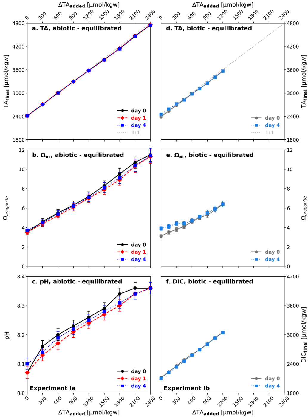
Figure 1: Temporal development after CO 2 equilibrated alkalinisation: (a, b, c) experiment Ia, (d, e, f) experiment Ib; (a, d) \Delta TA_{added} vs. TA_{final} ; (b, e) aragonite saturation state ( \Omega_{aragonite} ) in relation to \Delta TA_{added} ; (c) pH in relation to \Delta TA_{added} ; (f) DIC_{final} in relation to \Delta TA_{added} . Black/grey symbols correspond to start of the experiment, red after 1 day and blue after 4 days. TA_{initial} conditions of used seawater: \Delta TA_0 \approx 2,411 \mu\text{mol/kgw} , \Omega_{Ar} = 3.5 , pH = 8.07 .
